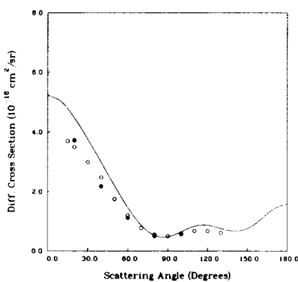
Figure 2. Differential cross section for elastic electron-CF 4 scattering at 8 eV. Solid line, present polarized result, filled circles, experiment of Mann and Linder, 46 and open circles, experiment of Boesten et al. 47
