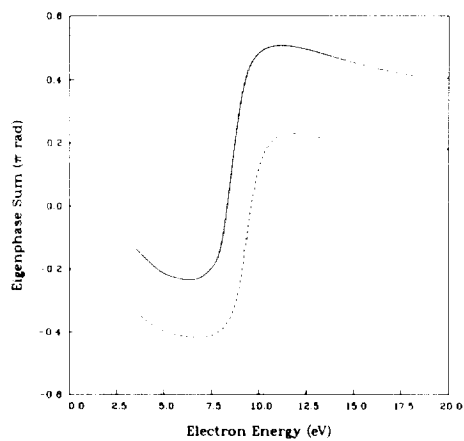
Figure 1. Eigenphase sums for electron-CF 4 scattering, showing resonances in the 2 A 1 (dashed line) and 2 T 2z (solid line) partial channels.
