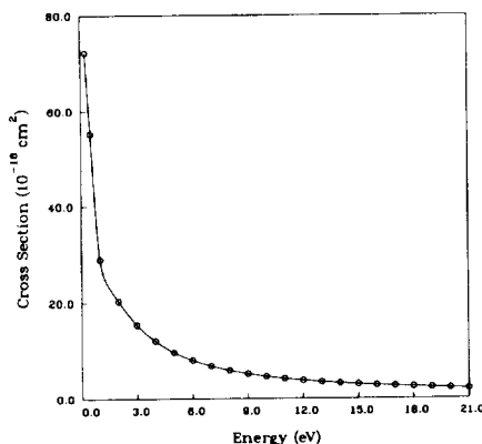
Figure 10. Integral cross section for e-H 2 ^2\Sigma_g^+ channel elastic scattering in the static-exchange approximation, calculated using a two-term CI function for the target
