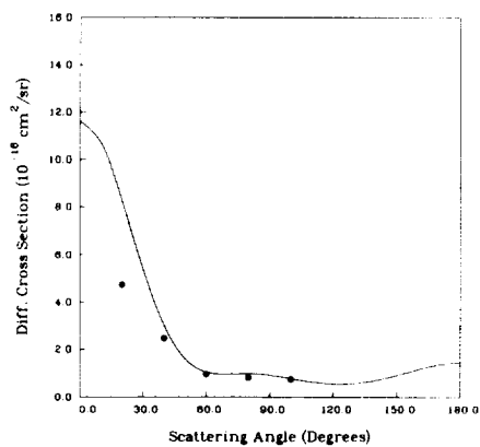
Figure 3. Differential cross section for elastic electron-CF 4 scattering at 11 eV. Solid line, present polarized result, and filled circles, experiment of Mann and Linder. 46
