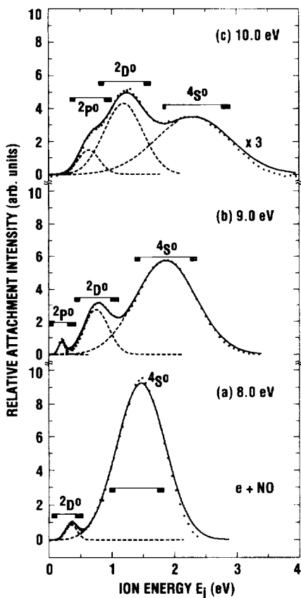
FIG. 2. Energy spectra of the channels O^-(^2P) + N(^2P^0, ^2D^0, ^4S^0) in DA to NO at the indicated electron energies of (a) 8 eV, (b) 9 eV, and (c) 10 eV. Dashed lines are results of unfolding; the solid line is the calculated sum intensity to be compared with data ( \bullet ). Lines above each feature represent the range of ion energies for the range \theta(0, \pi) , including contribution from a \pm 0.2 eV electron beam width [shaded areas, Eq. (5)].
