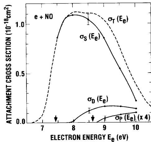
FIG. 4. Electron attachment cross sections \sigma_S(E_e) , \sigma_P(E_e) , and \sigma_D(E_e) for the individual S, P, D channels normalized to the total cross sections \sigma_T(E_e) of Ref. [8].
