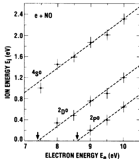
FIG. 3. Unfolded peak intensities of the channels O^-(^2P) + N(^2P^0, ^2D^0, ^4S^0) in DA to NO as a function of attaching electron energy E_e . Straight lines are drawn with the theoretical kinematic slope of \mu/m_0 = 14/30 . Threshold energies are 8.611 eV ( ^2P^0 ), 7.419 eV ( ^2D^0 ), and 5.035 eV ( ^4S^0 , not indicated).
