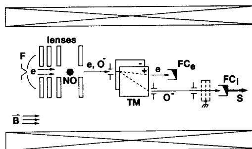
FIG. 1. Schematic diagram (not to scale) of the magnetically confined trochoidal system. Electrons ( e ) from a filament ( F ) attach in the energy range 7.5–10.0 eV to a beam of NO to form O^-(^2P) ions. The ions and parent electrons are separated by the trochoidal monochromator (TM), and the resulting energy-analyzed ion signal S is detected at FC_i in an analog mode. Length of the solenoidal magnet is 1 m.
