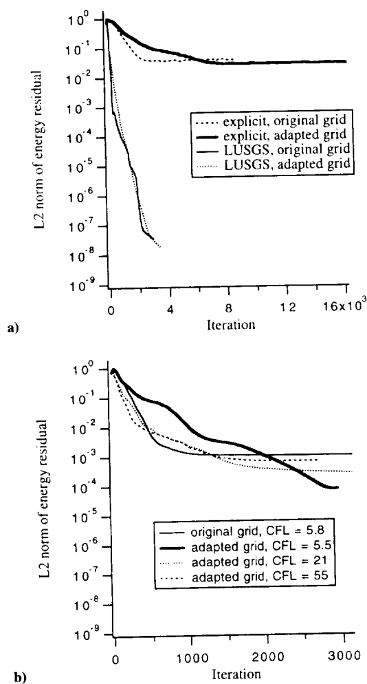
Fig. 8 Effect of grid adaption: a) grid comparison, Mach 30 and b) grid comparison, LUSGS, Mach 40.
