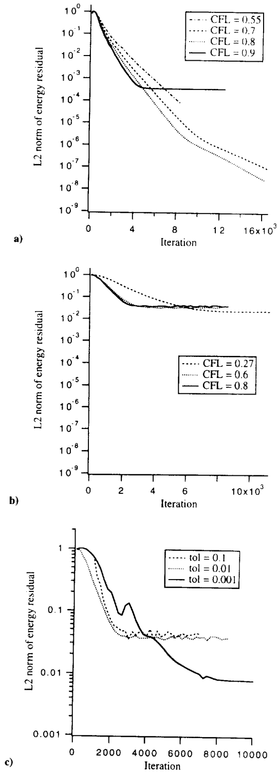
Fig. 4 Convergence histories, explicit under-relaxation method: a) Mach 15, b) Mach 30, and c) constant parametric study.
