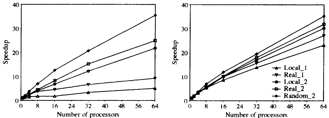
FIG. 3. Speedup of the parallel mesh adaptor during refinement (left) and coarsening (right).
