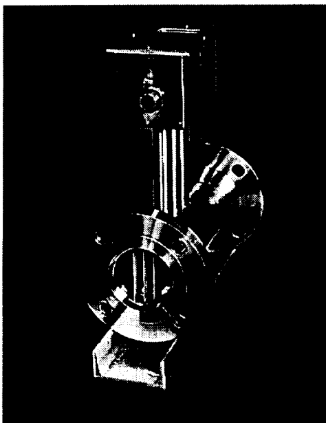
Capacitor plates in the two-phase meter enable the measurement of vapor liquid ratio.
