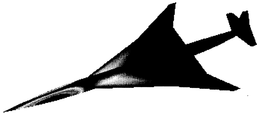
Fig. 7.6 Y-coordinate sensitivity with respect to chord.
