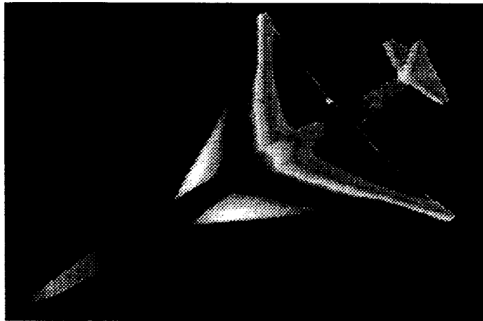
Fig. 7.9 Cp over the final HSCT configuration.
