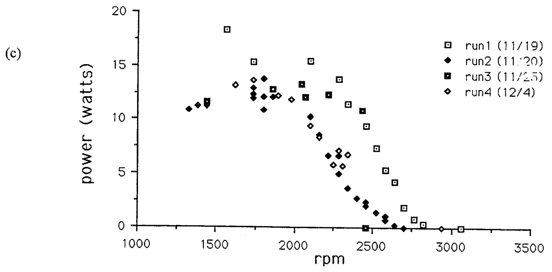
Fig. 36 Reproducibility testing of Ross engine.
