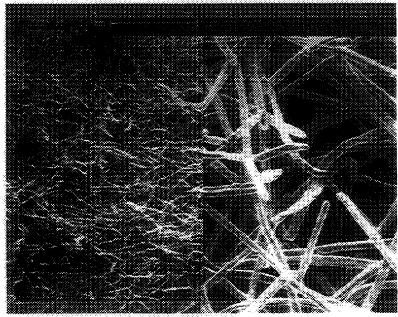
Fig. 10 SEM photos of (a) carbon and (b) steel felts.
