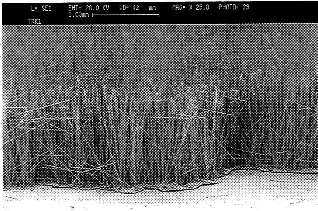
Fig. 21 Illustrative carbon fiber flocks.
