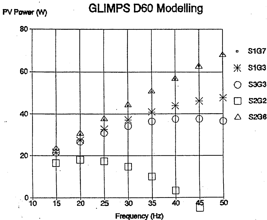
Fig. 31 GLIMPS modeling of Ross D-60 engine.
