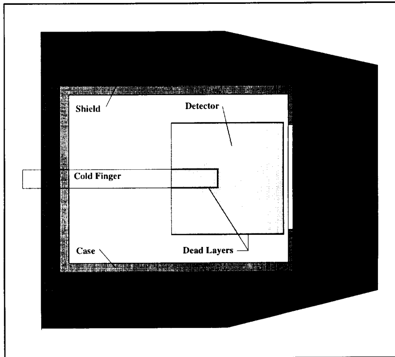
Figure 1: A sample detector and shield configuration.
