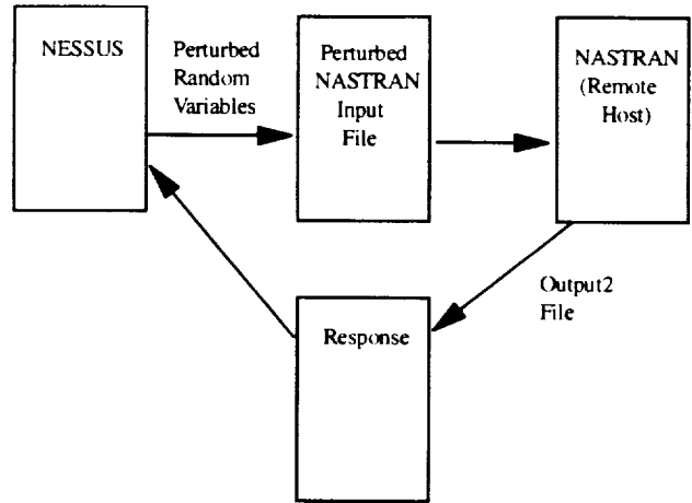
Figure 1. NESSUS/NASTRAN Schematic
