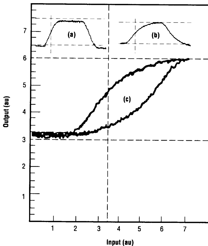
FIGURE 8.—The bistability loop of an 833-nm metal-free Pc film using a chopped CW He-Ne laser at 632.8 nm: (a) the input pulse, (b) the transmitted pulse, and (c) hysteresis switching constructed from (b).
