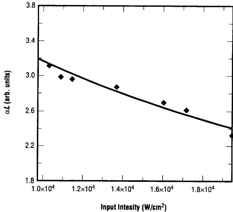
FIGURE 10.—Experimental and theoretical fitting of saturable absorption of a metal-free Pc film (232.5-nm thickness) at 632.8 nm from a CW He-Ne laser. The corresponding saturation intensity is 19.8 \times 10^3 \text{ W/cm}^2 .
