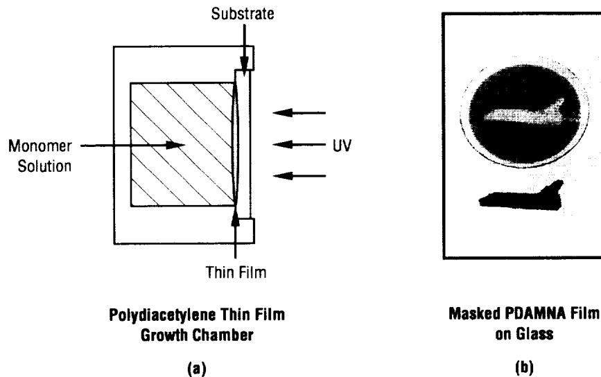
FIGURE 18.—(a) PDA thin film growth chamber, and (b) masked PDAMNA film on glass.
