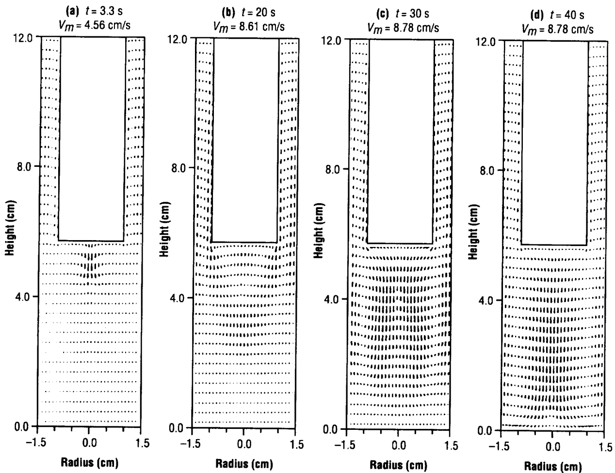
FIGURE 14.—Axisymmetric flow in the \theta = 0^\circ\text{--}180^\circ plane in cell in which deposition occurs with cell oriented vertically.
