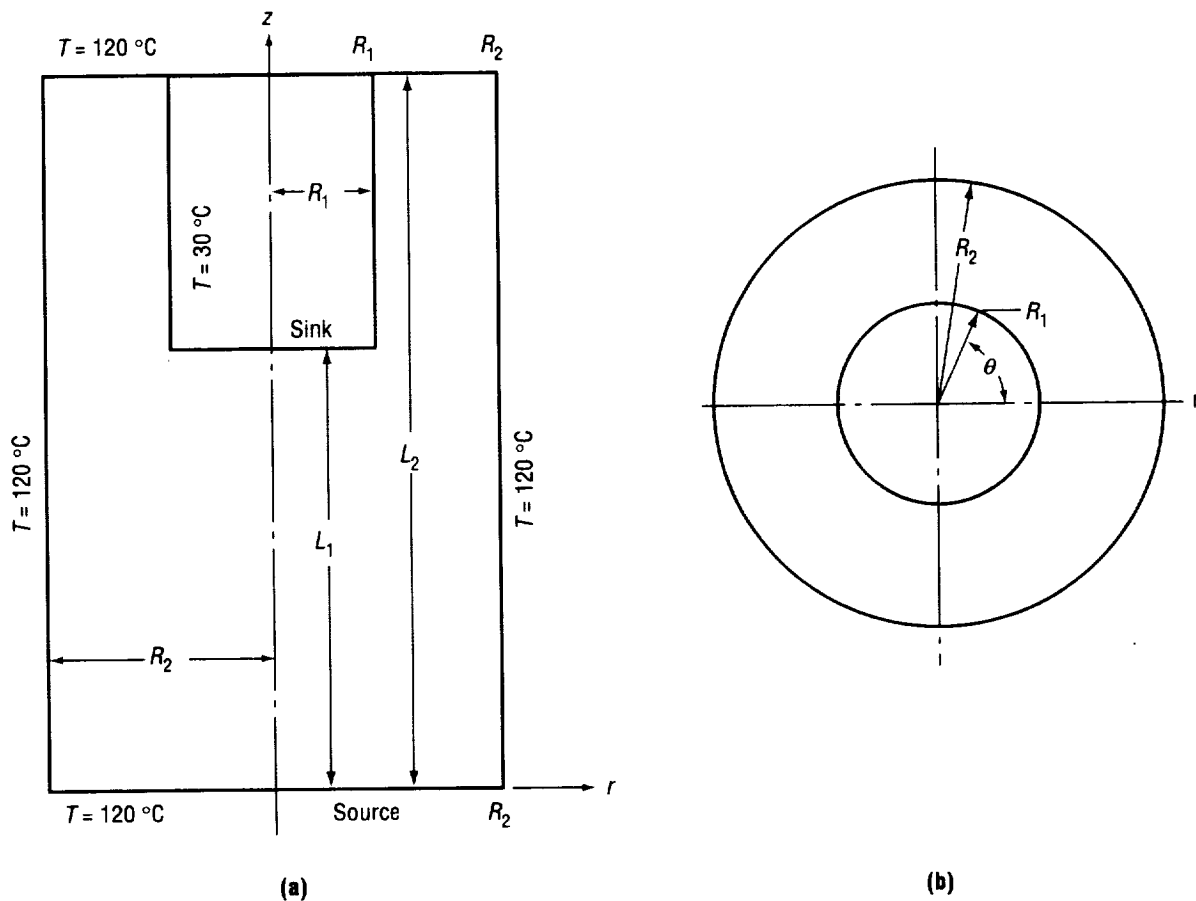
FIGURE 13.—Vapor deposition cell for PVT of DAMNA.
