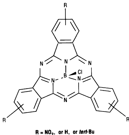
FIGURE 5.—Trinitro-substituted boron subPc.
