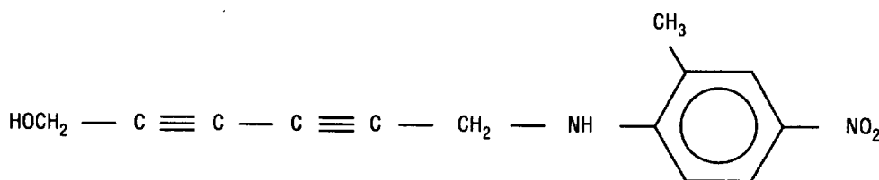
FIGURE 12.—Diacetylene monomer, DAMNA.
