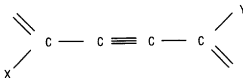
FIGURE 11.—Structure of PDA repeat unit.
