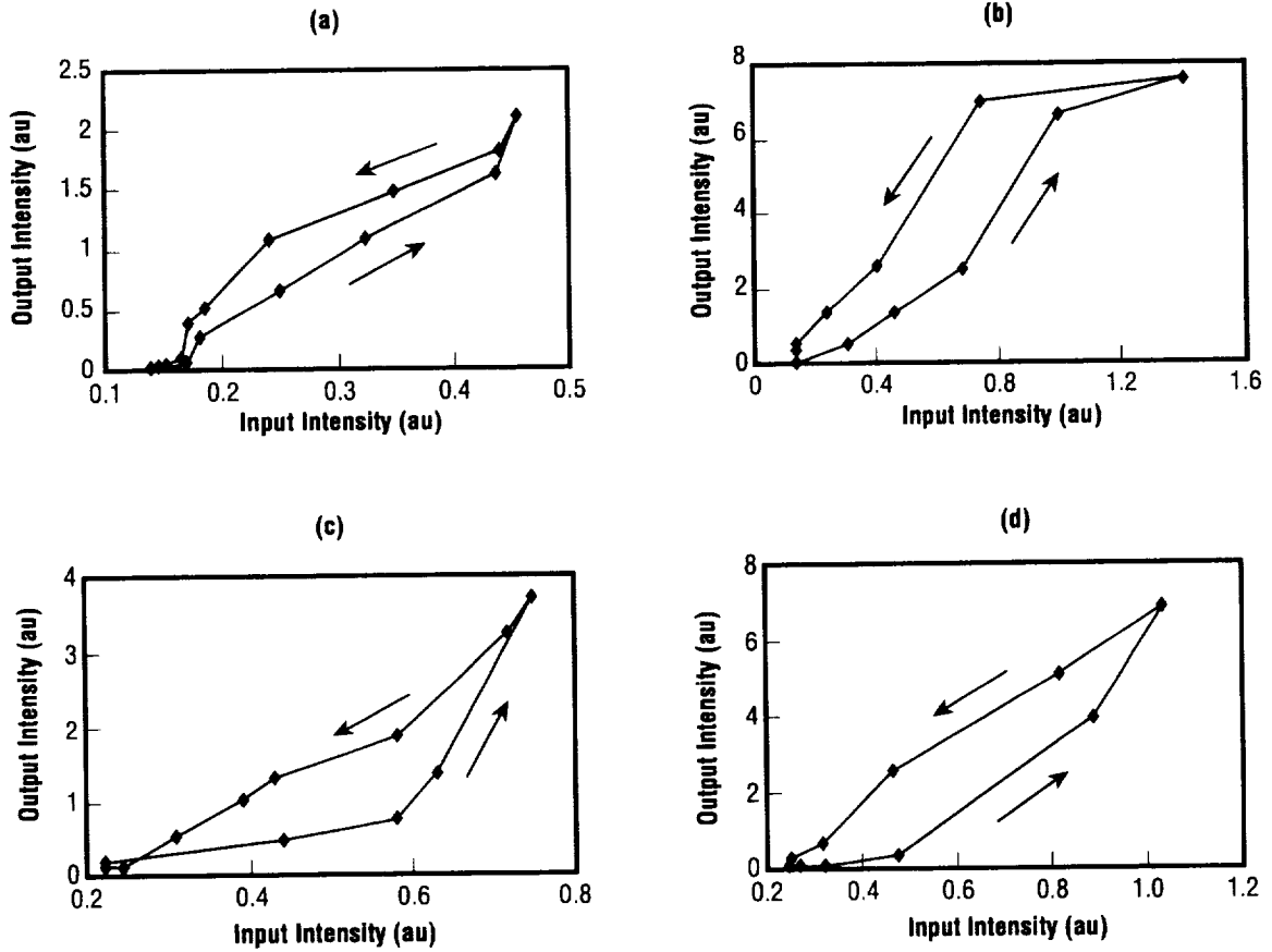
FIGURE 9.—The bistability loops for different timespans of a metal-free Pc film of 232.5-nm thickness using a CW He-Ne laser. Timespans between successive points are (a) 3.84 sec, (b) 10 sec, (c) 342 sec, and (d) 1,800 sec. (a) Shows the least prominent bistability loop while (b), (c), and (d) show a minimal effect of the timespan between points.
