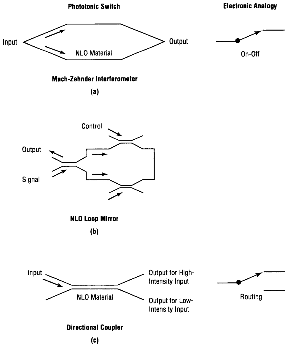
FIGURE 21.—(a) Mach-Zehnder interferometer, (b) NLO loop mirror, and (c) nonlinear directional coupler and their electronic analogs.
