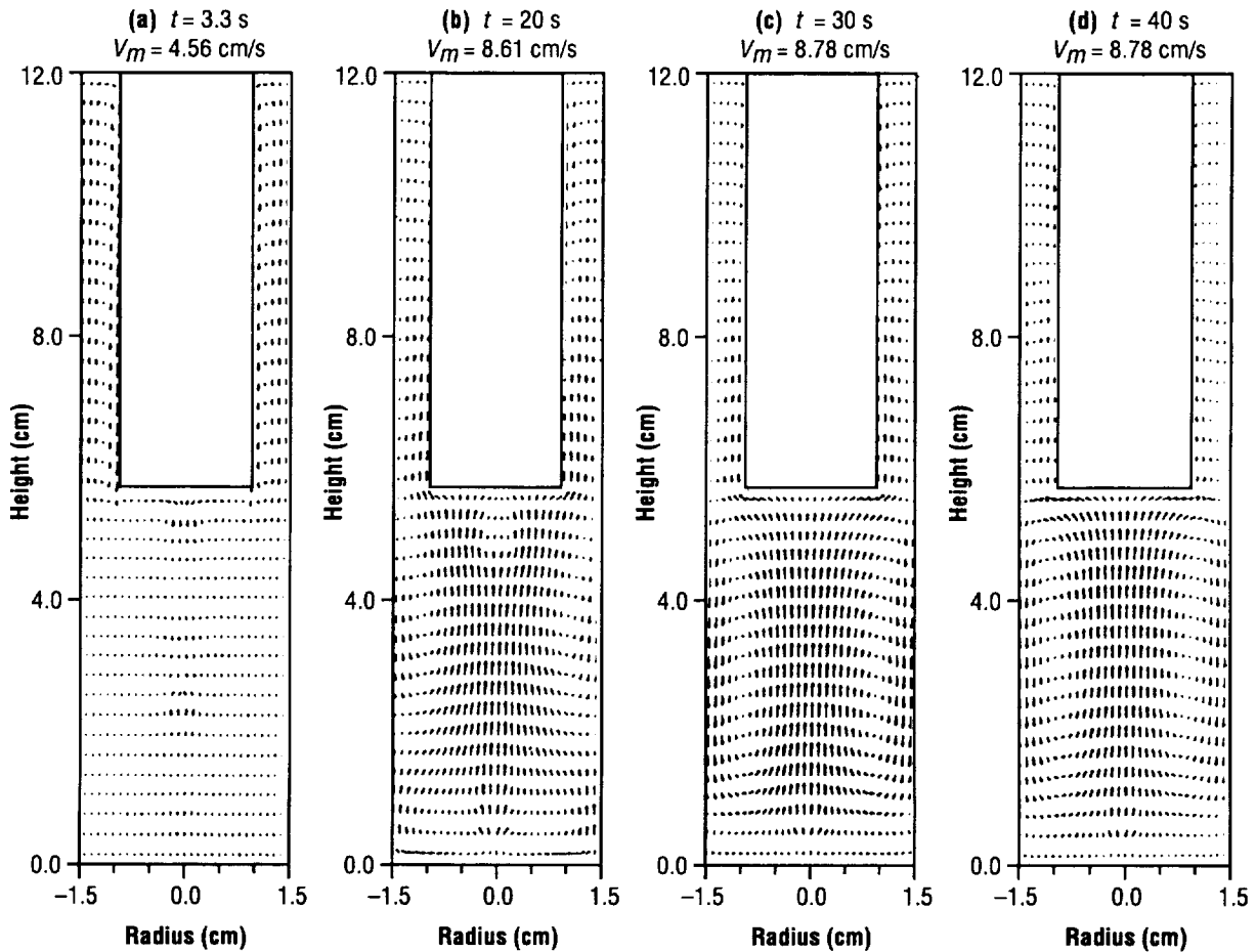
FIGURE 16.—Flow in the \theta = 90^\circ\text{--}270^\circ plane in cell in which deposition occurs with cell tilted 45^\circ to vertical axis.
