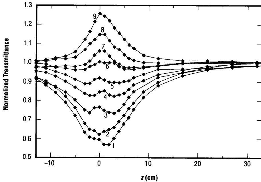
FIGURE 2.—Elimination of induced absorption in HITCI by the addition of small Au particles. For each z -scan the peak power was P_i = 0.16 MW and the on-axis peak irradiance at focus was I_o = 2.1 GW/cm 2 .
