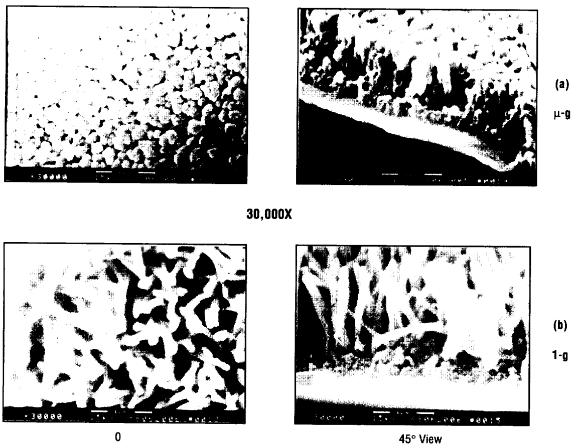
FIGURE 6.—CuPc films epitaxially vapor-deposited onto copper substrate: (a) \mu -g deposition of CuPc epilayer, and (b) 1-g deposition of CuPc epilayer (courtesy of 3M Corporation).
