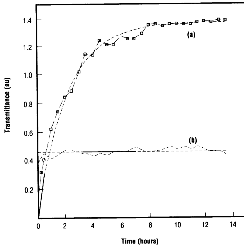
FIGURE 7.—(a) Time-dependent transmittance through a metal-free Pc film (230-nm-thick), using a CW He-Ne laser at 632.8 nm and 30 mW power. The dotted curve represents the experimental data, while the solid line represents a single exponential theoretical fit. (b) The dotted line represents laser stability throughout the experiment, while the solid line is the corresponding straight-line fit.
