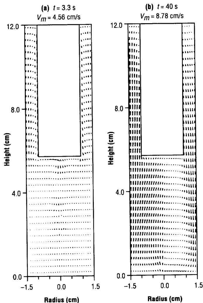
FIGURE 15.—Flow in the \theta = 0^\circ – 180^\circ plane in cell in which deposition occurs with cell tilted 45^\circ to vertical axis.
