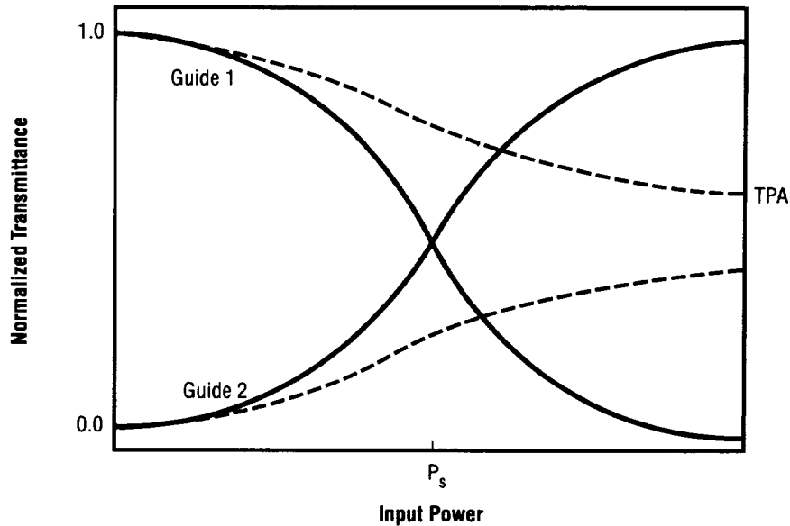
FIGURE 1.— Effect of TPA on an NLDC. The coupler is initially in a crossed state. Increasing the input power perturbs the coupling, resulting in switching, but the presence of the TPA suppresses switching.
