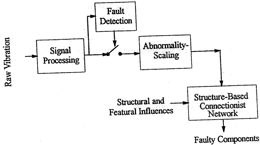
Figure 1: Overview of fault detection and diagnosis in the proposed structure-based diagnostic system for helicopter gearboxes.
