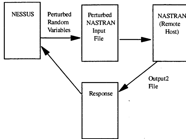
Figure 1. NESSUS/NASTRAN Schematic
