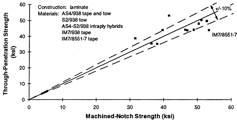
Figure 5-4. Comparison of the Residual Tensile Strength of Laminates with Through-Penetrations and Machined Notches.
