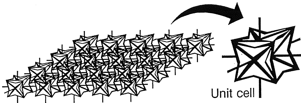
Figure 4-8. Cellular Core Material with Re-Entrant Microstructure.
