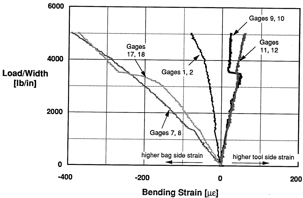
Figure E-10: Load-bending strain behavior for specimen DEMO1-42 (solid plug in ramp, compression).
