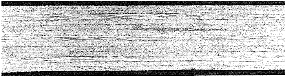
Figure 4-2. Microstructure of an AS4/938 Laminate Fabricated with the Automated Fiber Placement Process (BCA Head).
