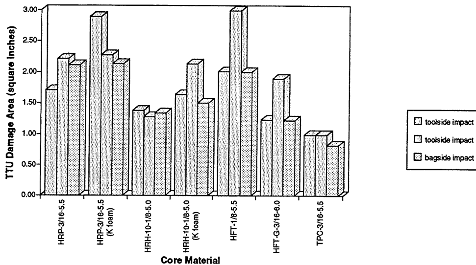
Figure F-5. Bagside and Tootside Impact Damage Resistance of Representative Minimum Gage Sandwich Structure (Damage Area).
