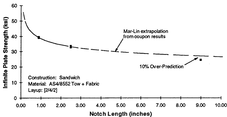
Figure 5-7. Prediction of Large Notch Strength from Small Notch Data with the Functional Form of the Mar-Lin Fracture Model ([X/Y/Z] indicates the number of plies in the [0/±45/90] orientations).
