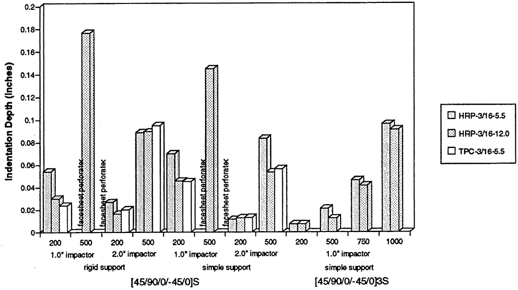
Figure G-5: Effect of Core Material Type and Density on Indentation Depth in Composite Sandwich Structures.
