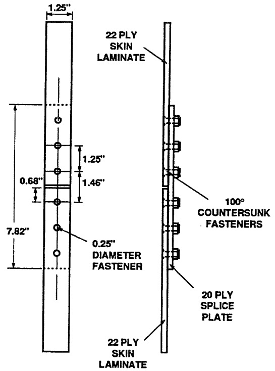
CIRCUMFERENTIAL SKIN SPLICE SPECIMEN
