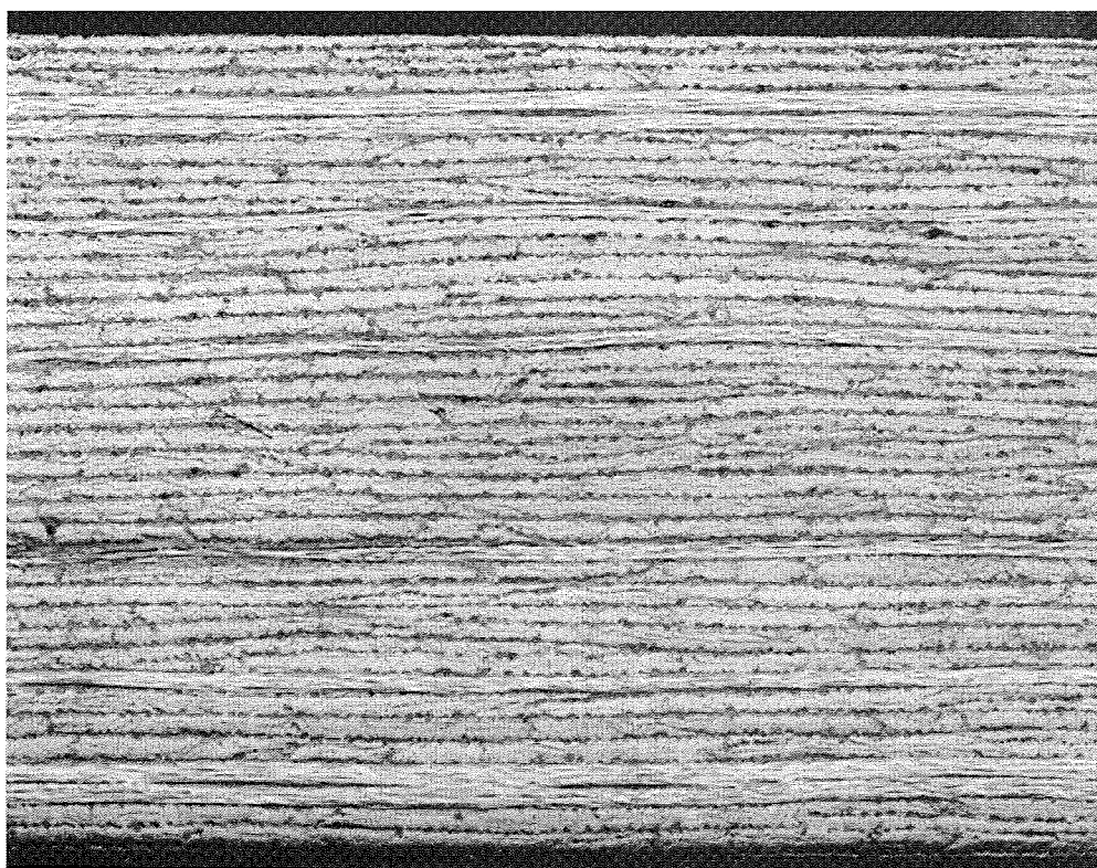
Figure 4-5. Microstructure of an AS4/8553-40 Interlayer Particulate Toughened Laminate Fabricated with the Automated Fiber Placement Process (BCA Head).
