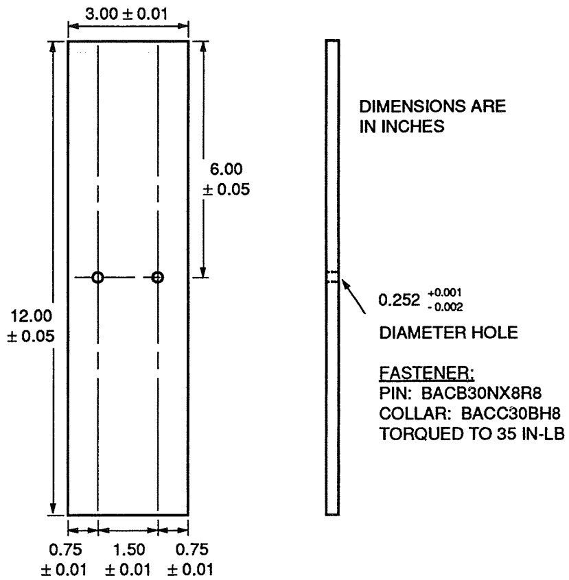
Figure D-5: Transverse bearing-compression bypass specimen configuration.
