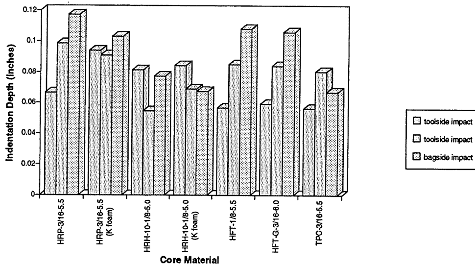
Figure F-4. Bagside and Tootside Impact Damage Resistance of Representative Minimum Gage Sandwich Structure (Indentation Depth).
