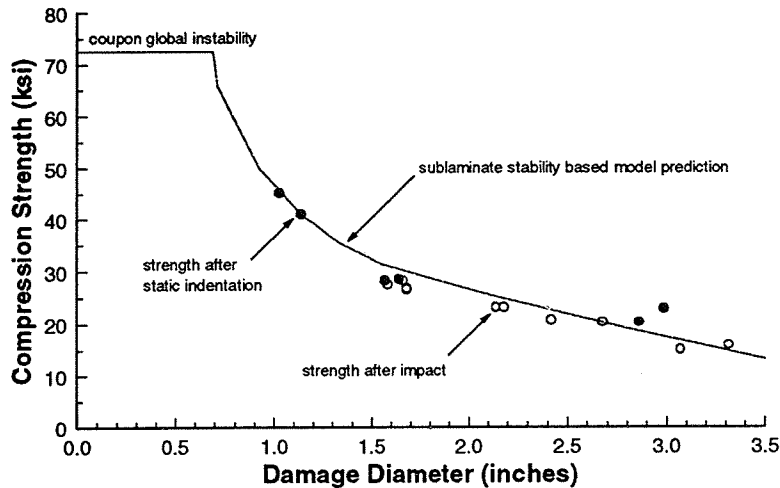
Figure 6-2. Correlation of Sublaminare Stability Based CAI Strength Prediction with Experimental Data for Damage Induced by Impact and by Static Indentation.
