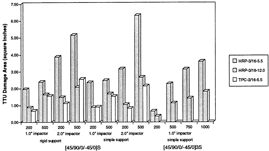
Figure G-6: Effect of Impactor Diameter on Damage Area in Composite Sandwich Structures.
