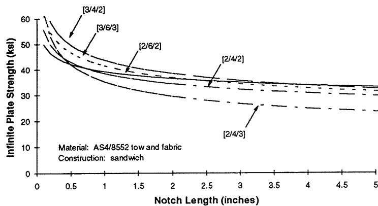
Figure 5-9. Influence of Layup on Tensile Notch Sensitivity of AS4/8552 Sandwich Structure ([X/Y/Z] indicates the number of plies in the [0/± 45/90] orientations).
