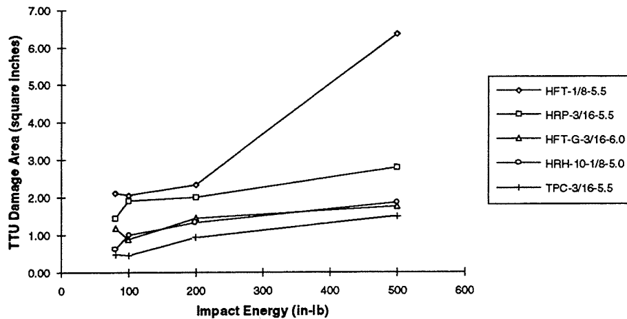
Figure 6-5. Impact Damage Resistance of Representative Minimum Gage Sandwich Structure with Candidate Honeycomb Core Materials.
