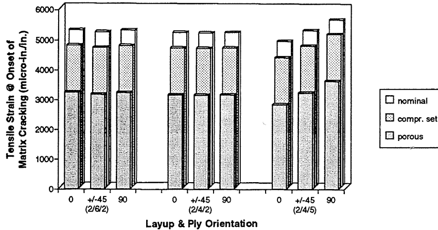
Figure 6-11 Estimated Tensile Strain at Onset of Matrix Cracking in AS4/8552 Facesheet Materials. (X/Y/Z) Indicates the Number of (0/± 45/90) Plies.
