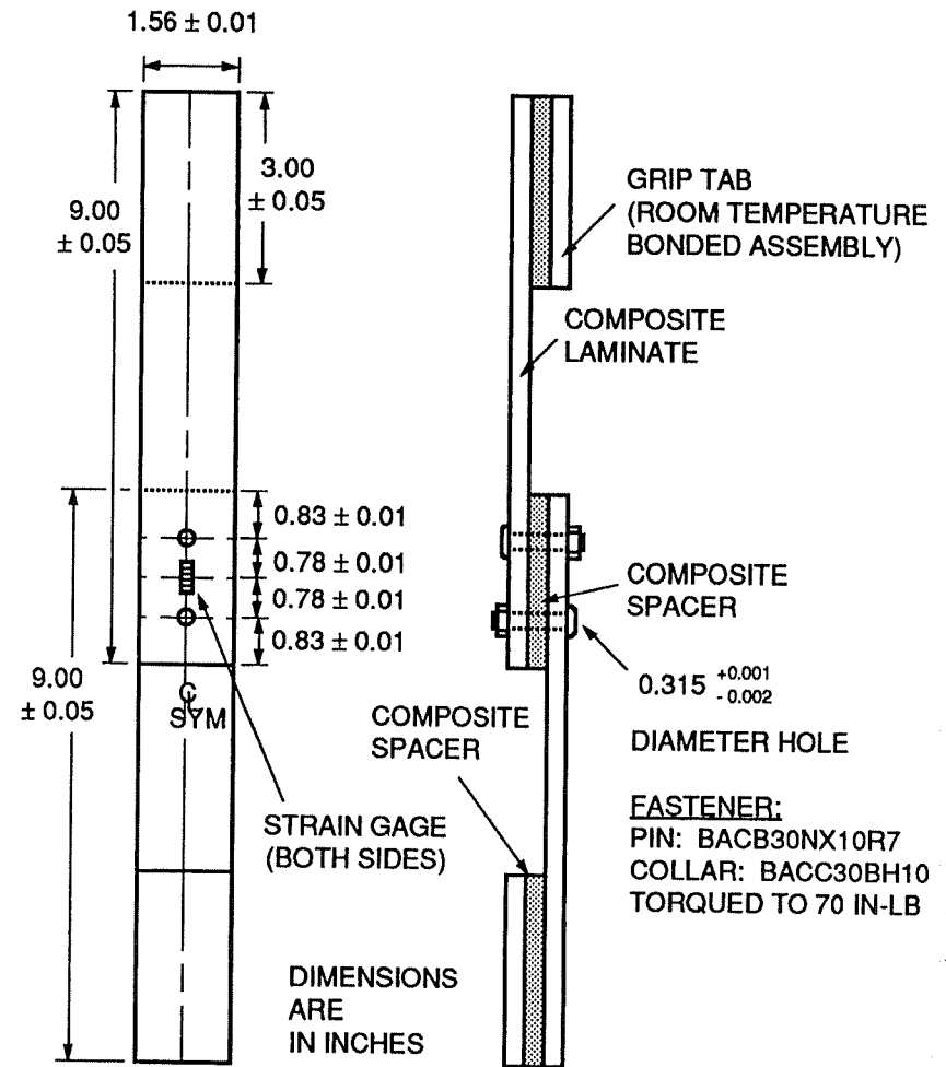
Figure D-22: 50% load transfer joint with structural spacer.
