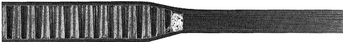
Figure 4-24. Aft Side Circumferential Panel Splice Core Close-Out Manufacturing Demonstration.
