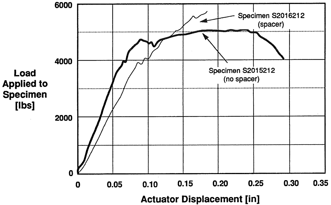
Figure D-23: Comparison of actuator displacement vs. load measurements for specimens with and without spacers.
