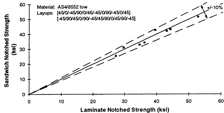
Figure 5-12. Comparable Tensile Notch Sensitivity of Laminate and Sandwich Structures.
