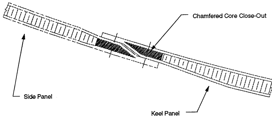
a. Ramped Core Close-Out
