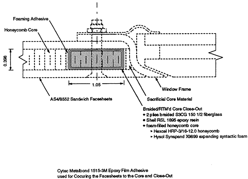
Figure 4-25. Window Cutout Core Close-Out Constructed of Braided and Resin Transfer Molded Tubes with Syntactic Foam Filled Honeycomb Core.
