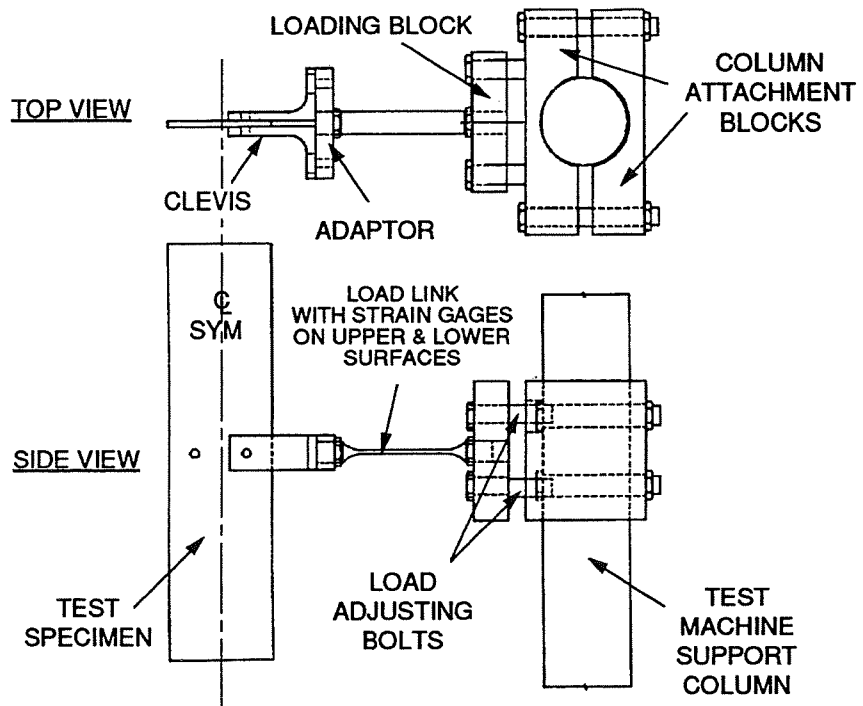
Figure D-6: Transverse loading apparatus.
