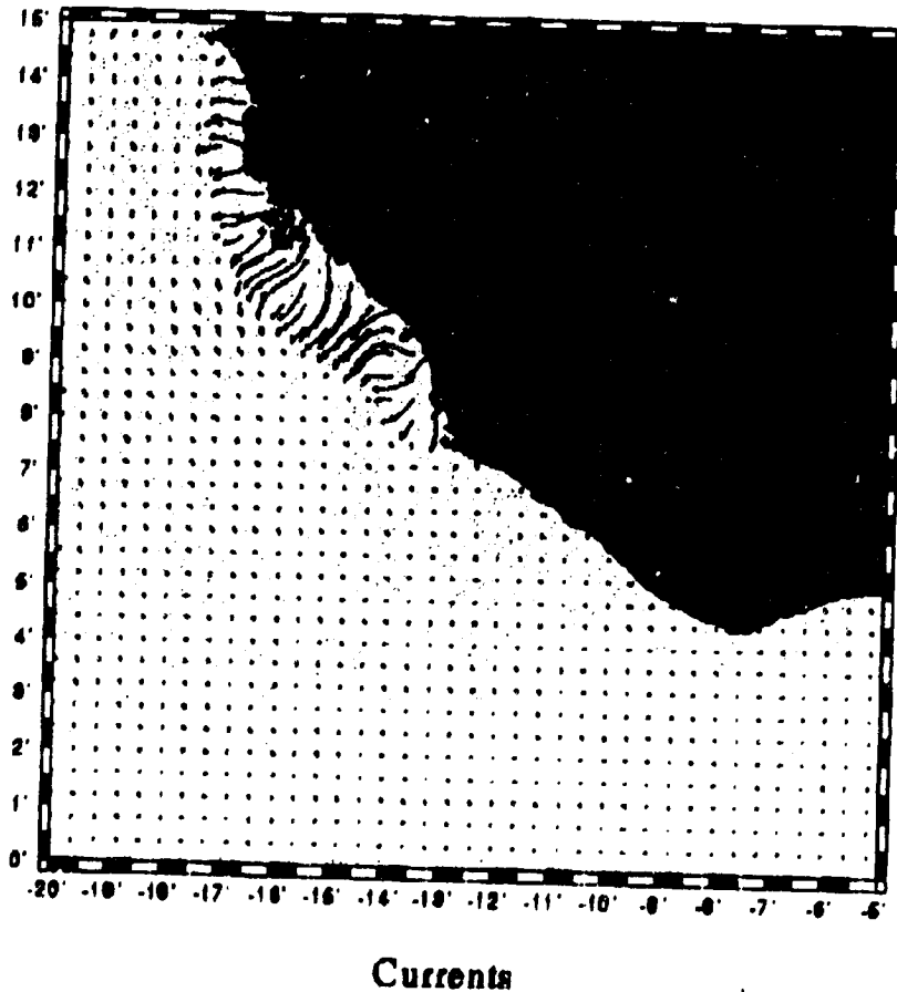
Figure 5. Streak-Plot of Tidal Currents for Coarse Grid Domain for 17 April.
