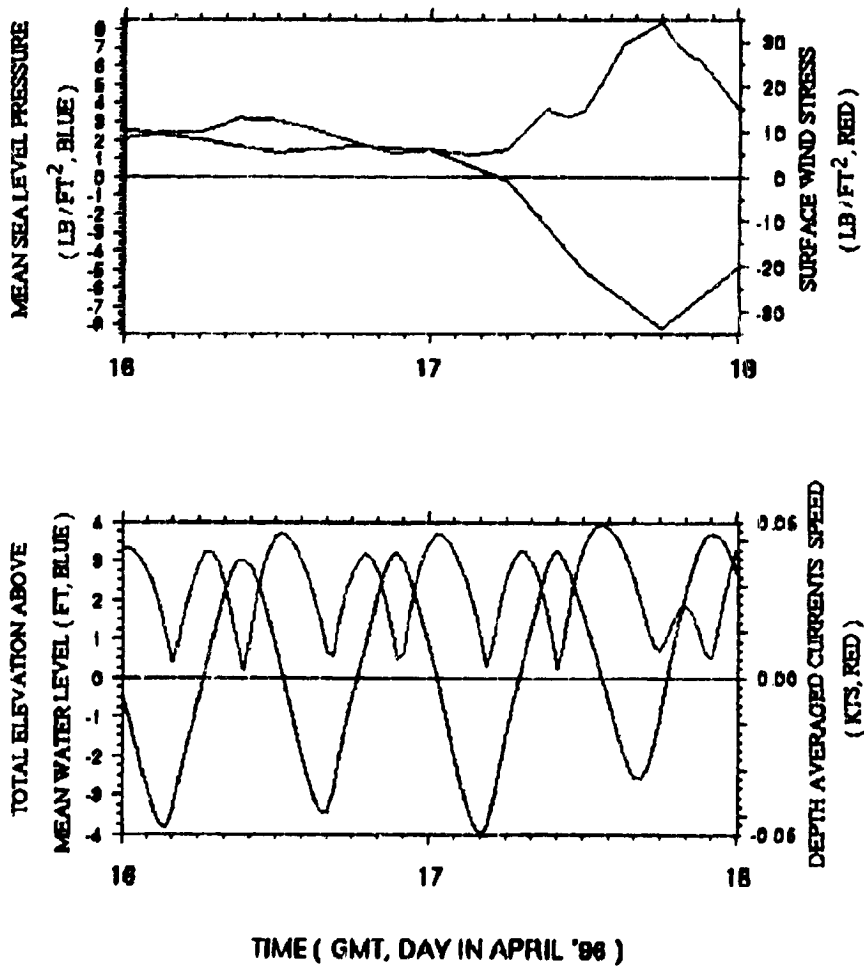
Figure 13. Time Series plots for Freetown ( Coarse Grid )
