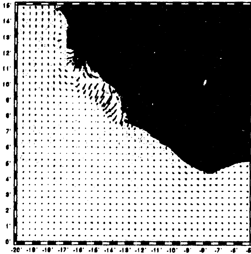
Figure 4. Streak-Plot of Tidal Currents for Coarse Grid Domain for 16 April.
