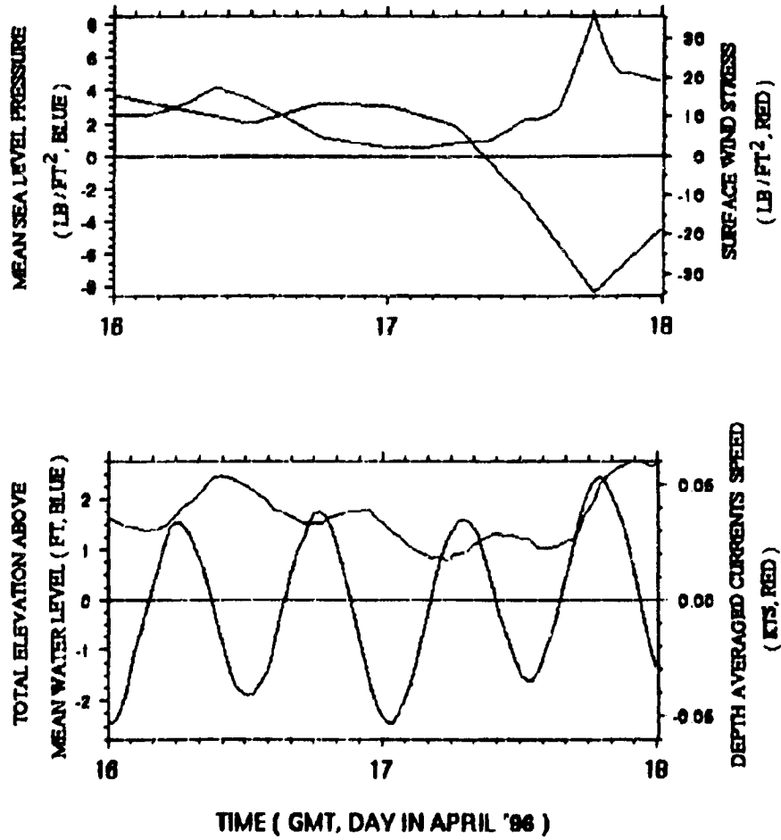
Figure 19. Time Series plots for Monrovia ( Fine Grid )
