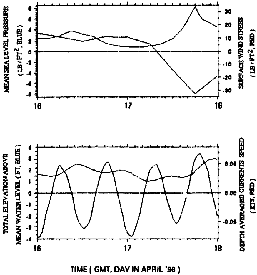
Figure 18. Time Series plots for Kasi ( Fine Grid )
