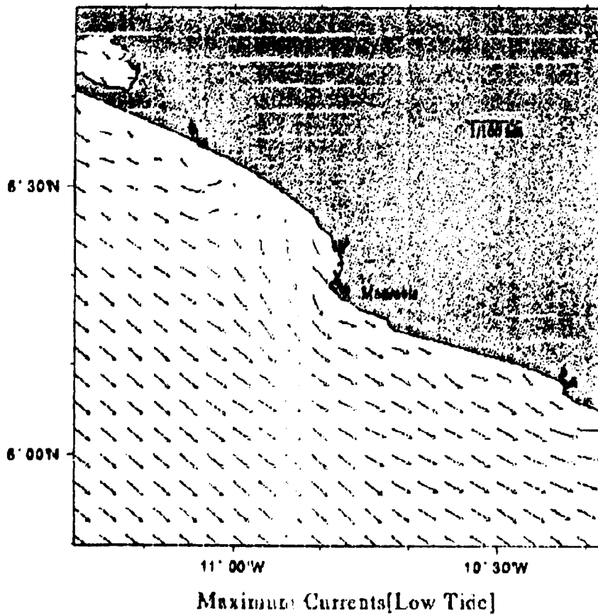
Figure 10. Maximum Currents at Monrovia at Low Tide ( Fine Grid )
