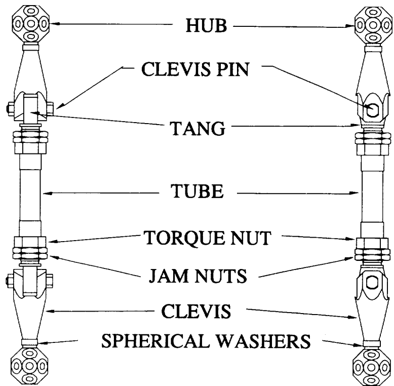
Fig. 5. Illustration of the strut design.
