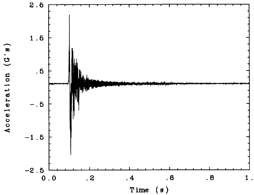
Fig. 105. Torsion twang test recorded on the GAS bridge during Space Shuttle integration.
