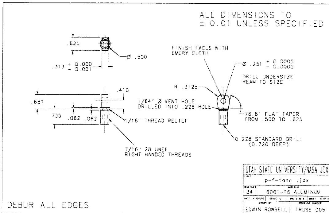
Fig. 82. JDX tang design.
