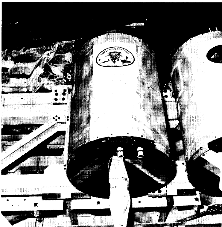
Fig. 41. Photograph of JDX attached to the GAS bridge.
