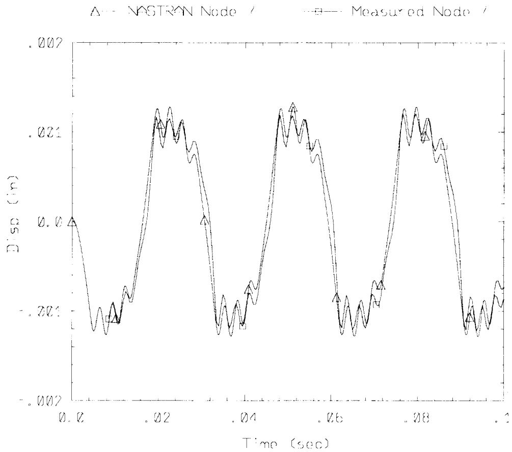
Fig. 63. Comparison of the finite element model to measured data for a short strut with a 0.1862 inch pin and a 35 Hz. forcing frequency.
