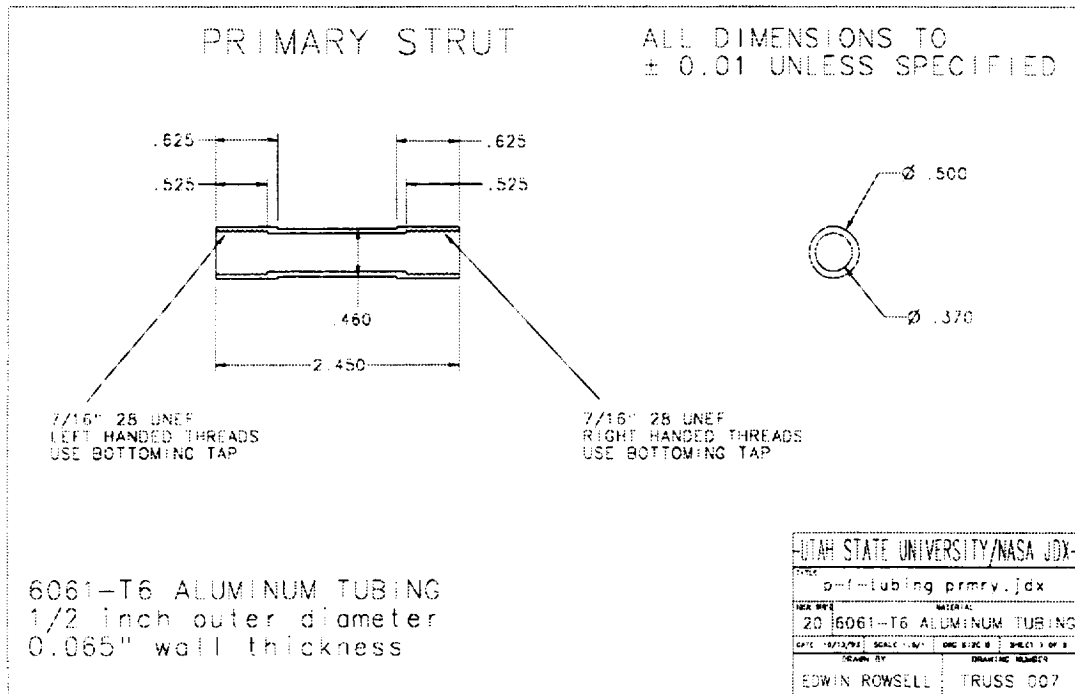
Fig. 83. JDX short tube design.
