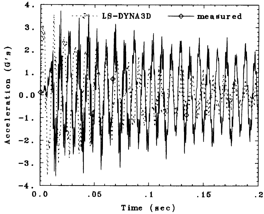
Fig. 75. Torsion test acceleration for a locked truss.
