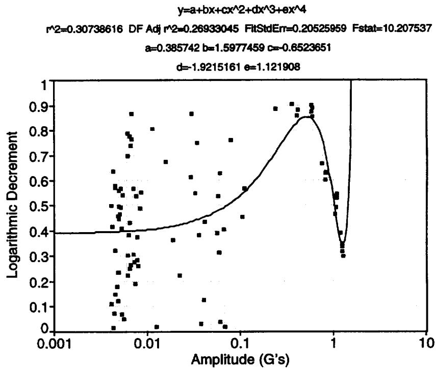
Fig. 139. Cold cell bend 2 test at 20° C.
