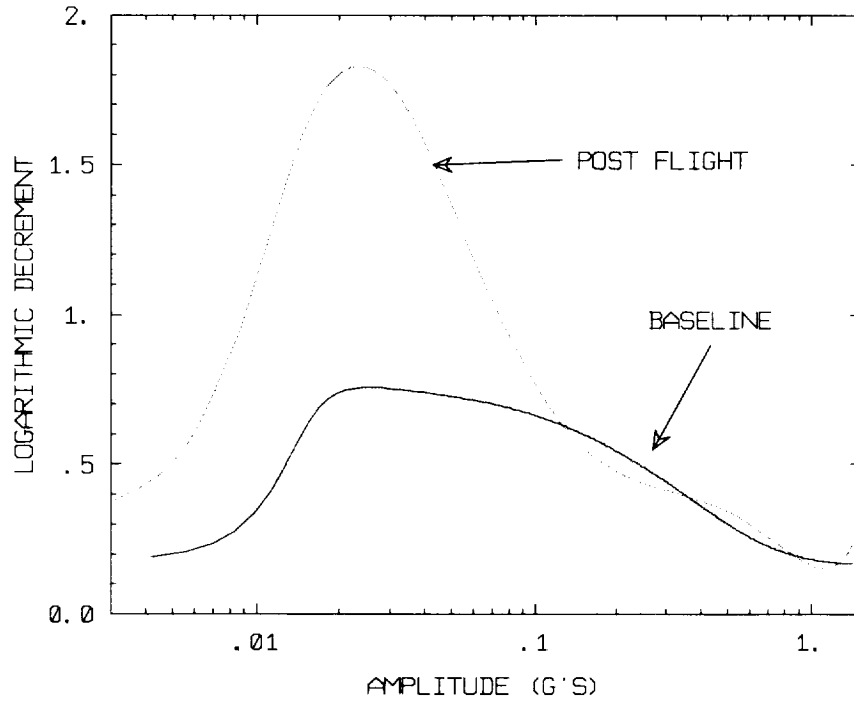
Fig. 52. Comparison of bend 1 mode damping from baseline and post flight tests.
