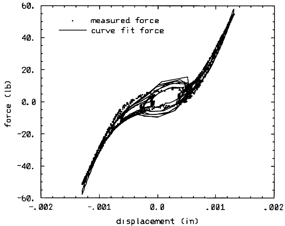
Fig. 58. Plot showing the data for the short strut with a 0.1862 inch pin and 1 Hz. forcing frequency compared to the curve fit given by Eq. 4.
