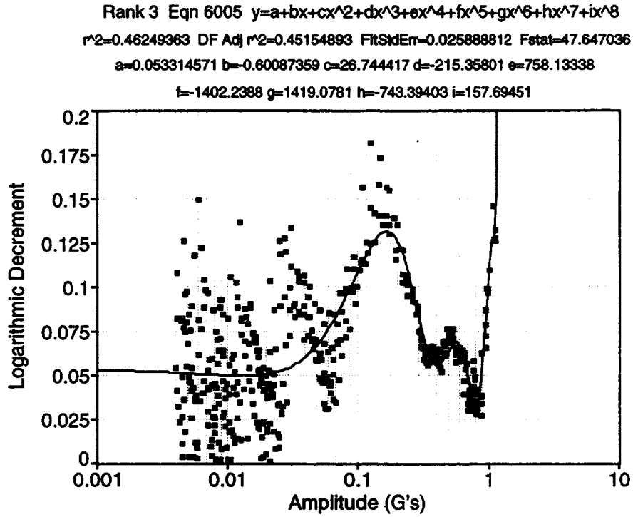
Fig. 122. Baseline bend 1 test, upper peaks, in the 90° truss orientation.
