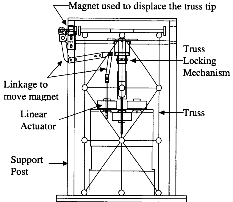
Fig. 10. Illustration of the Bend 1 mode excitation system and the truss locking mechanism.
