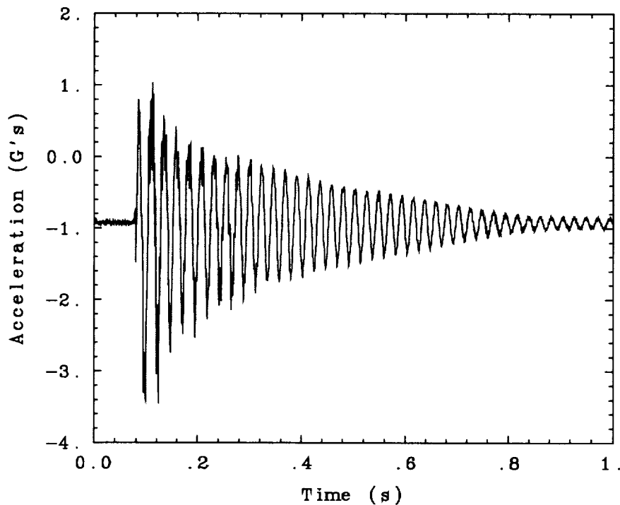
Fig. 26. Bend 1 mode baseline twang test in the 90° truss orientation.
