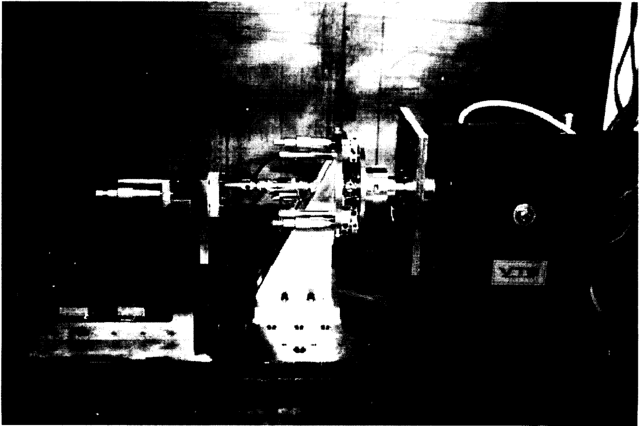
Fig. 54. Photograph of the Force State Map test setup.
