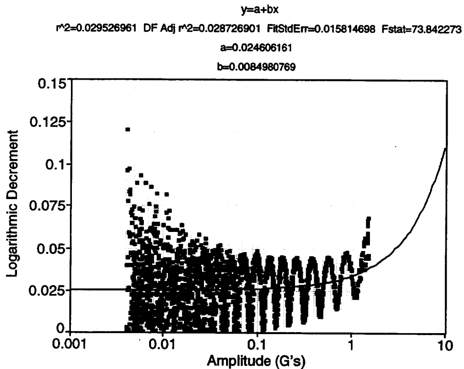
Fig. 133. Bend 2 test in the 0° truss orientation with all joints locked.
