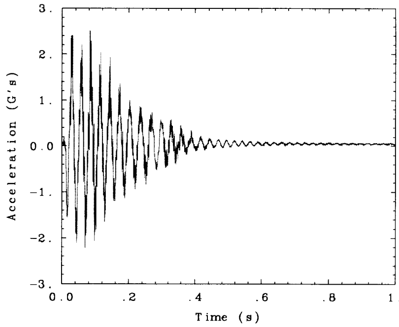
Fig. 20. Bend 1 mode twang test with pin set 2, 0° truss orientation.
