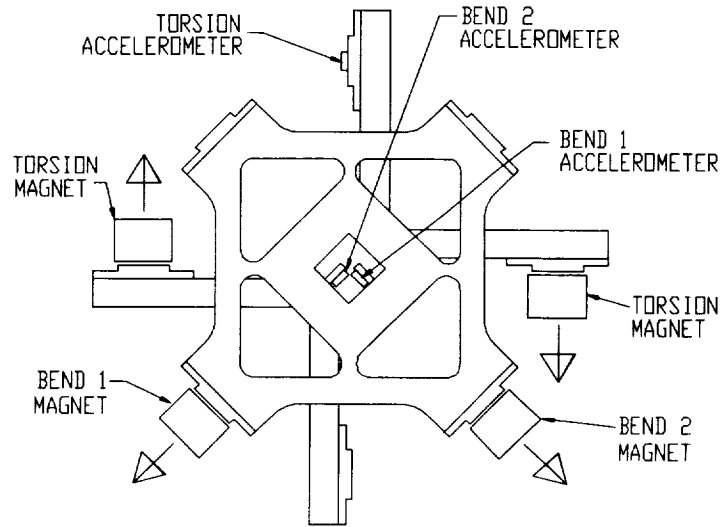
Fig. 9. Top view of the tip mass showing the magnets and the accelerometer locations.
