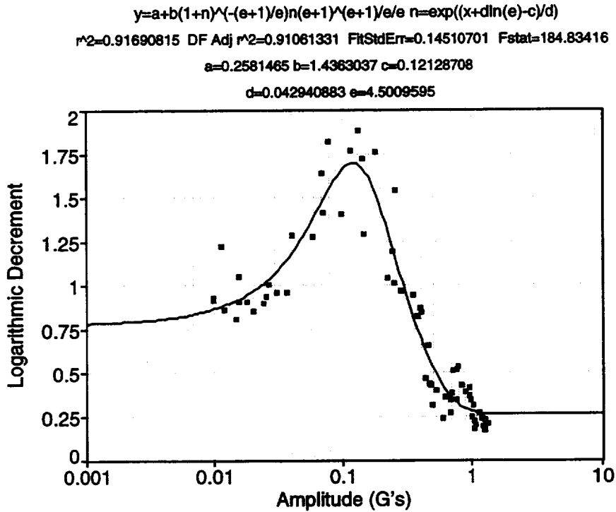
Fig. 130. Low-G bend 1 test.
