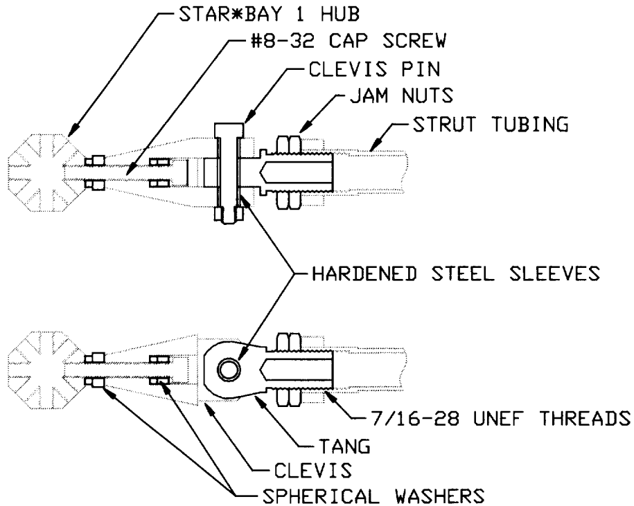
Fig. 6. Illustration of the pinned joint design.
