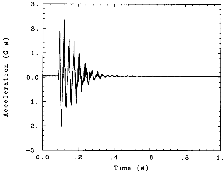
Fig. 108. Bend 1 twang test recorded during cold cell tests at 10° C.
