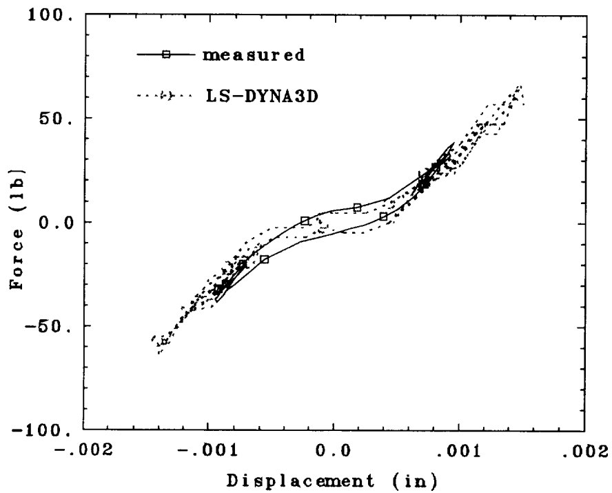
Fig. 67. Measured and predicted hysteresis curves.
