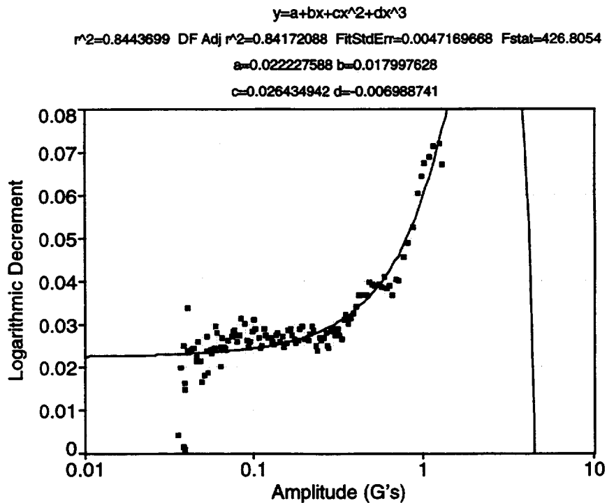
Fig. 119. Bend 1 test, lower peaks, in the 90° truss orientation using pin set two.
