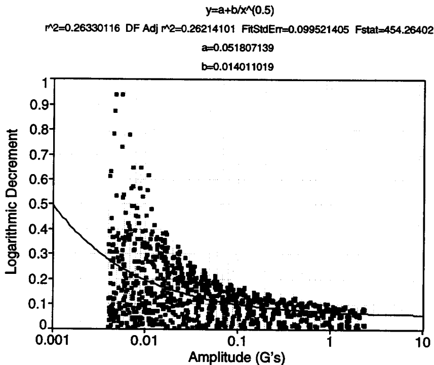
Fig. 149. Baseline torsion test, upper peaks, in the 90° truss orientation.
