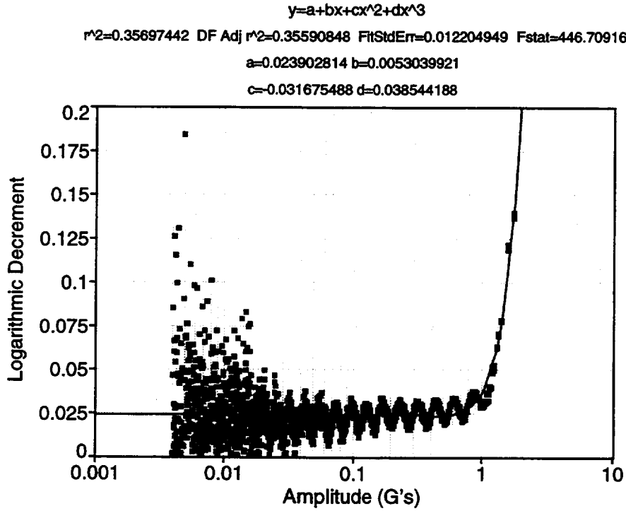
Fig. 112. Bend 1 test in the 0° truss orientation with all joints locked.
