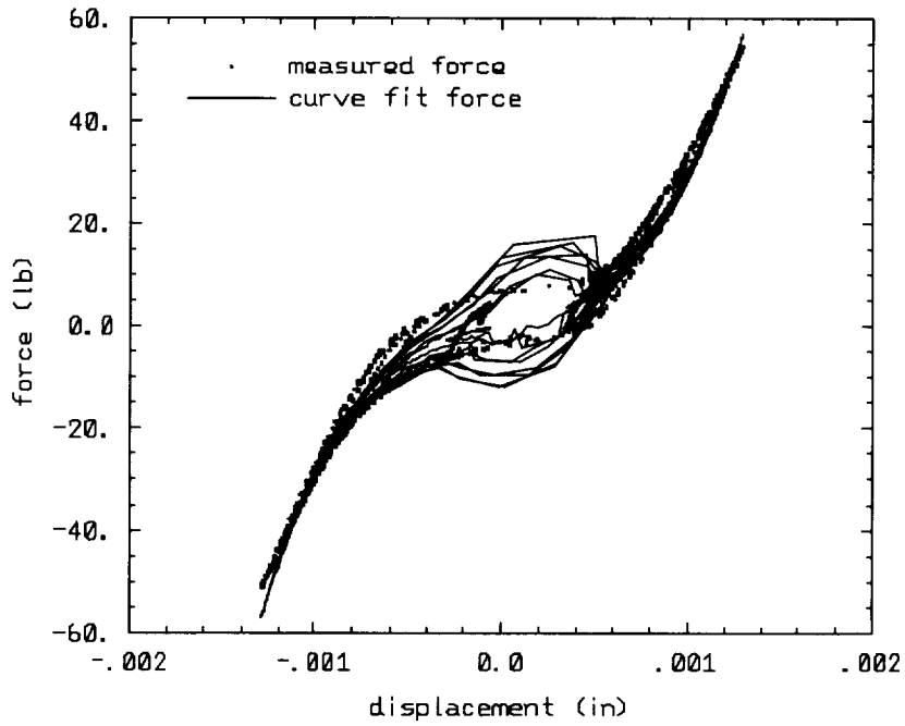
Fig. 56 Plot showing the data for the short strut with a 0.1862 in. pin and 1 Hz forcing frequency compared to the curve fit given by Eq. 2.
