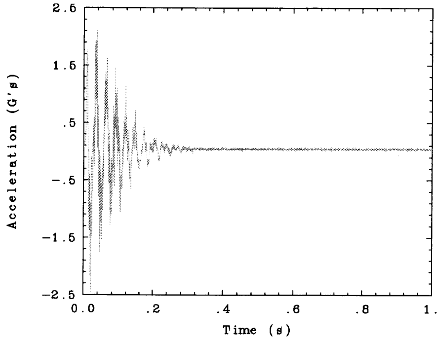
Fig. 91. Bend 2 twang test using pin set three in the 0° truss orientation.
