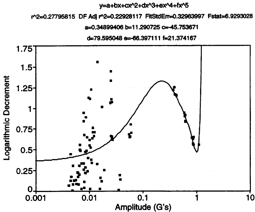
Fig. 143. Cold cell bend 2 test at -20° C.
