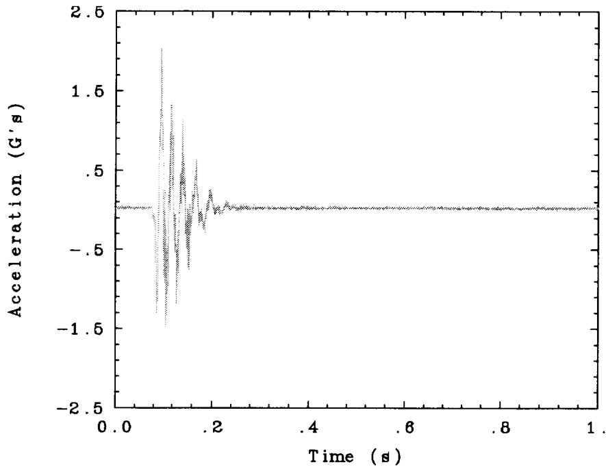
Fig. 96. Bend 2 twang test recorded during low-G flight.
