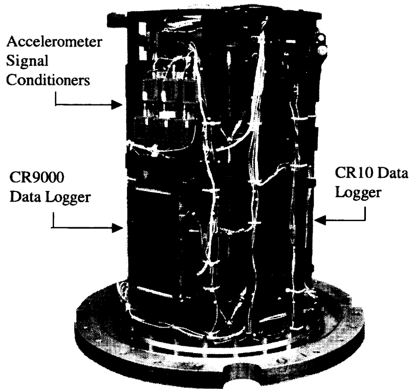
Fig. 11. Photograph of JDX showing the locations of the CR10 and CR9000 data loggers and the accelerometer signal conditioners.
