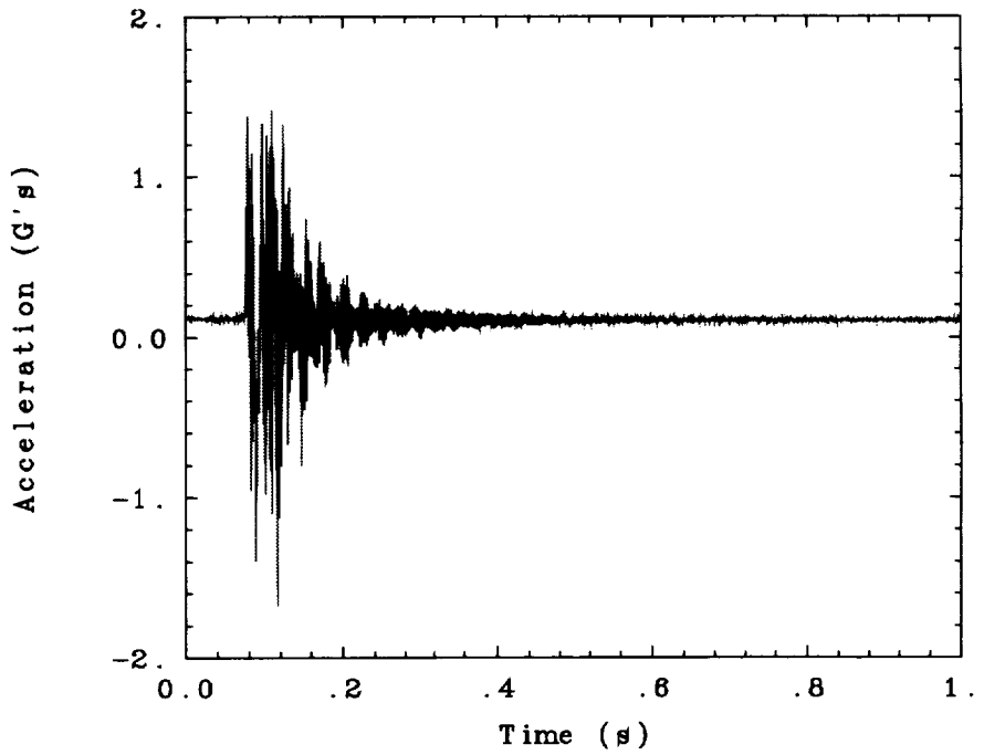
Fig. 106. Torsion twang test recorded during Space Shuttle flight.
