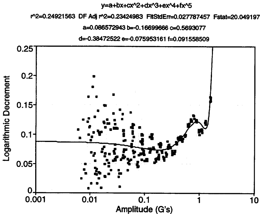
Fig. 137. Baseline bend 2 test, upper peaks, in the 90° truss orientation.
