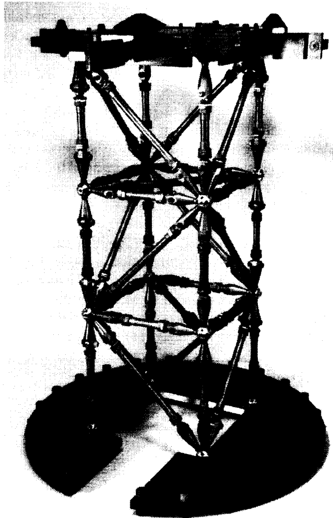
Fig. 1. Photograph of the truss.
