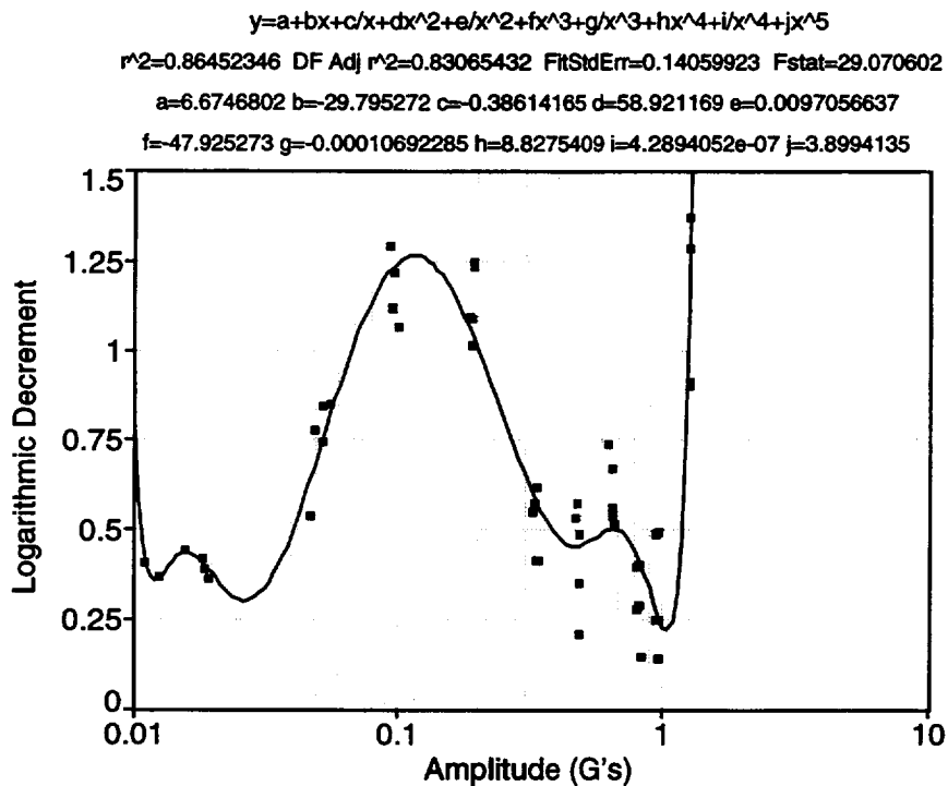
Fig. 145. Bend 2 test during the Space Shuttle flight.
