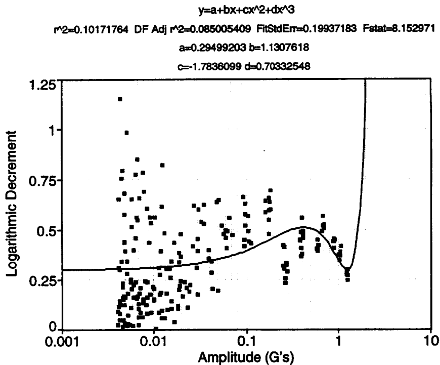
Fig. 135. Baseline bend 2 test in the 0° truss orientation.
