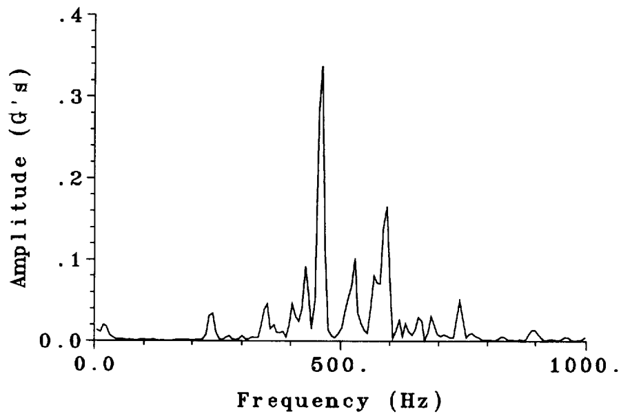
Fig. 80. Predicted torsion test frequencies for unlocked truss in micro gravity.
