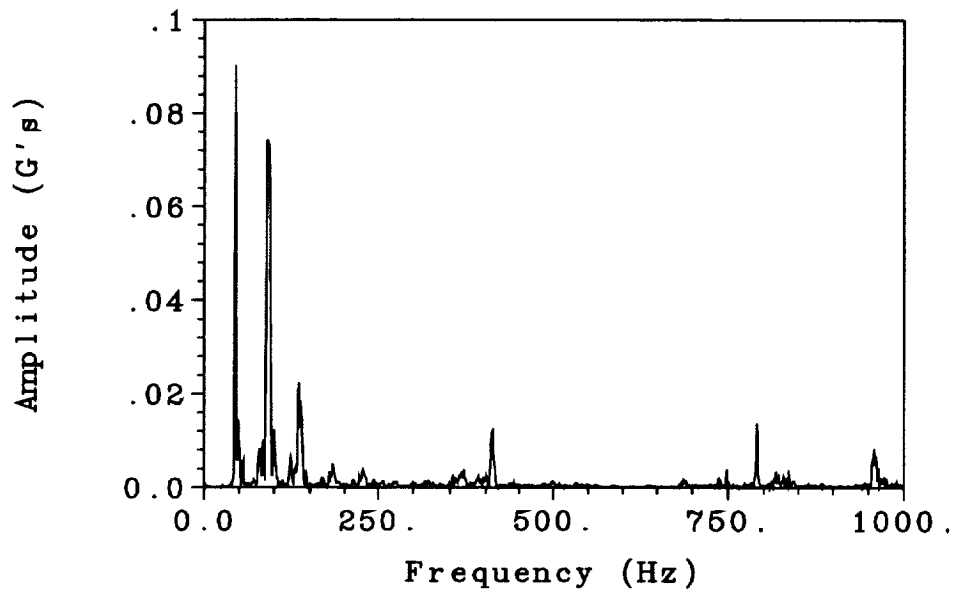
Fig. 39. FFT of a torsion mode twang test of the Flight Model truss in a 90° truss orientation.
