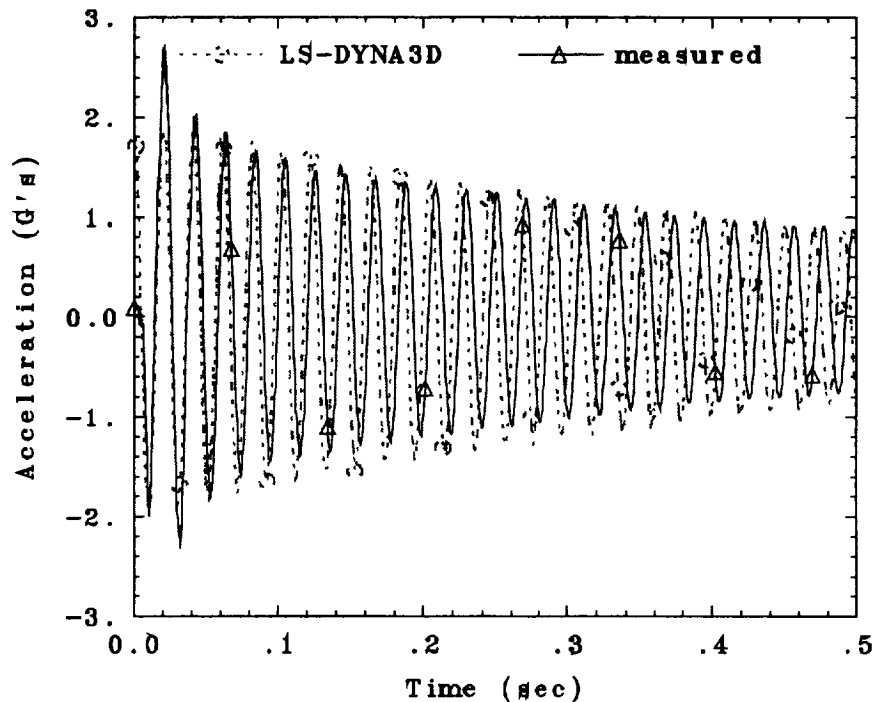
Fig. 71. Bend 1 acceleration for a locked truss in 0-deg orientation.
