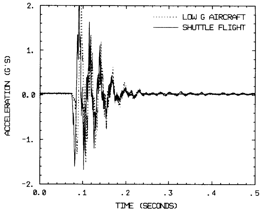
Fig. 49. Comparison of bend 2 mode twang tests from Shuttle flight and low-G tests.
