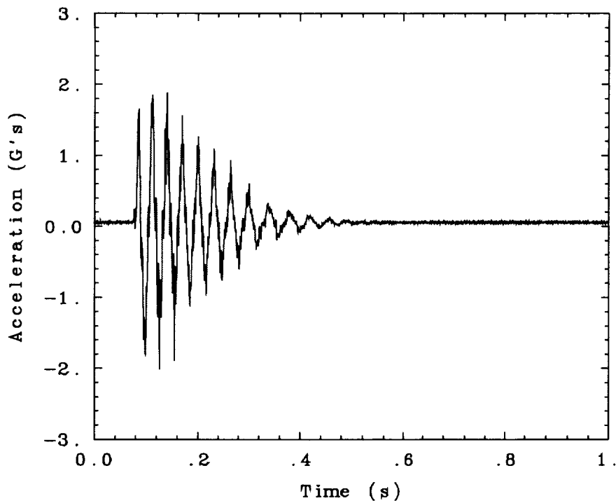
Fig. 25. Bend 1 mode baseline twang test in the 0° truss orientation.
