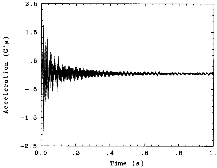
Fig. 99. Torsion test using pin set one in the 0° truss orientation.
