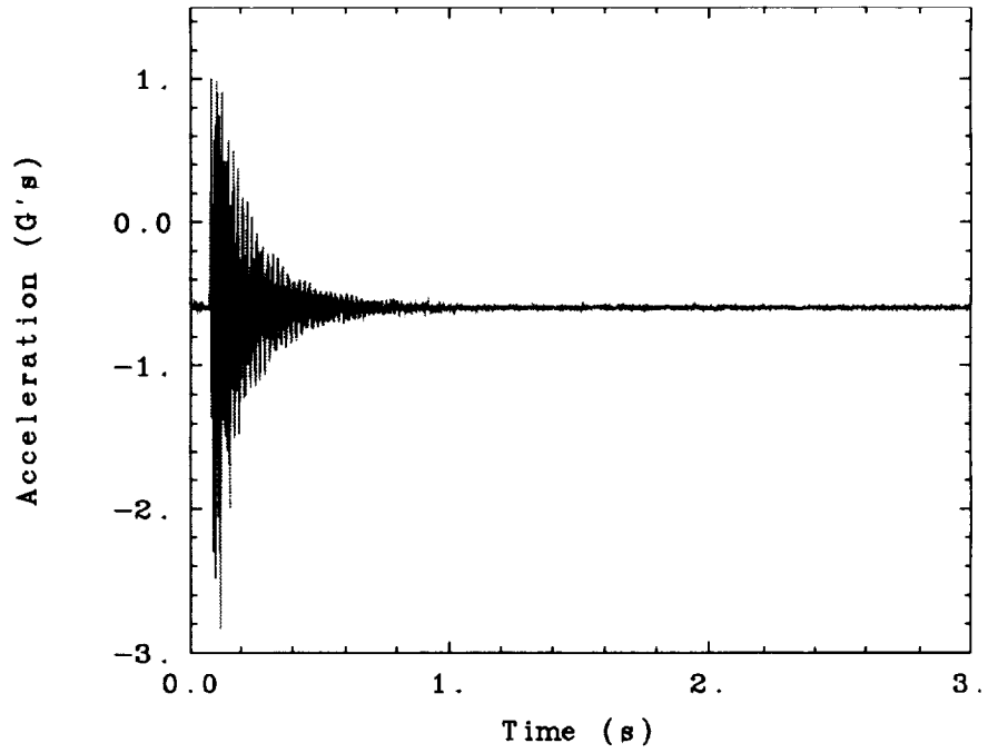
Fig. 102. Baseline torsion twang test in the 90° truss orientation.
