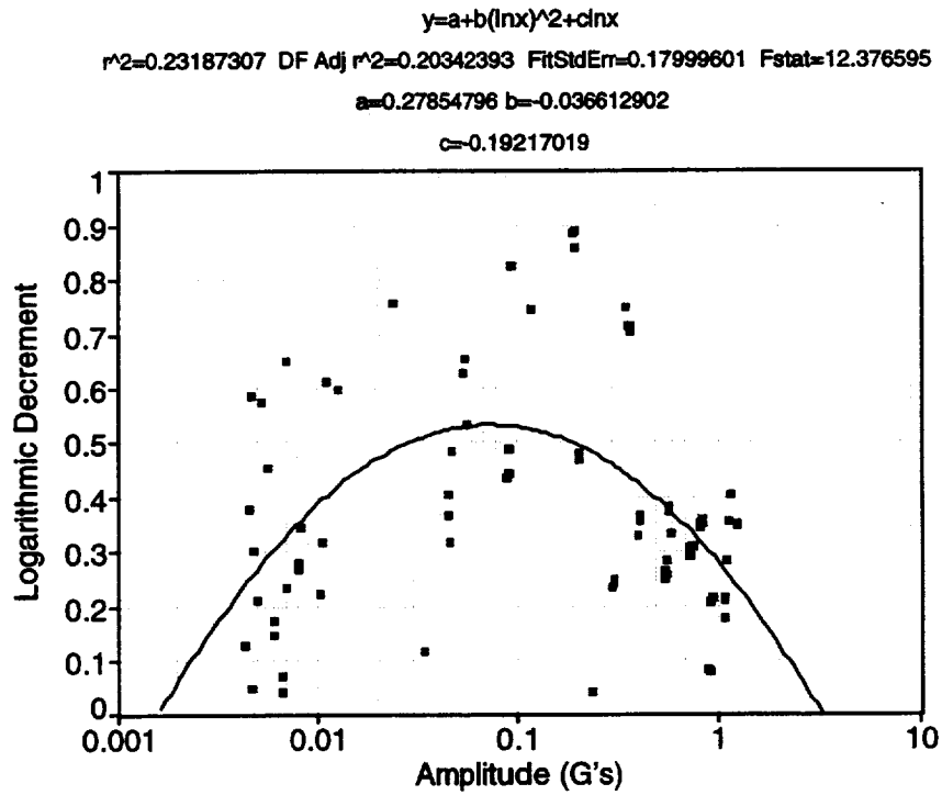
Fig. 134. Bend two test in the 0° truss orientation using pin set three.
