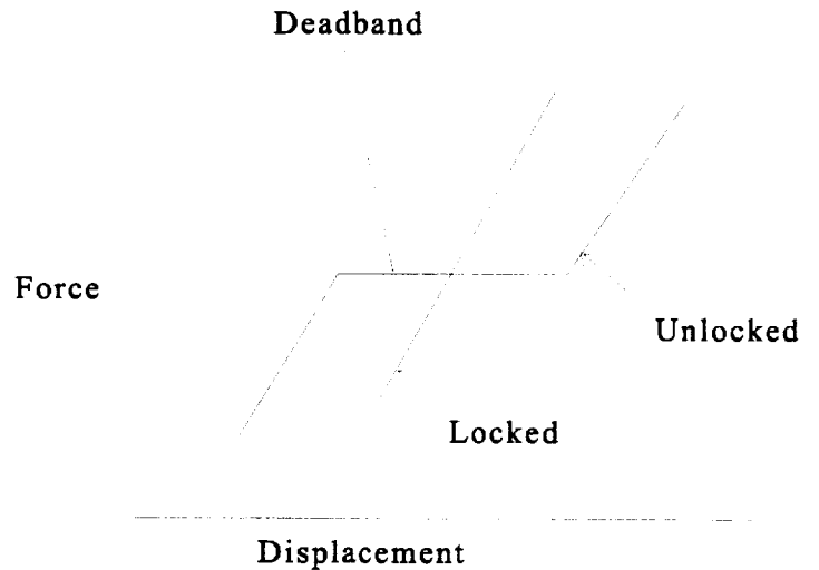
Fig. 7. Illustration of joint deadband effects on the force-displacement relationship of a strut.
