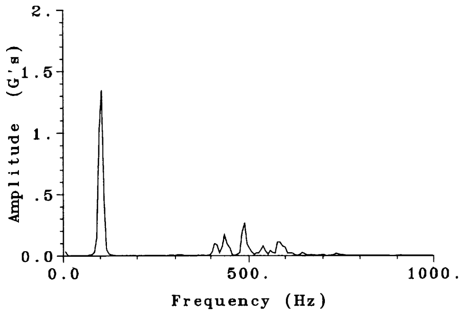
Fig. 78. Predicted torsion test frequencies for locked truss in 0° truss orientation.
