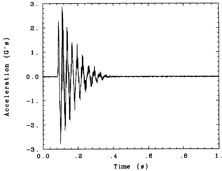
Fig. 109. Bend 1 twang test recorded during cold cell tests at 0° C.
