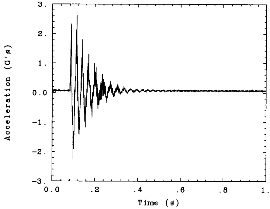
Fig. 107. Bend 1 twang test recorded during cold cell tests at 20° C.
