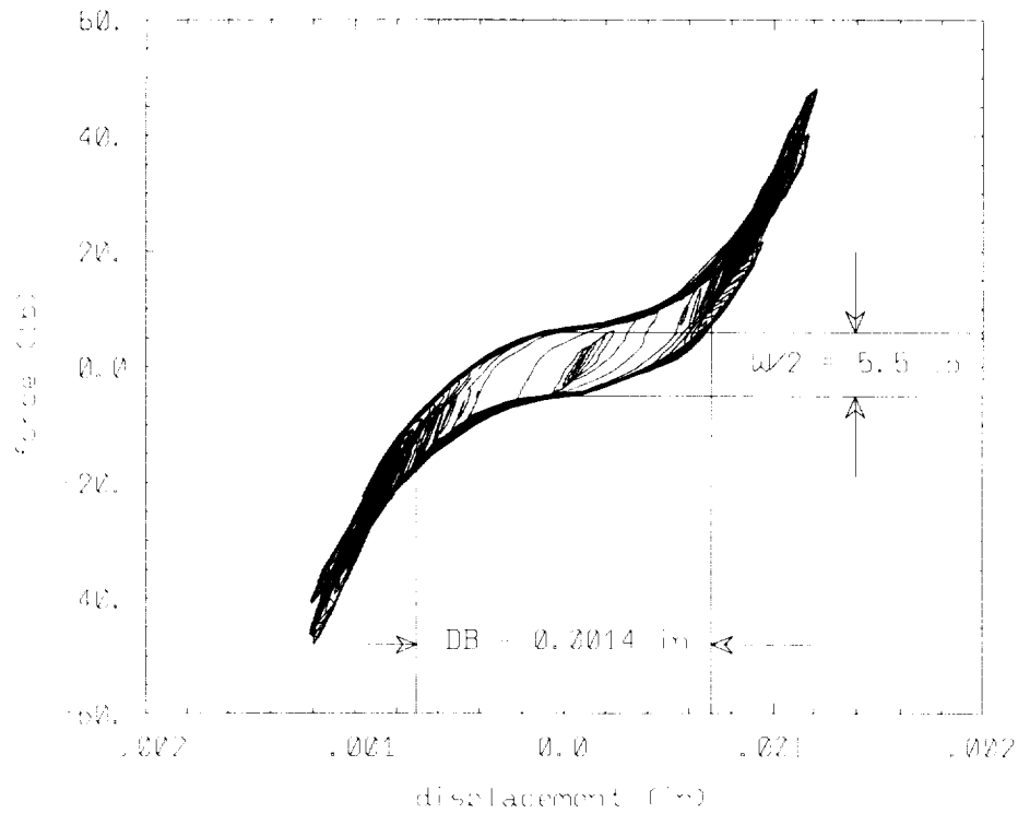
Fig. 62. Illustration of the determination of deadband parameters from dynamic test data for the finite element model.
