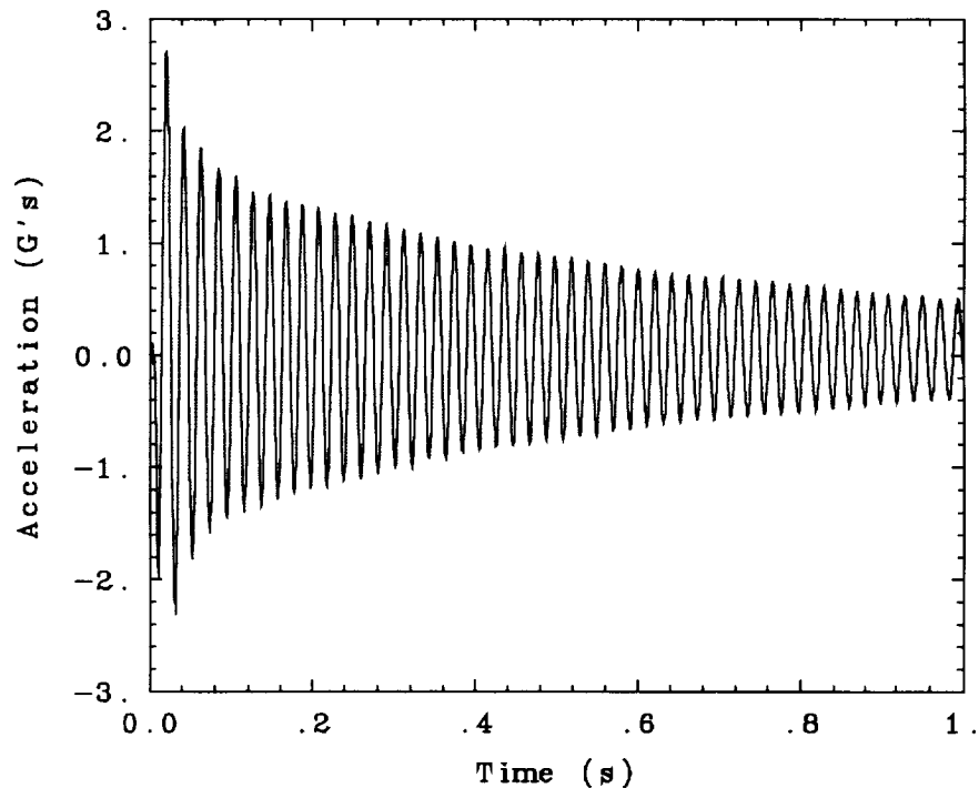
Fig. 24. Bend 1 mode twang test in the 0^\circ truss orientation with all joints locked.
