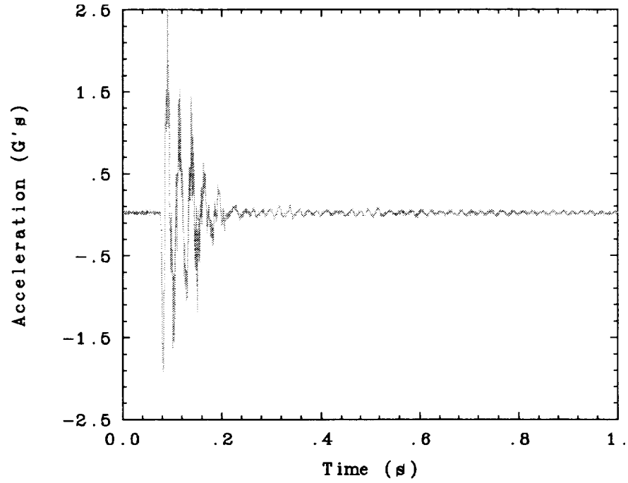
Fig. 97. Bend 2 twang test recorded on the GAS bridge during space shuttle integration.
