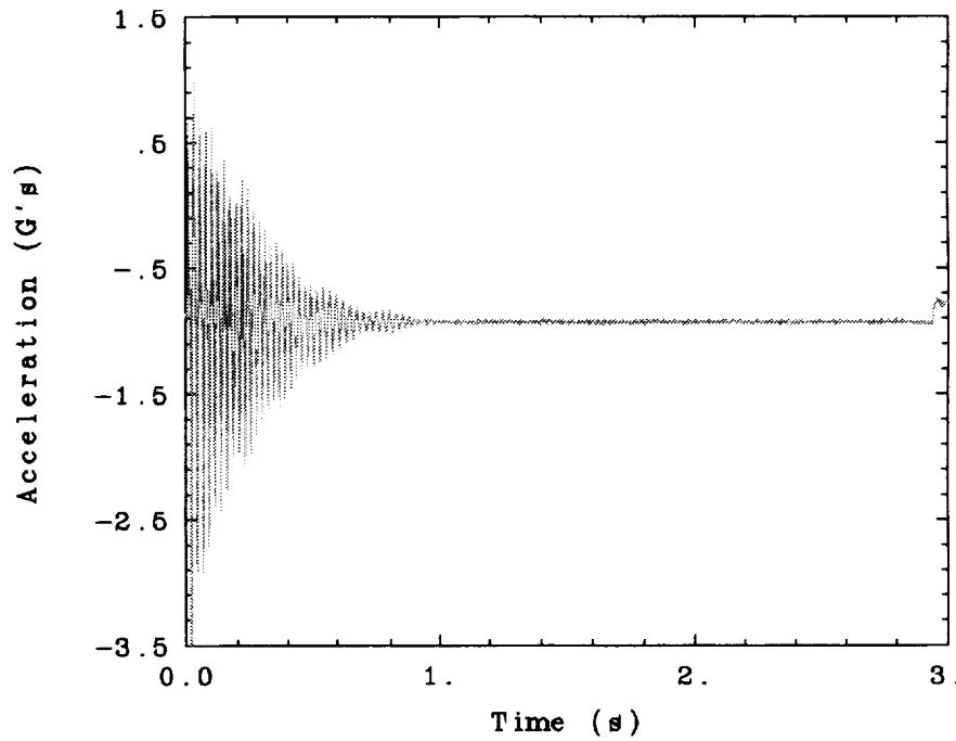
Fig. 90. Bend 2 twang test using pin set two in the 90° truss orientation.
