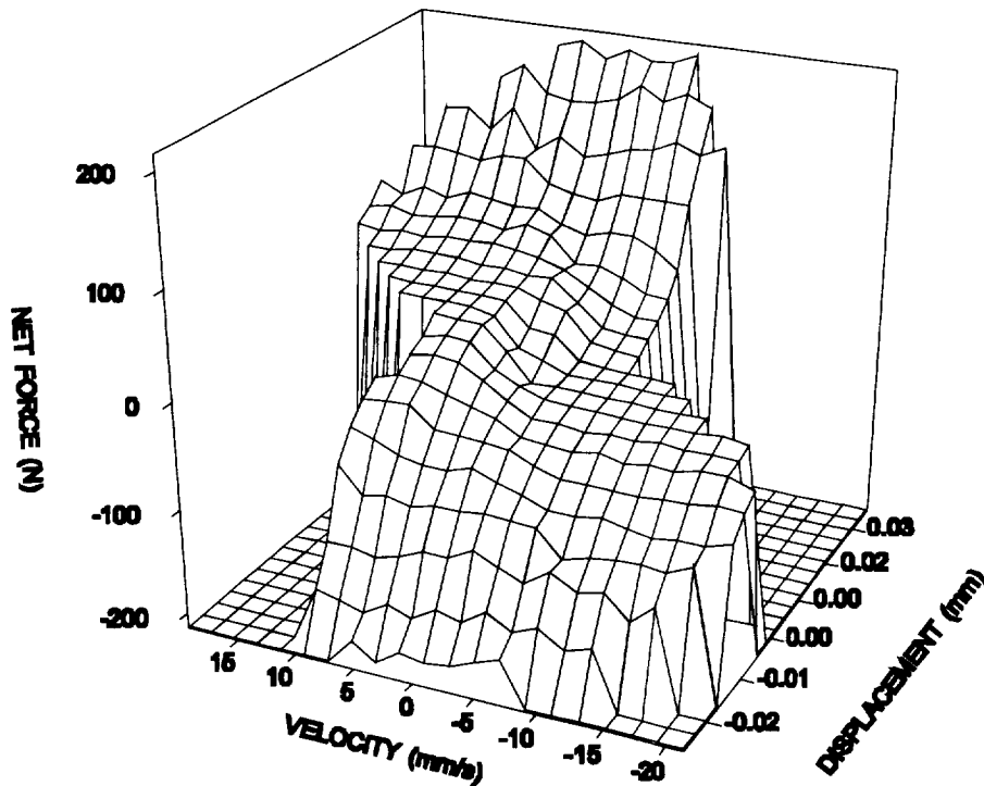
Fig. 59. Force state map of measured data for the short strut with a 0.1862 inch pin and a 35 Hz. forcing frequency.
