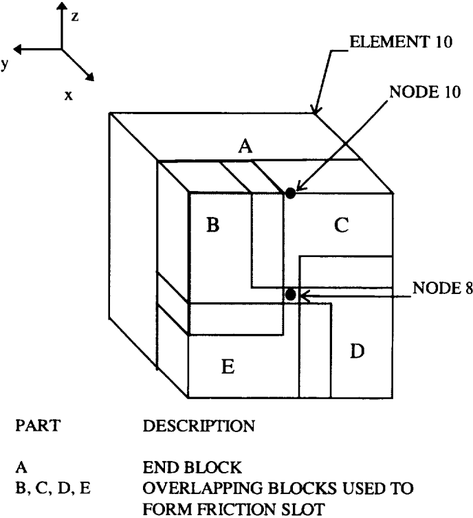
Fig. 65. Three-dimensional view of the unlocked joint model.
