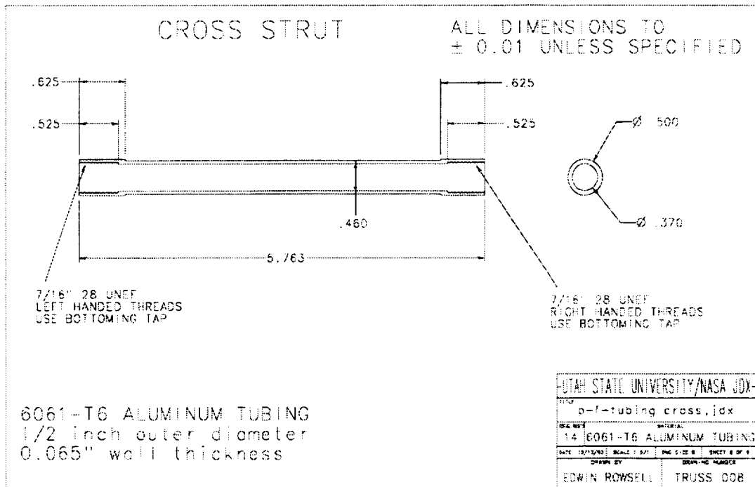
Fig. 84. JDX long tube design
