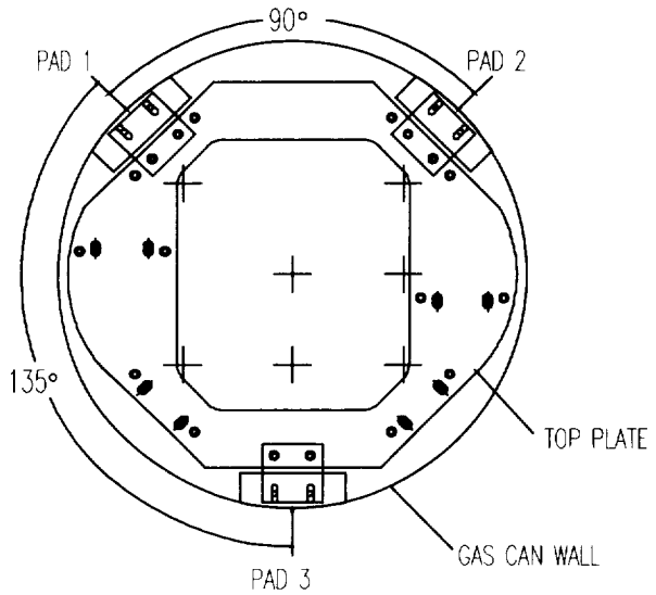
Fig. 3. Illustration of the bumper pads.
