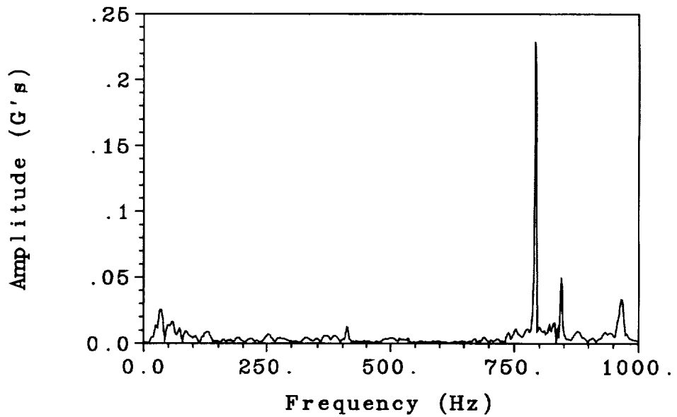
Fig. 40. FFT of a torsion mode free float twang test of the Flight Model truss conducted during a low-G aircraft flight.
