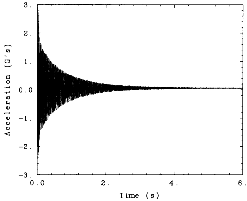
Fig. 18. Bend 1 mode twang test with all joints locked, 0° truss orientation.
