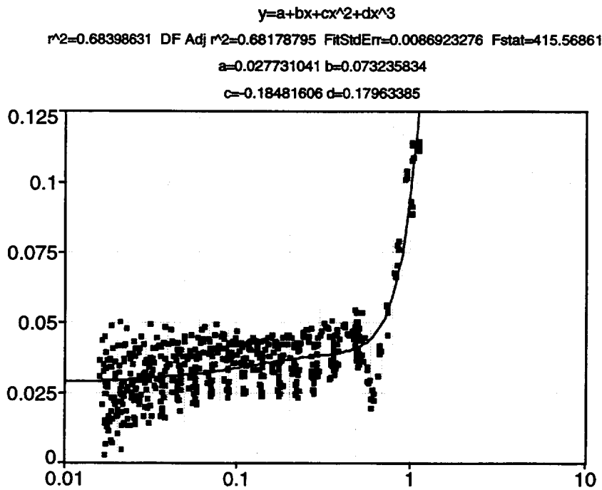
Fig. 120. Bend 1 test, upper peaks, in the 90° truss orientation using pin set three.
