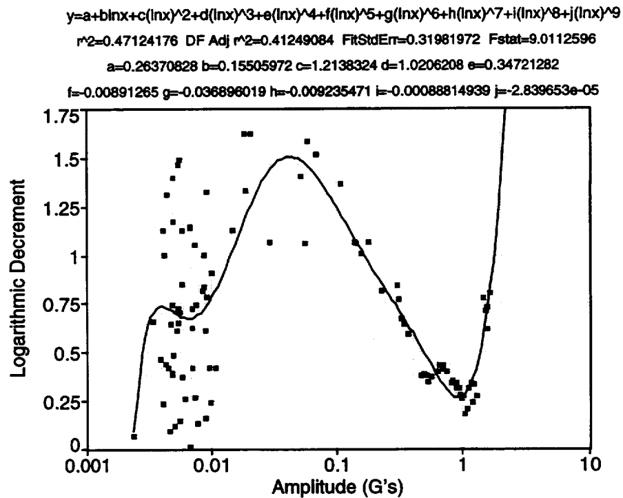
Fig. 131. Bend 1 test during the Space Shuttle flight.
