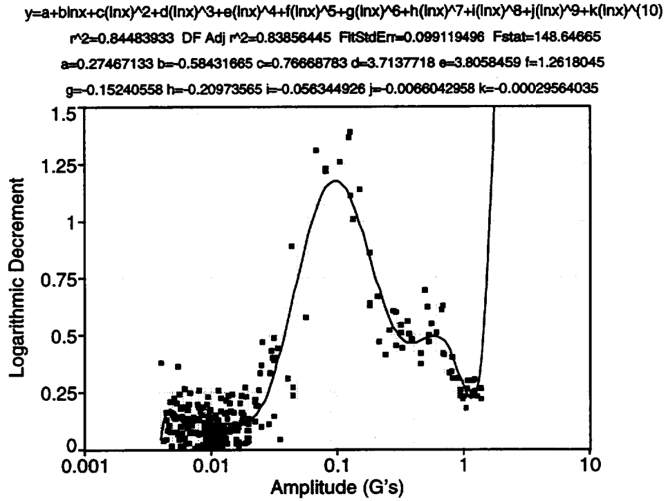
Fig. 138. Baseline bend 2 test in the 180° truss orientation.
