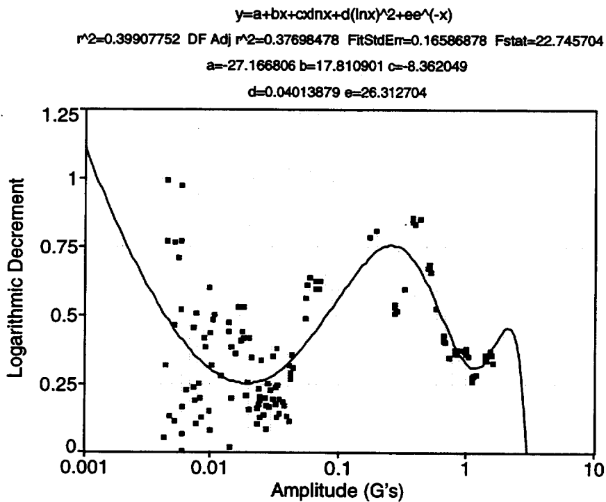
Fig. 129. Cold cell bend 1 test at -20^{\circ} C.
