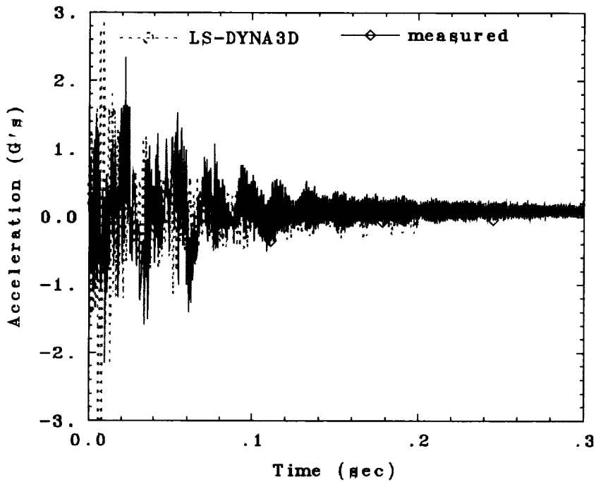
Fig. 76. Torsion test acceleration for an unlocked truss in micro gravity.
