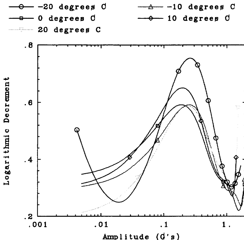
Fig. 30. Logarithmic decrement curves for the Bend 1 mode cold cell twang tests.
