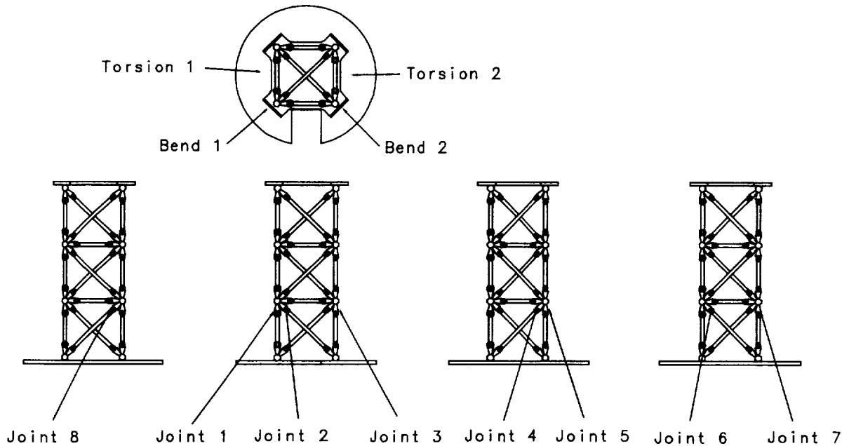
Fig. 22. Illustration of the pinned joint locations and identification numbers.
