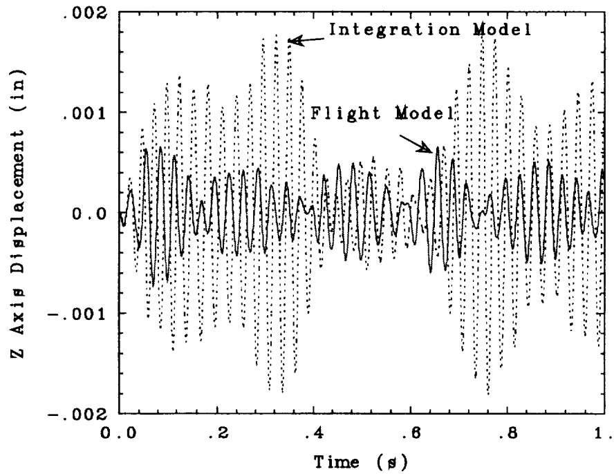
Fig. 44. Predicted Z displacements of the base plate during a bend 1 mode twang test.
