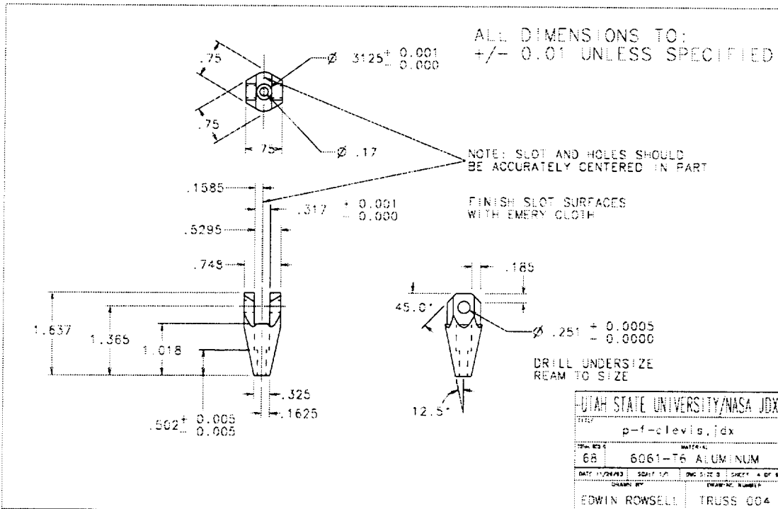
Fig. 81. JDX clevis design.
