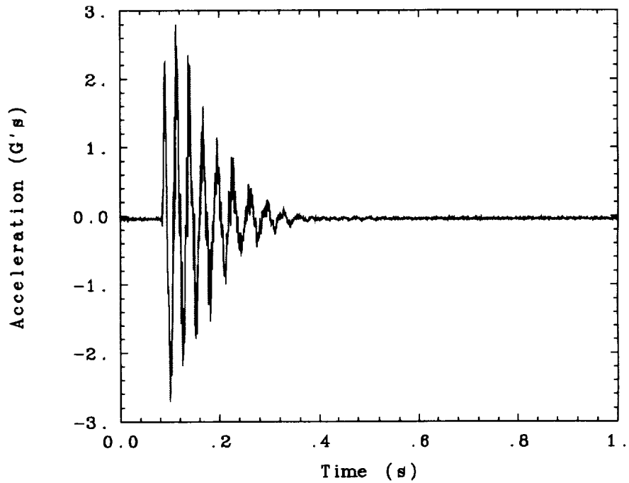
Fig. 110. Bend 1 twang test recorded during cold cell tests at -10° C.
