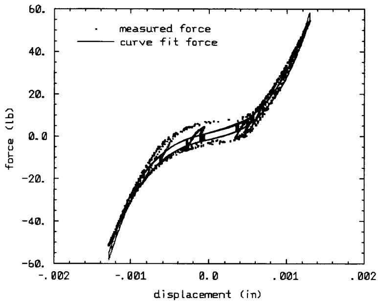
Fig. 57. Plot showing the data for a short strut with a 0.1862 inch pin and 1 Hz. forcing frequency compared to the curve fit given by Eq. 3.
