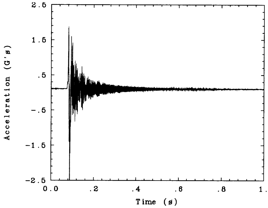
Fig. 103. Baseline torsion twang test in the 180° truss orientation.
