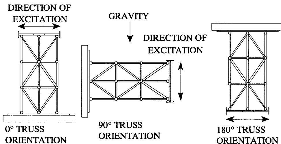
Fig. 15. Illustrations of the truss orientations used for ground tests.
