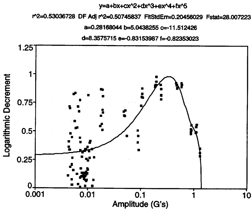
Fig. 141. Cold cell bend 2 test at 0° C.
