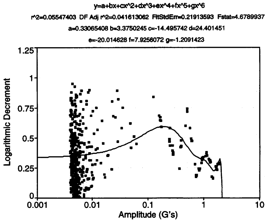
Fig. 127. Cold cell bend 1 test at 0° C.
