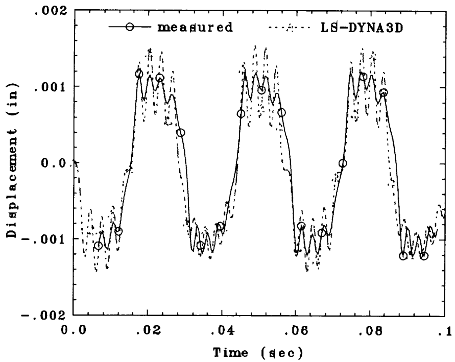
Fig. 68. Measured and predicted time-displacement curves.
