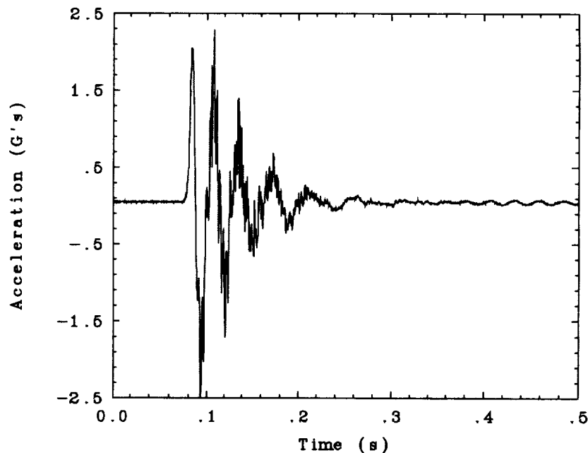
Fig. 43. Bend 1 mode twang test conducted during Space Shuttle integration.
