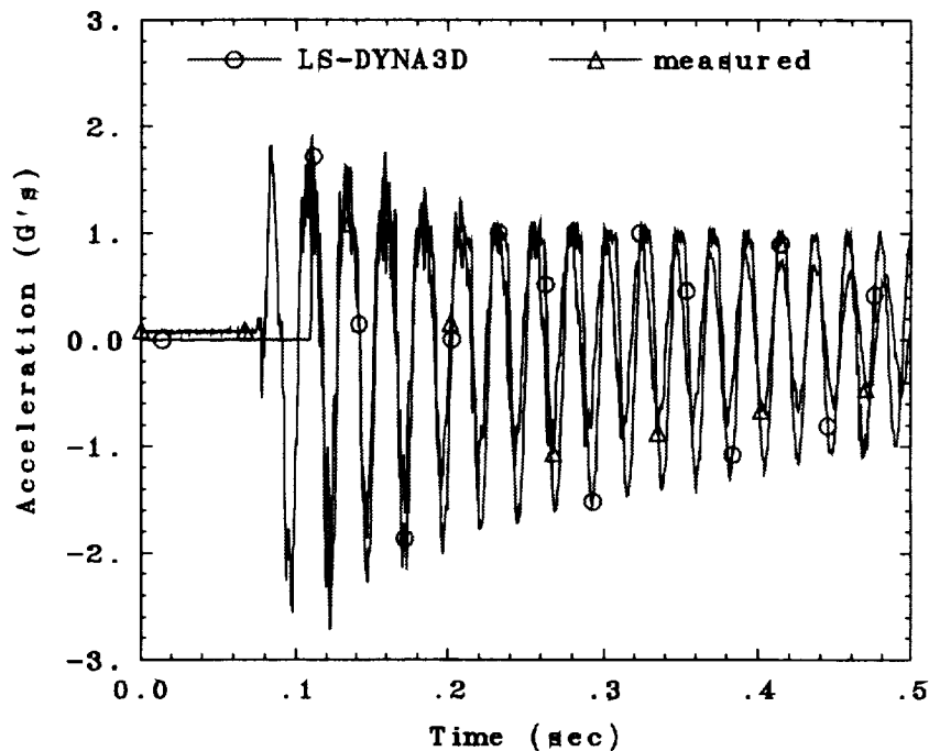
Fig. 74. Bend 1 acceleration for an unlocked truss in 90° truss orientation.
