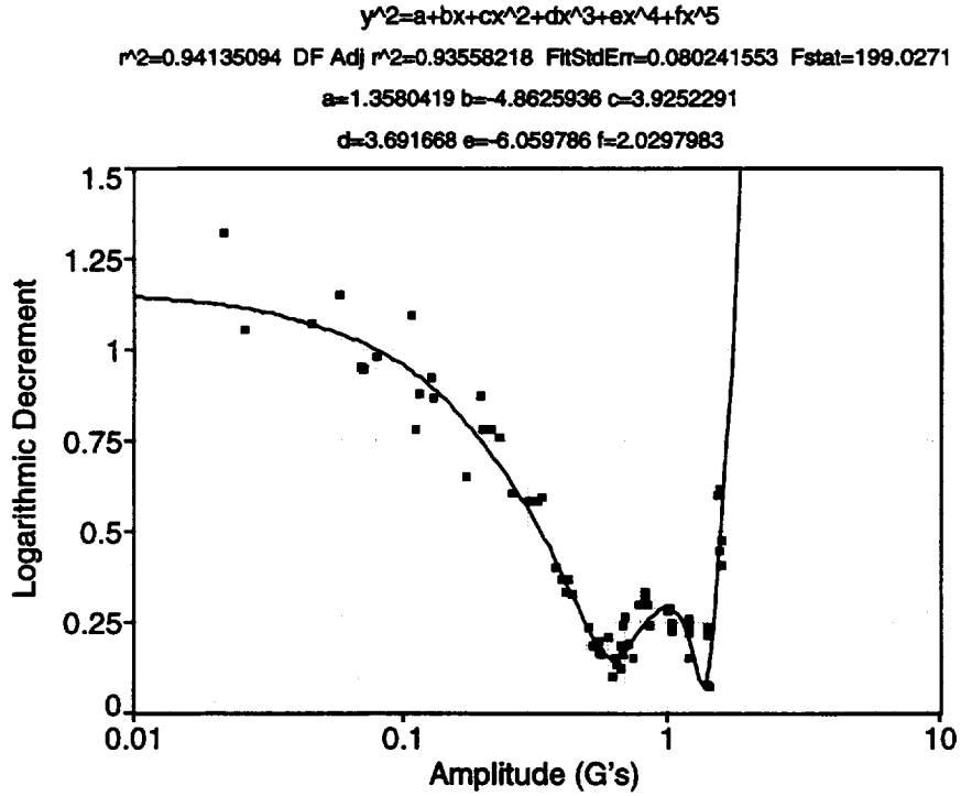
Fig. 146. Bend 2 post flight test in the 0° truss orientation.
