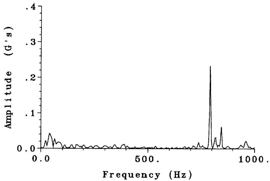
Fig. 79. Measured torsion test frequencies for unlocked truss in micro gravity.
