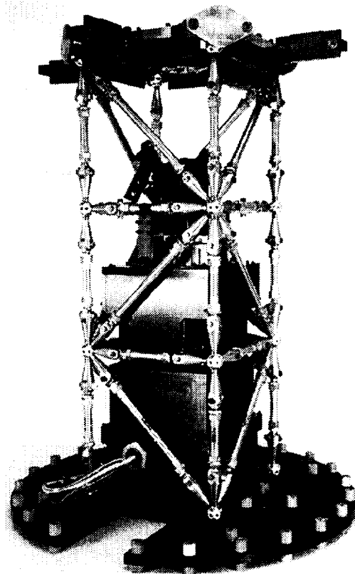
Fig. 4. Photograph showing the items located inside the truss bays.
