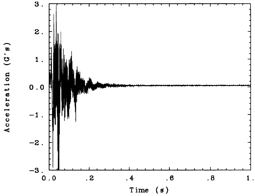
Fig. 101. Torsion twang test using pin set three in the 0° truss orientation.
