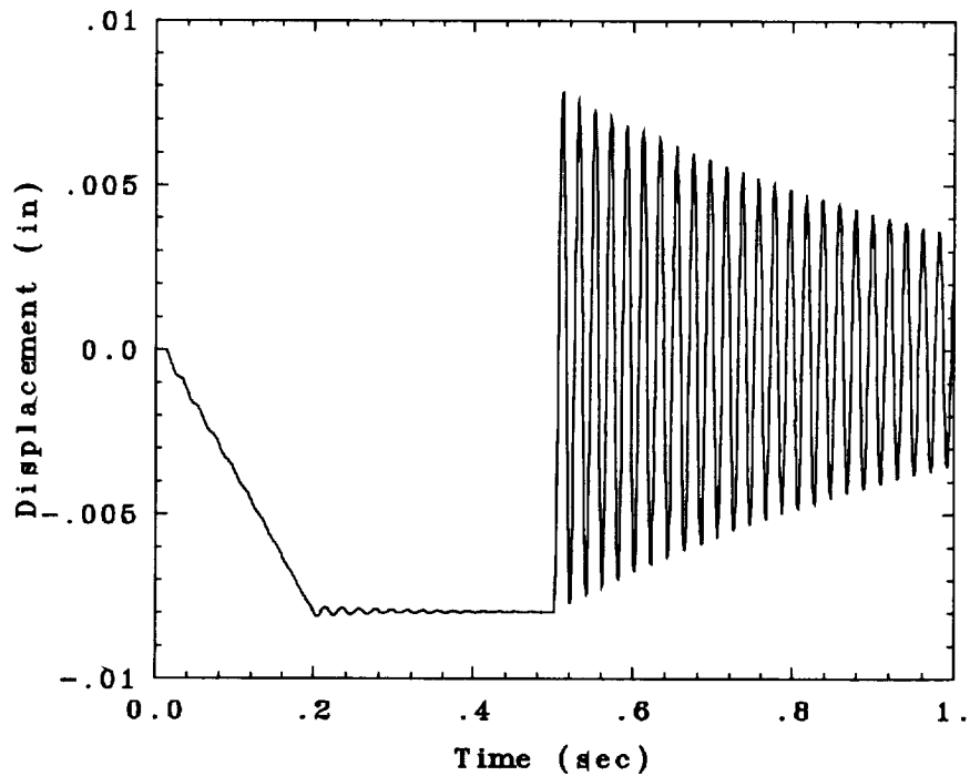
Fig. 70. Bend 1 displacement of tip mass in locked truss model.
