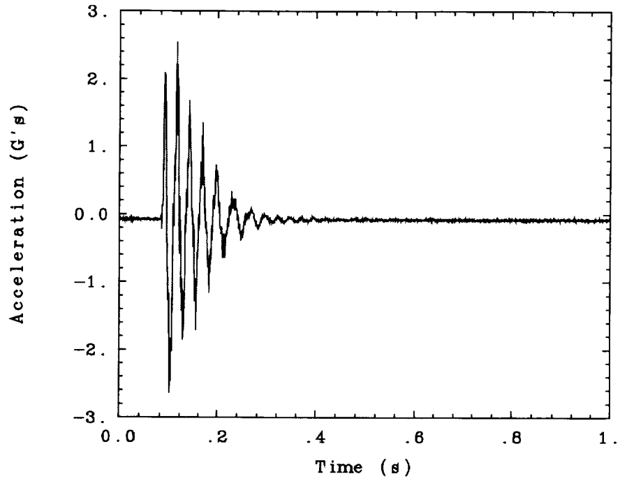
Fig. 111. Bend 1 twang test recorded during cold cell tests at -20° C.
