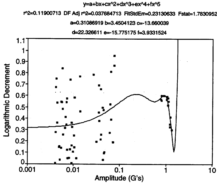
Fig. 140. Cold cell bend 2 test at 10° C.
