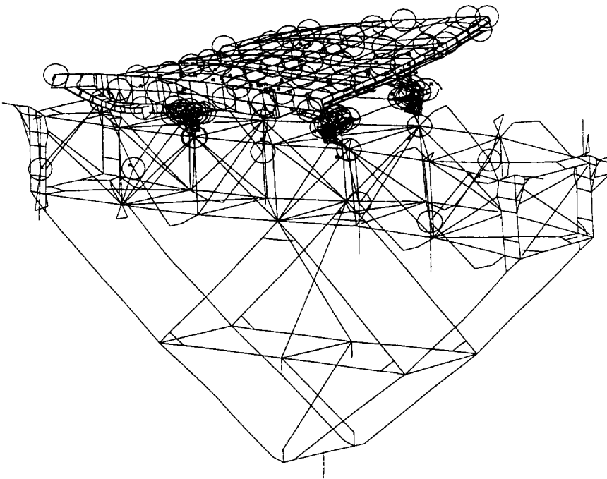
Fig. 46. Predicted 40 Hz. GAS bridge mode shape.
