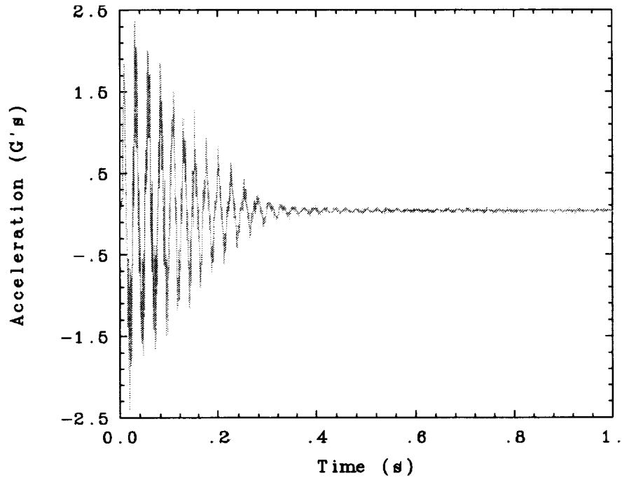
Fig. 89. Bend 2 twang test using pin set two in the 0° truss orientation.
