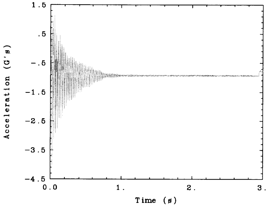
Fig. 92. Bend two twang test using pin set three in the 90° truss orientation.
