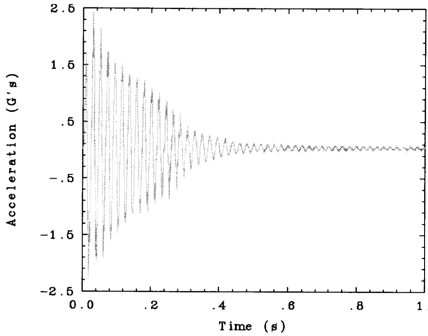
Fig. 87. Bend 2 twang test using pin set one in the 0° truss orientation.
