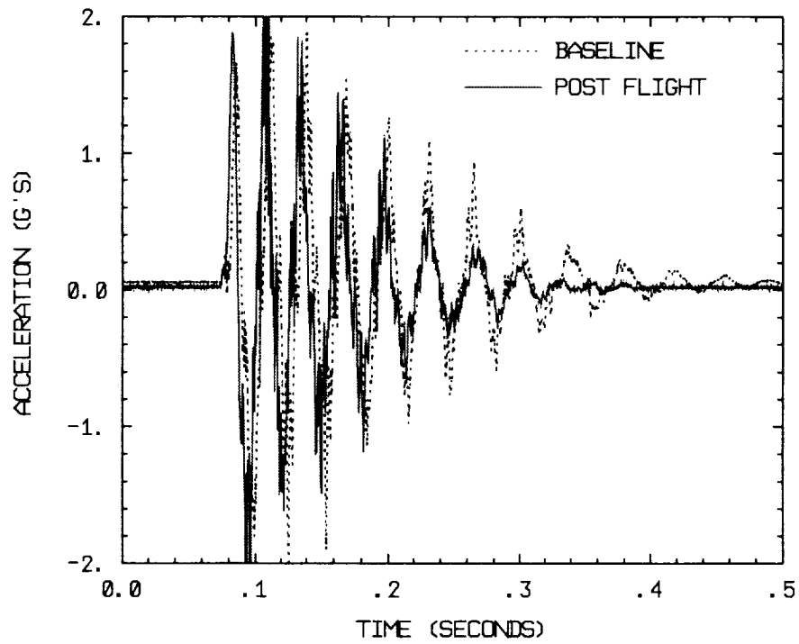
Fig. 51. Comparison of bend 1 mode twang tests from baseline (before flight) and post flight ground tests.
