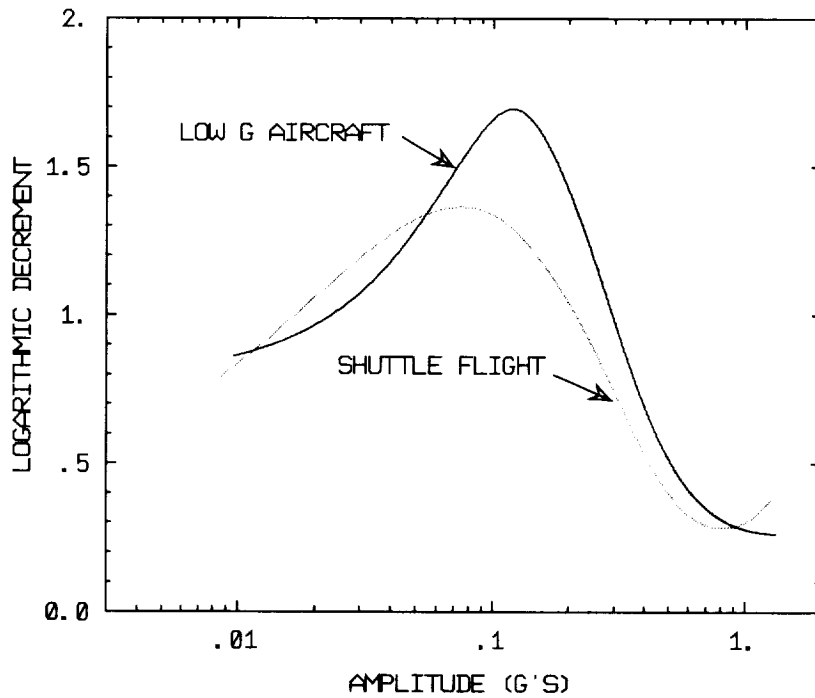
Fig. 50. Comparison of the damping for the bend 1 mode from Shuttle flight and low-G tests.
