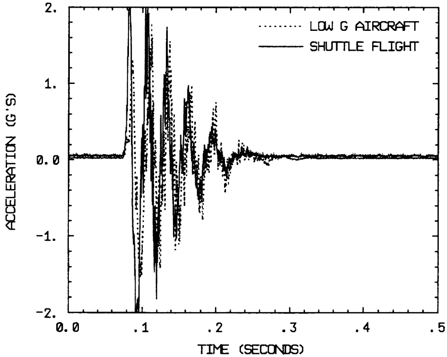
Fig. 48. Comparison of bend 1 mode twang tests from Shuttle flight and low-G tests.
