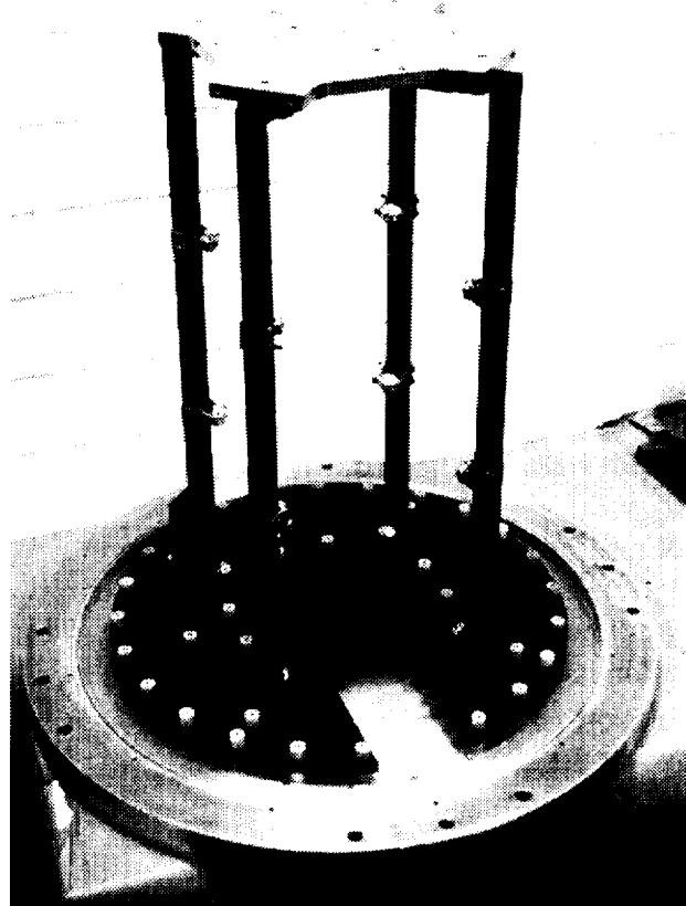
Fig. 12. Photograph of the truss assembly jig.
