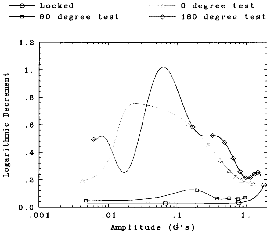
Fig. 28. Logarithmic decrement curves for the Bend 1 mode baseline tests.
