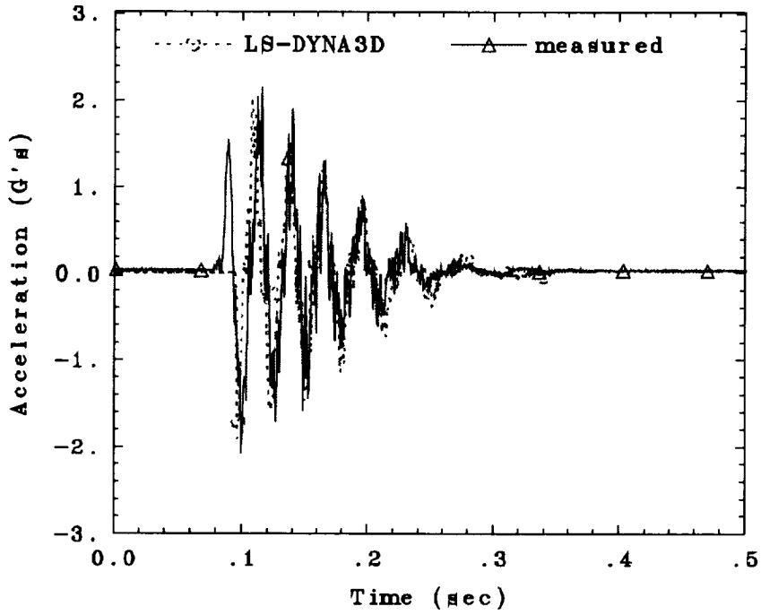
Fig. 72. Bend 1 acceleration for an unlocked truss in micro gravity.
