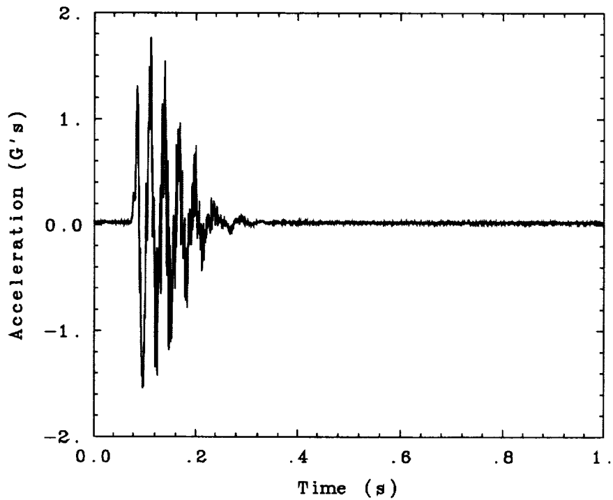
Fig. 33. Bend 1 mode free float twang test conducted aboard the low-G aircraft.
