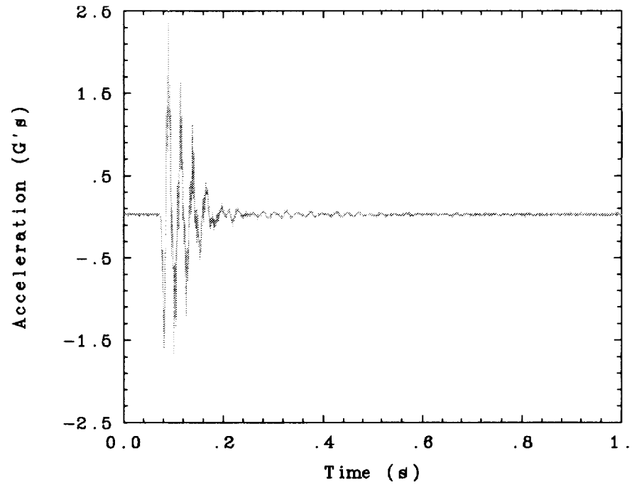
Fig. 98. Bend 2 twang test recorded during Space Shuttle flight.
