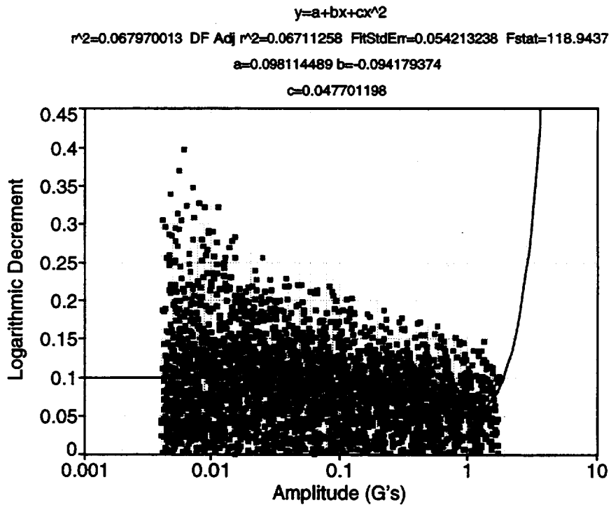
Fig. 147. Torsion test in the 0° truss orientation with all joints locked.
