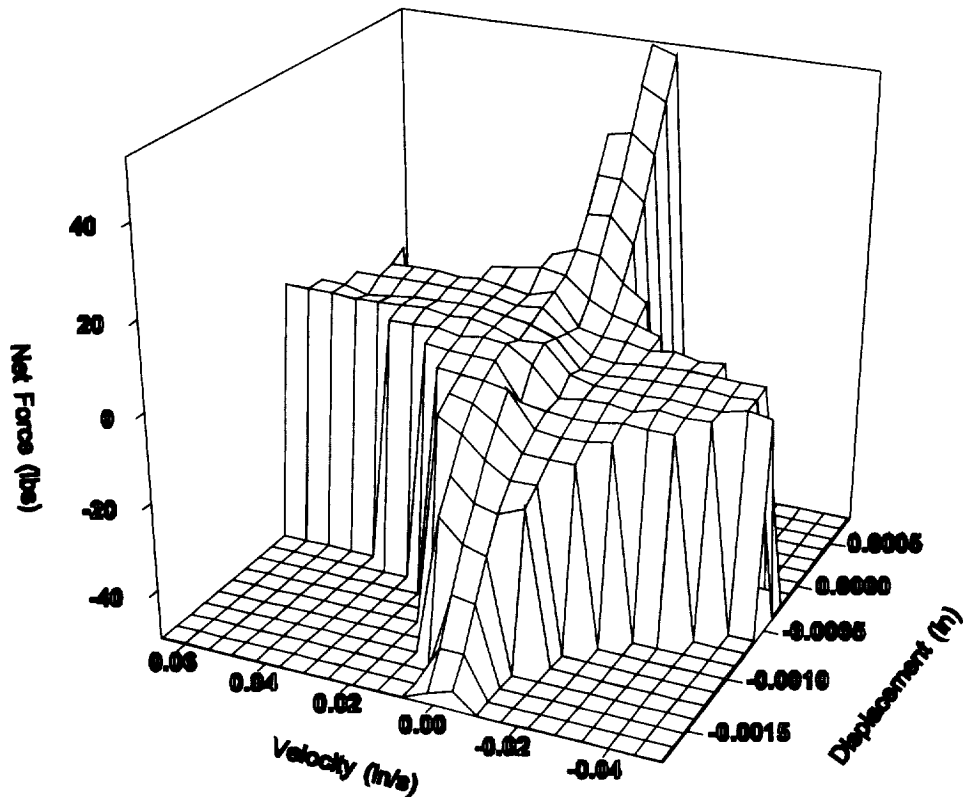
Fig. 55. Force State Map surface for a quasi-static test.
