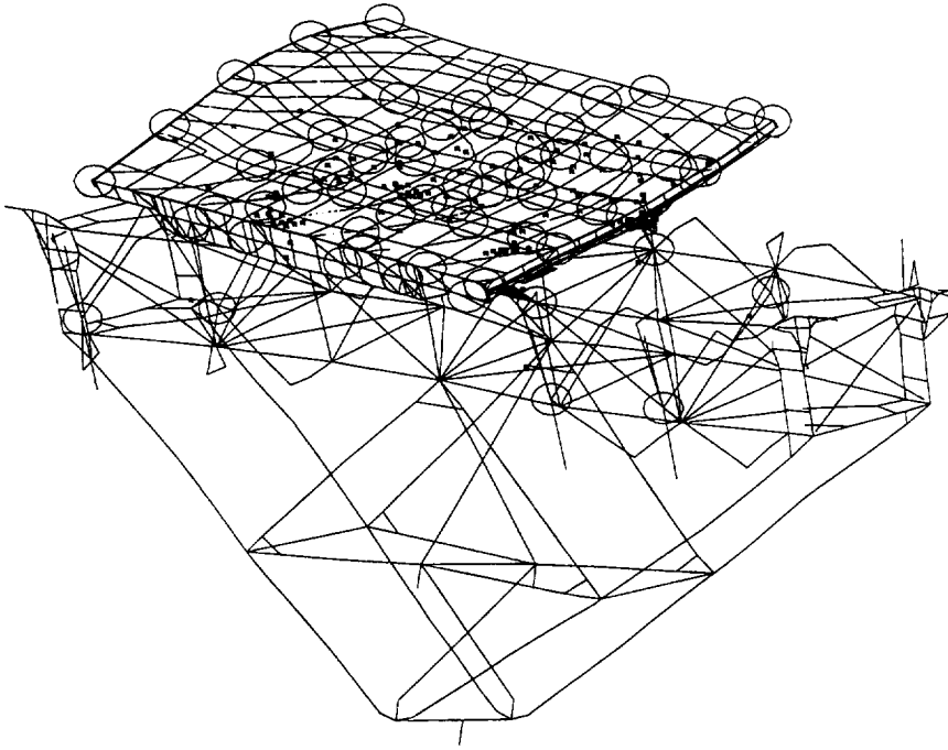
Fig. 45. Predicted 34 Hz. GAS bridge mode shape.
