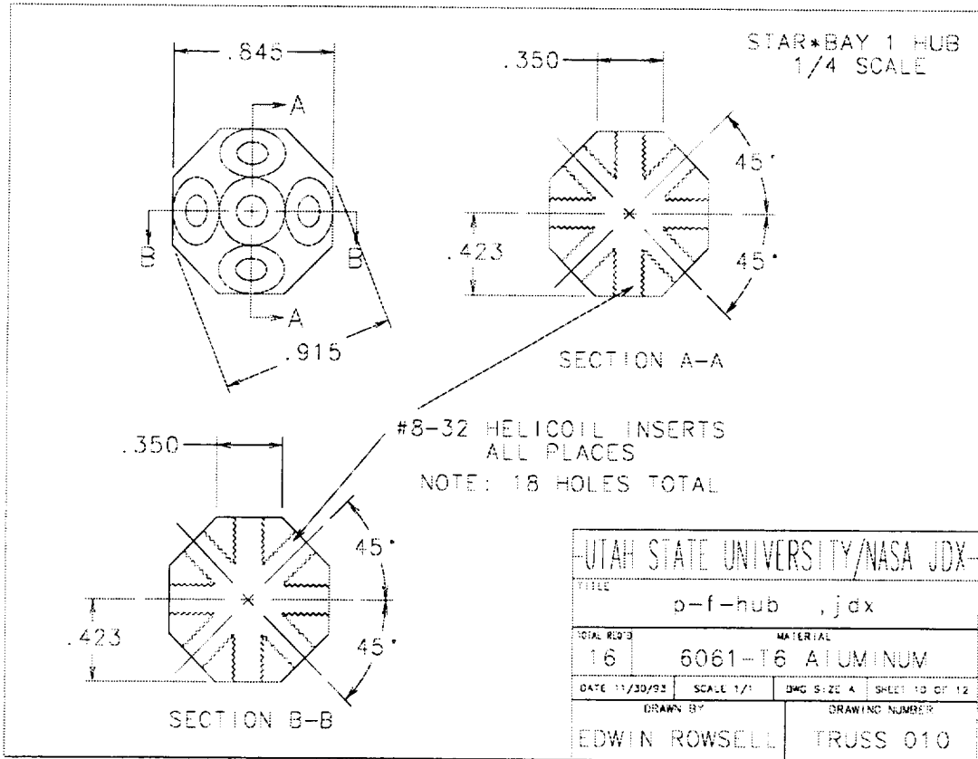
Fig. 85. JDX hub design.
