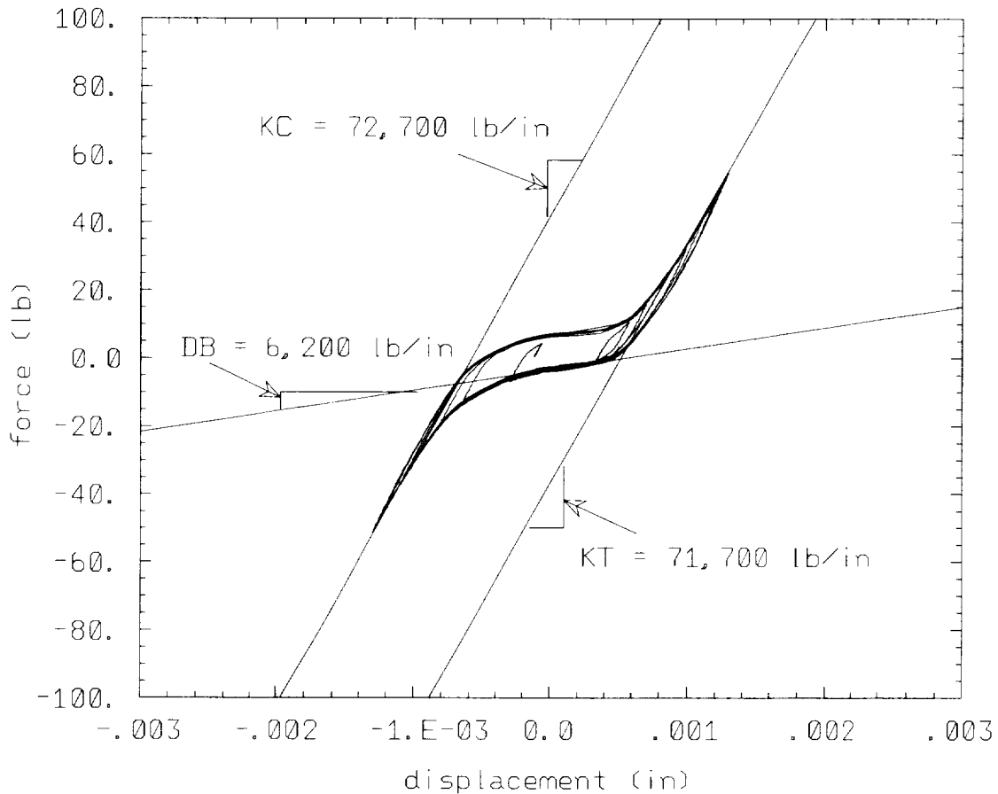
Fig. 61. Illustration of the determination of stiffness from quasi-static test data for the finite element model.
