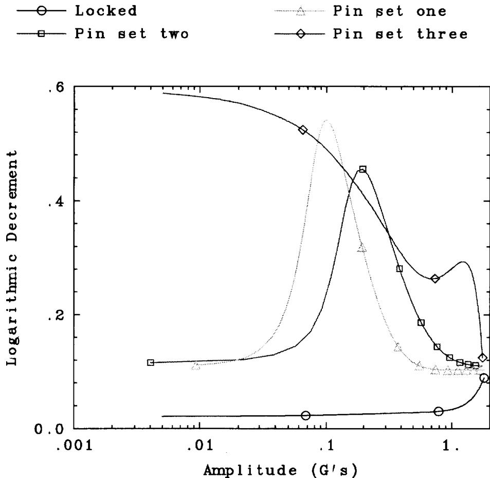
Fig. 23. Logarithmic decrement data from the three pins sets and for a locked truss.
