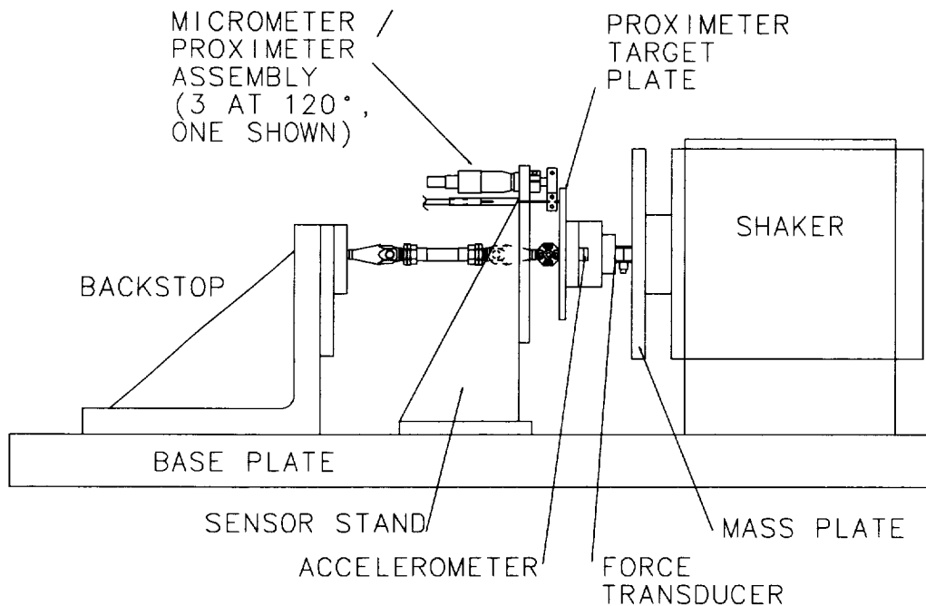
Fig. 53. Illustration of the Force State Map test setup.
