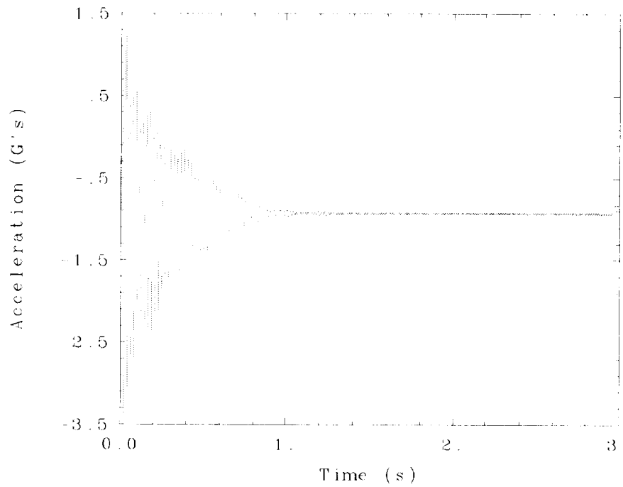
Fig. 88. Bend 2 twang test using pin set one in the 90° truss orientation.
