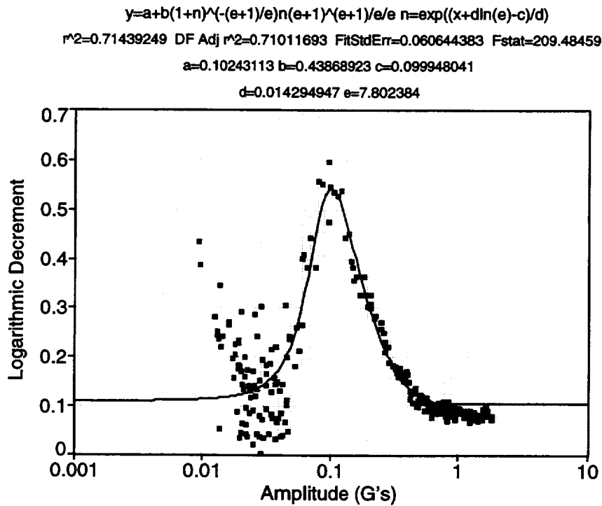
Fig. 113. Bend 1 test using pin set one in the 0° truss orientation.
