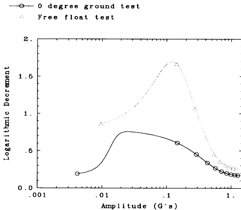
Fig. 34. Logarithmic decrement curves for the bend 1 mode low-G twang tests.
