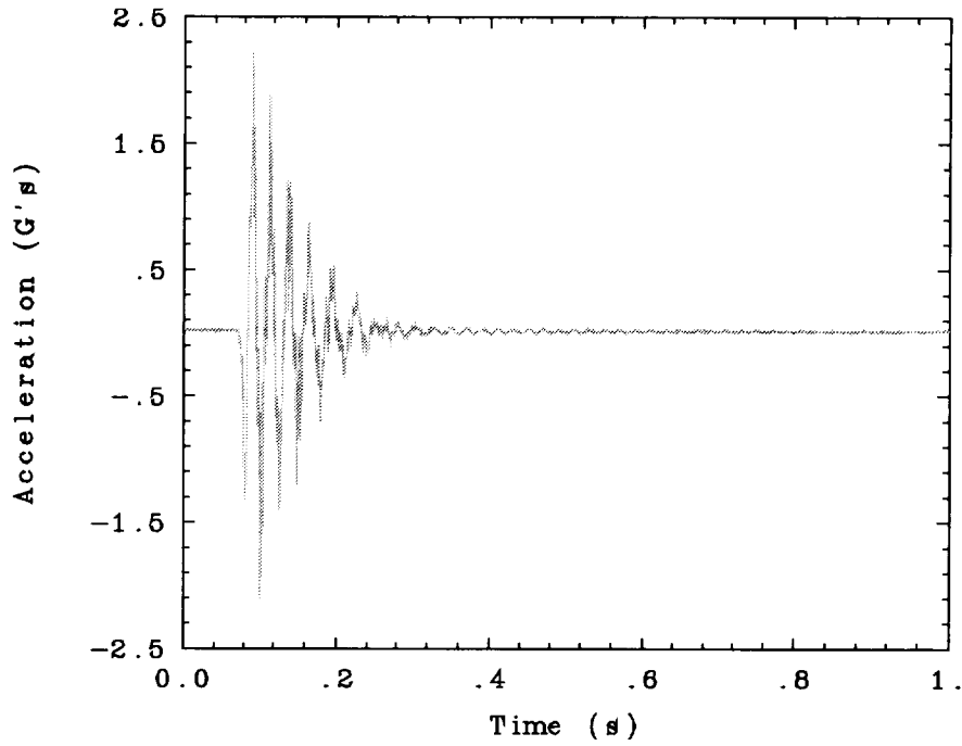
Fig. 95. Baseline bend 2 twang test in the 180° truss orientation.
