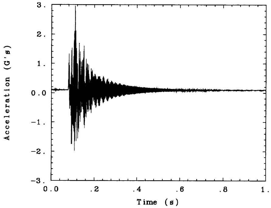
Fig. 104. Torsion twang test recorded during low-G testing.
