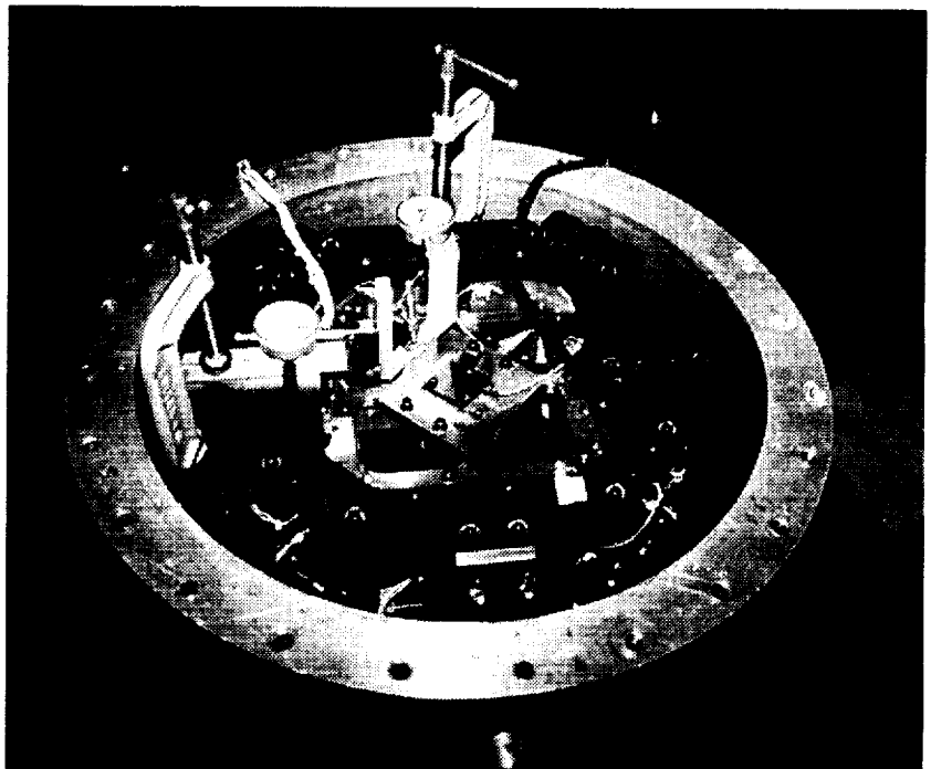
Fig. 14. Photograph showing how movements in the framework were monitored while the lateral support pads were tightened
