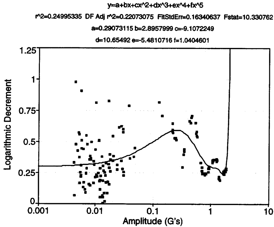
Fig. 128. Cold cell bend 1 test at -10^{\circ} C.
