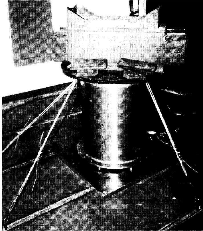
Fig. 17. Photograph of the 180° truss orientation test setup.
