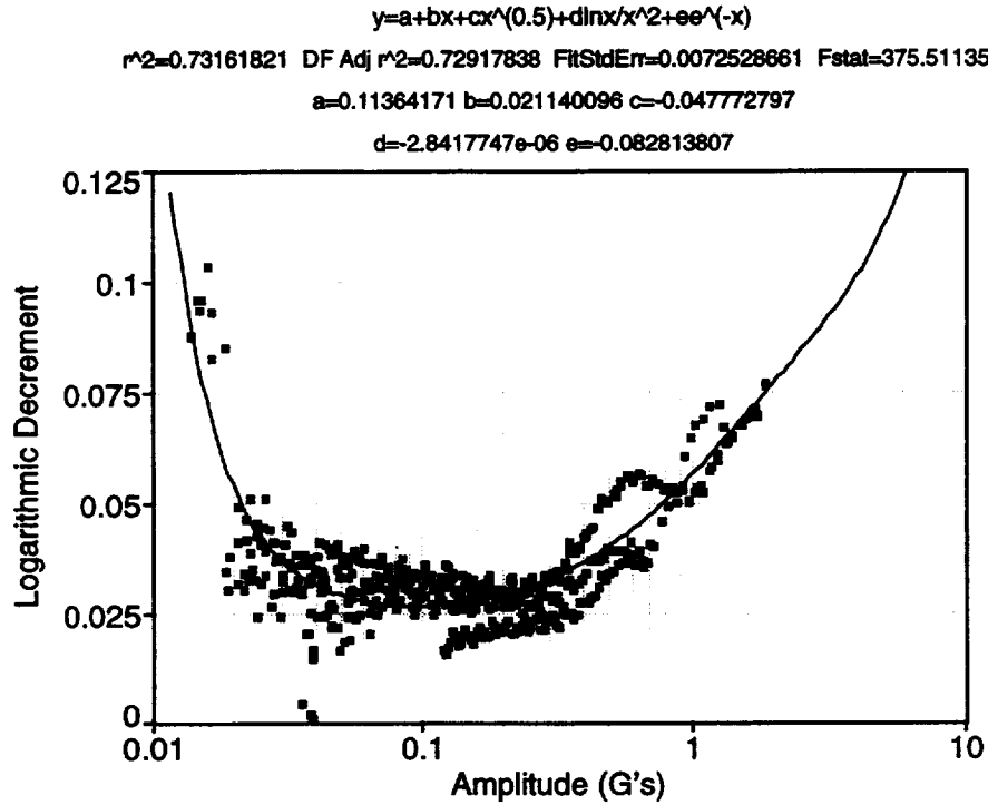
Fig. 118. Bend 1 test, upper peaks, in the 90° truss orientation using pin set two.
