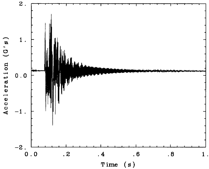
Fig. 37. Torsion mode twang test of the Flight Model truss in a 0° truss orientation.
