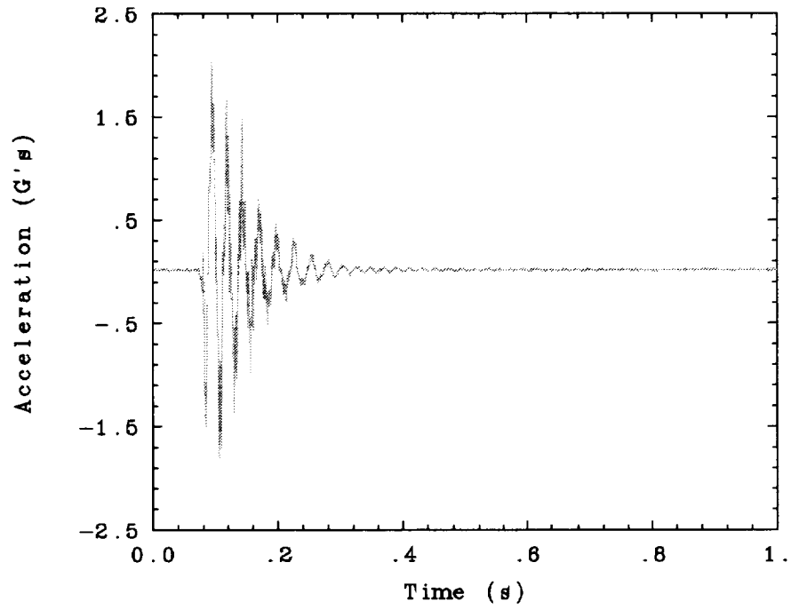
Fig. 93. Baseline bend 2 twang test in the 0° truss orientation.
