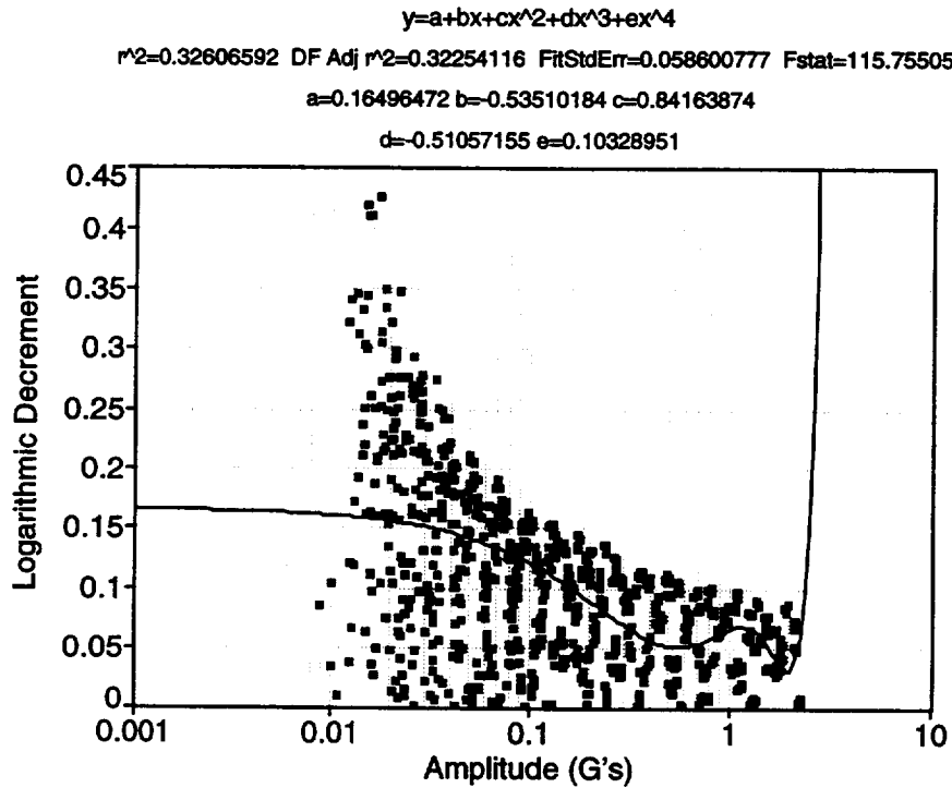
Fig. 148. Baseline torsion test, lower peaks, in the 90° truss orientation.
