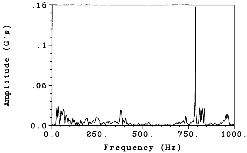
Fig. 38. FFT of a torsion mode twang test of the Flight Model truss in a 0° truss orientation.
