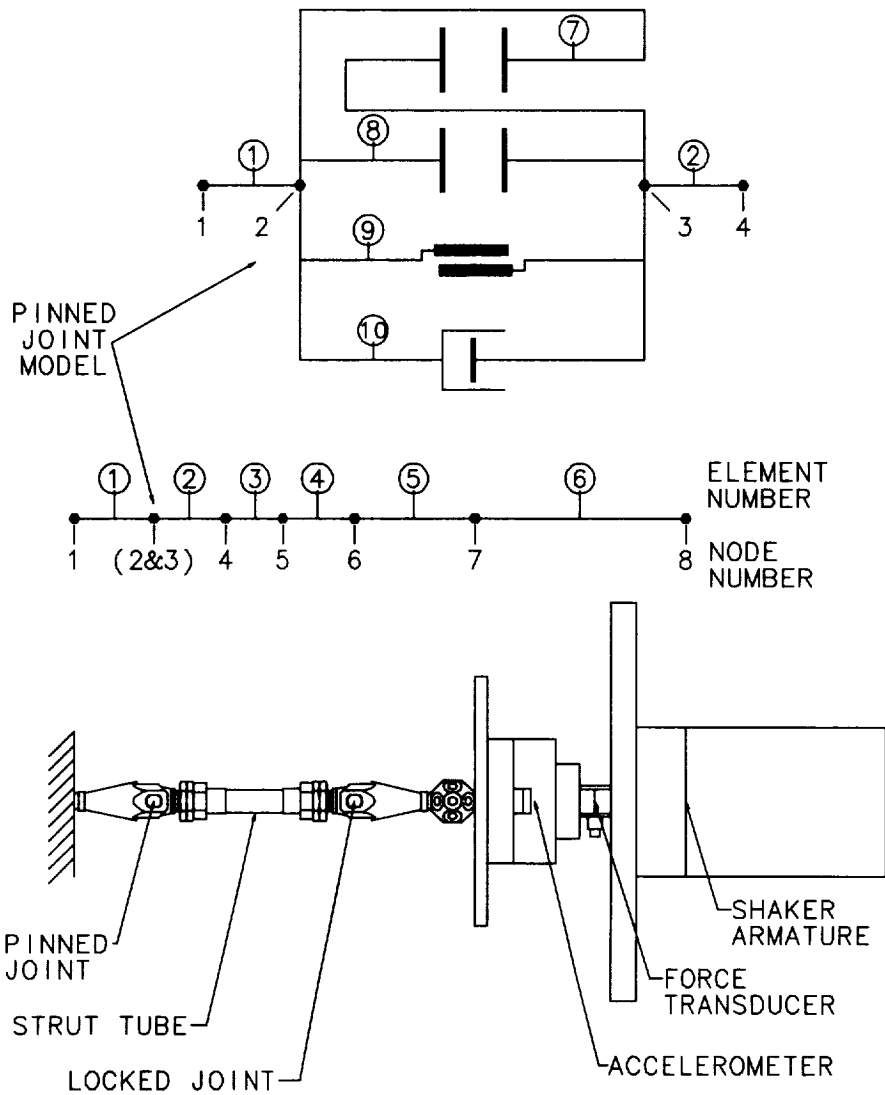
Fig. 60. Illustration of the strut in the test bed and the corresponding finite element model.
