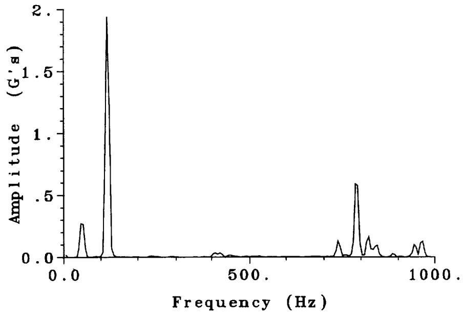
Fig. 77. Measured torsion test frequencies for locked truss in 0° truss orientation.
