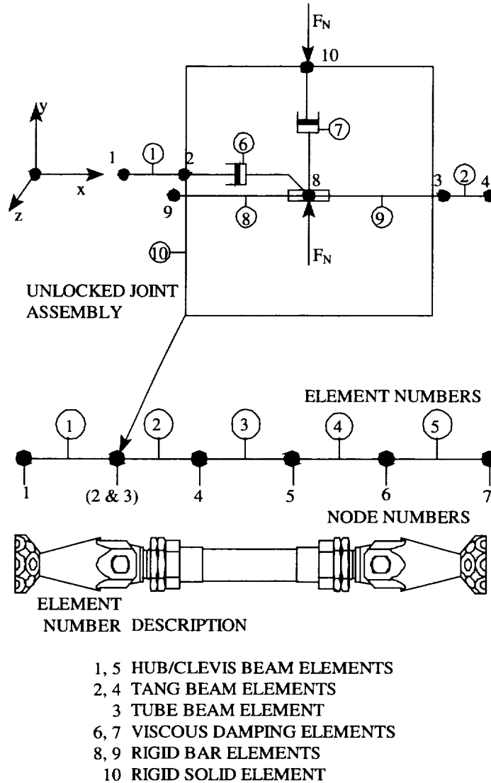
Fig. 64. Finite element model of a strut with an unlocked joint.
