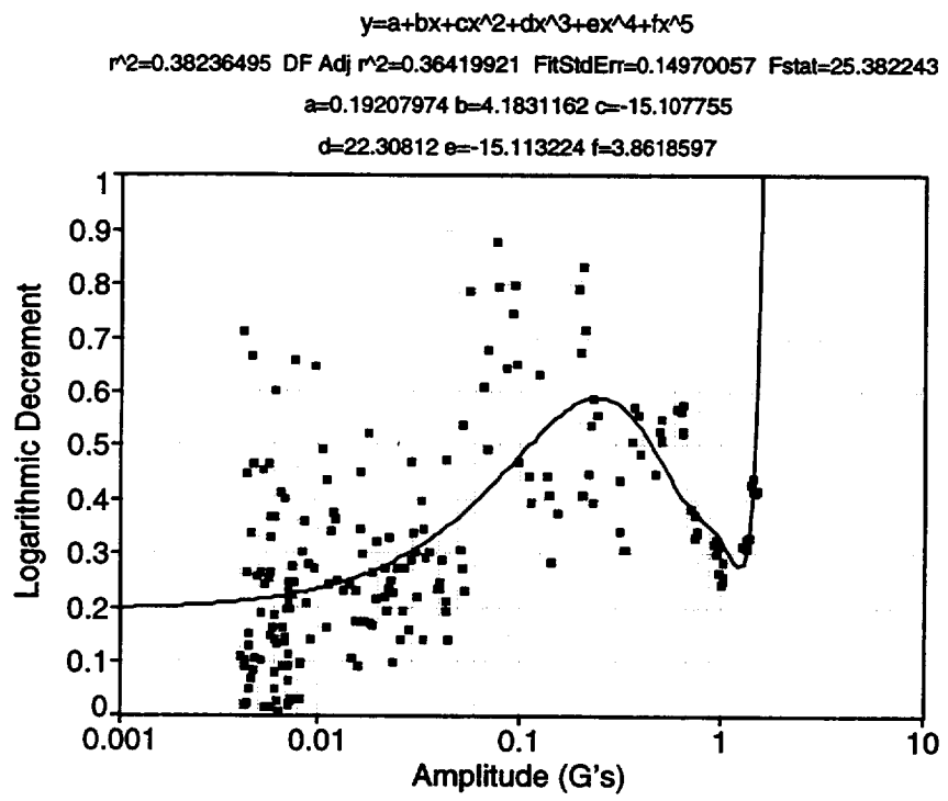
Fig. 125. Cold cell bend 1 test at 20° C.
