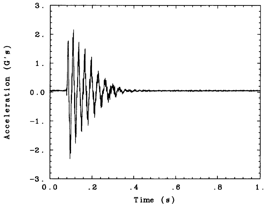
Fig. 27. Bend 1 mode baseline twang test in the 180° truss orientation.
