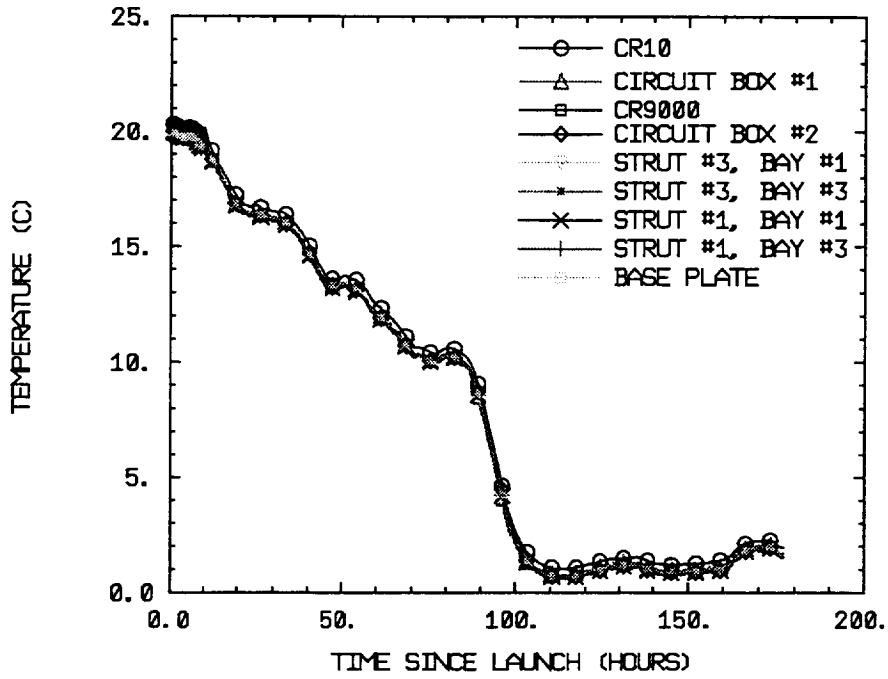
Fig. 47. Illustration of the temperatures recorded during flight.
