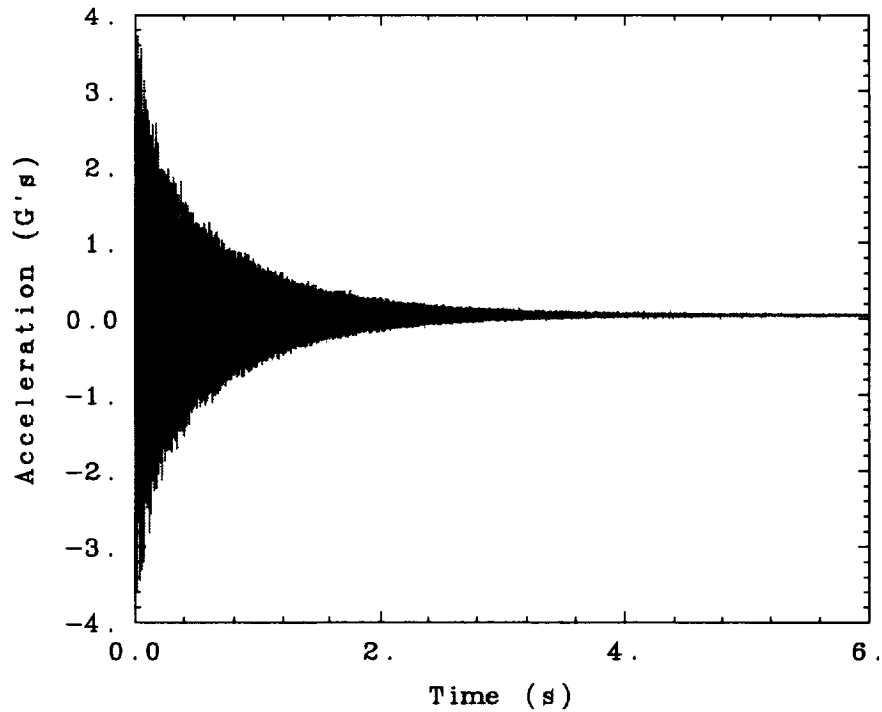
Fig. 35. Torsion mode twang test with all joints locked and a 0° truss orientation.
