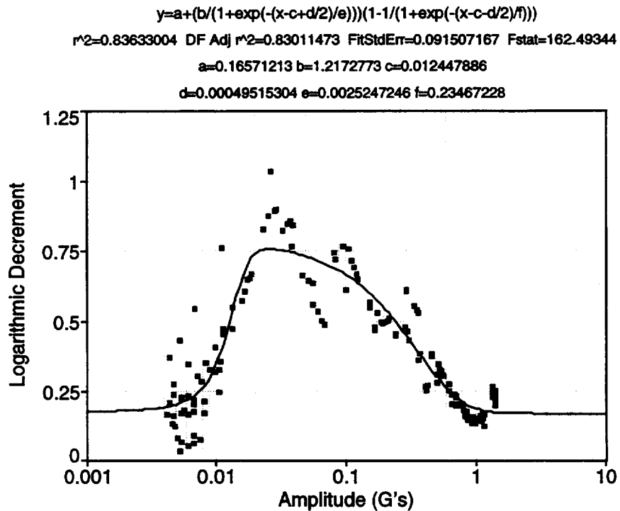
Fig. 115. Baseline bend 1 test in the 0° truss orientation.
