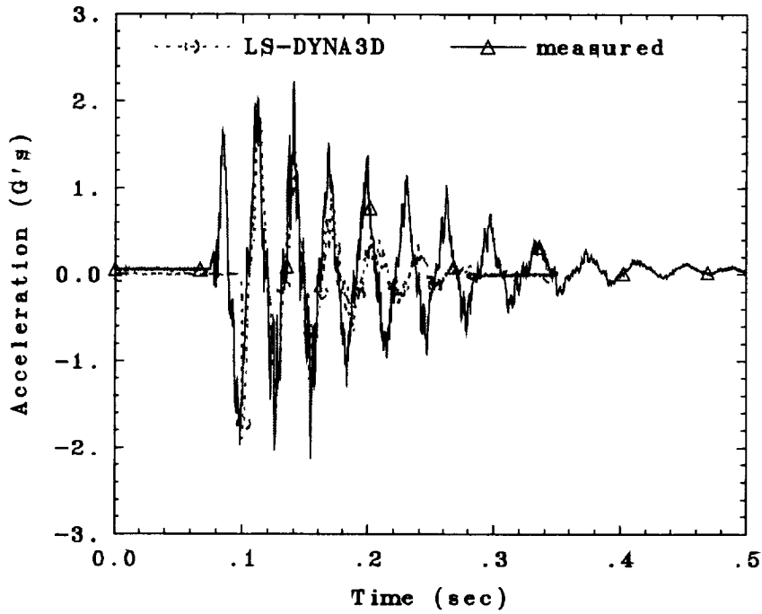
Fig. 73. Bend 1 acceleration for an unlocked truss in 0° truss orientation.
