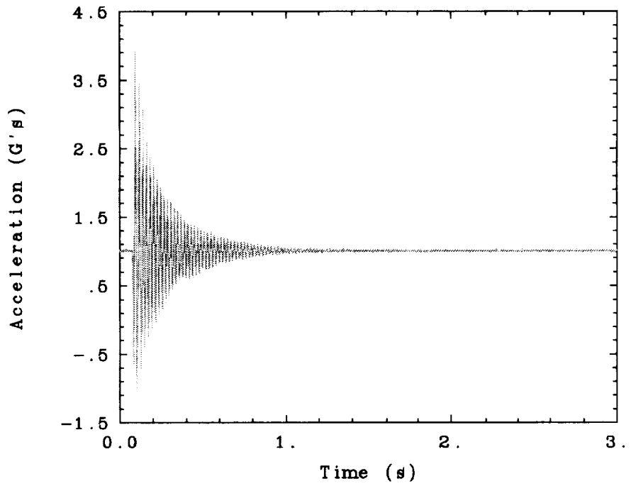
Fig. 94. Baseline bend 2 twang test in the 90° truss orientation.
