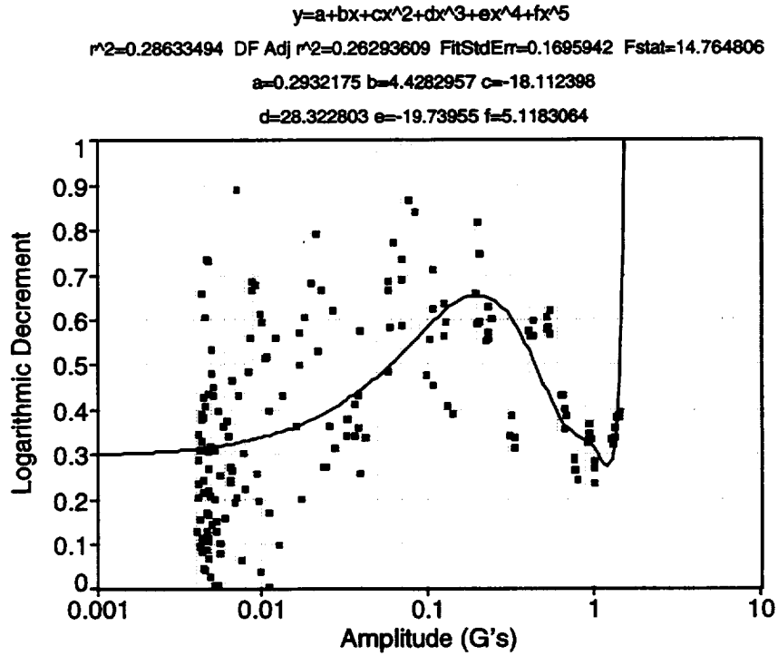
Fig. 126. Cold cell bend 1 test at 10° C.
