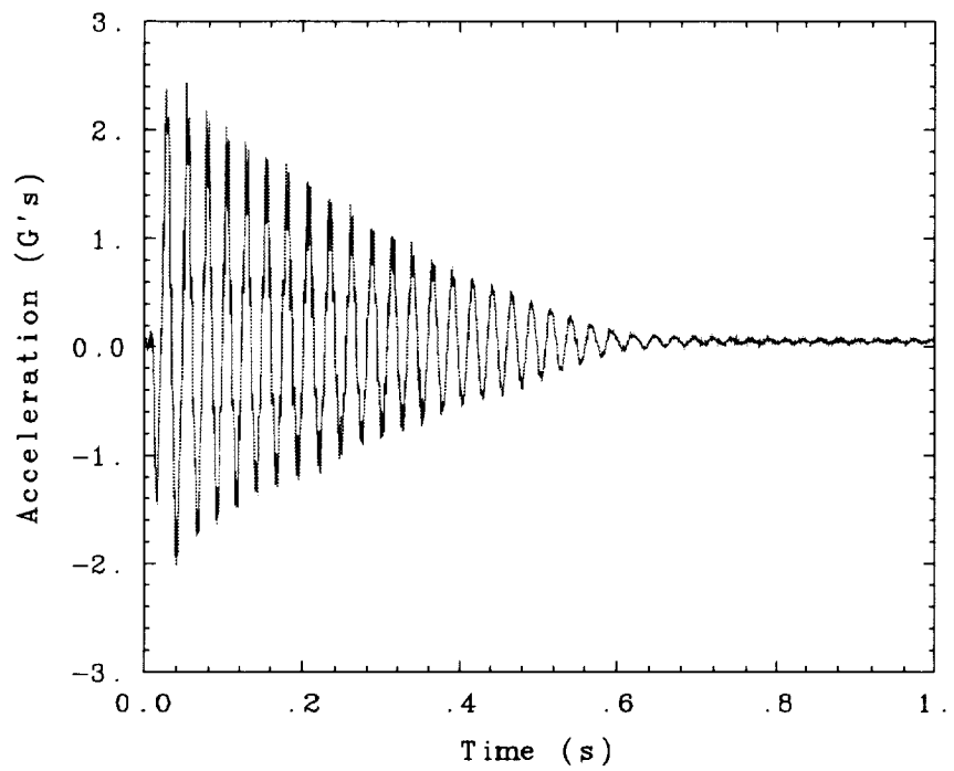
Fig. 19. Bend 1 mode twang test with pin set 1, 0° truss orientation.
