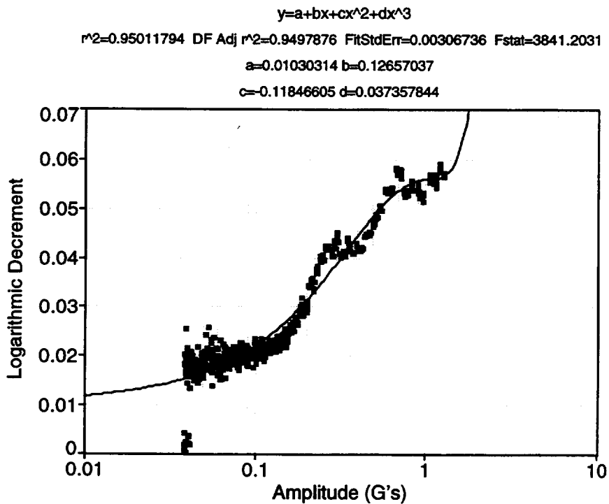
Fig. 117. Bend 1 test, lower peaks, in the 90° truss orientation using pin set one.
