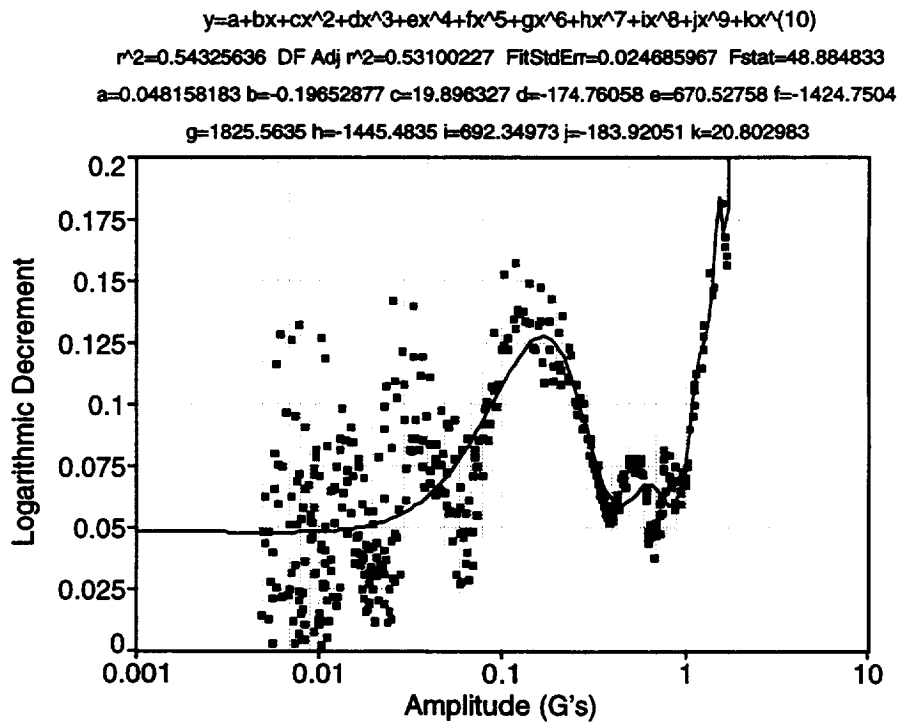
Fig. 123. Baseline bend 1 test, lower peaks, in the 90° truss orientation.
