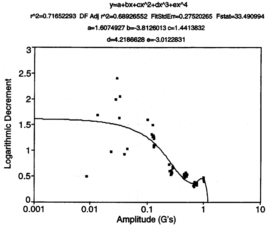
Fig. 144. Bend 2 test during a low-G flight.
