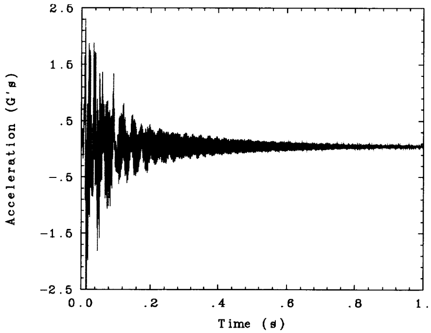
Fig. 100. Torsion twang test using pin set two in the 0° truss orientation.
