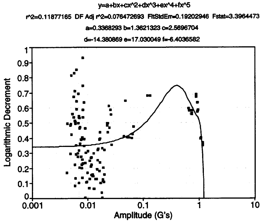
Fig. 142. Cold cell bend 2 test at -10° C.
