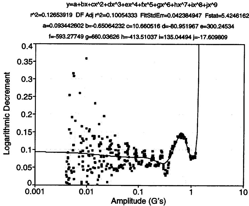
Fig. 136. Baseline bend 2 test, lower peaks, in the 90° truss orientation.
