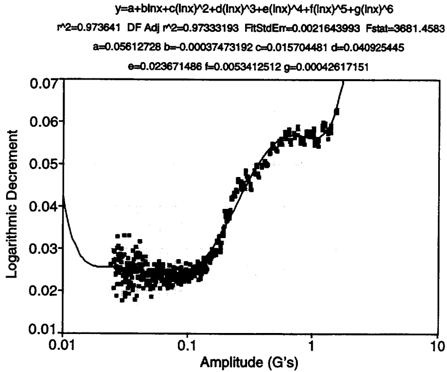
Fig. 116. Bend 1 test, upper peaks, in the 90° orientation using pin set one.
