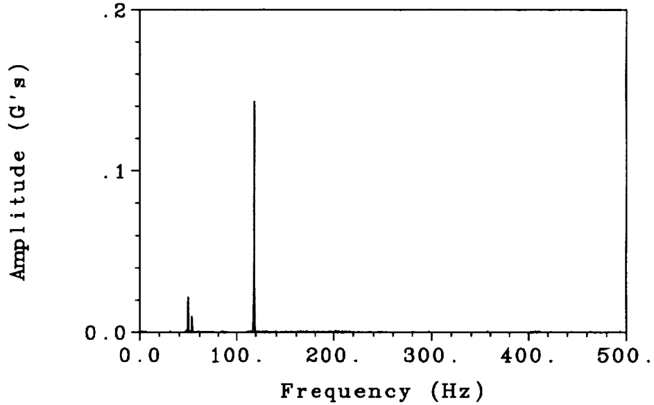
Fig. 36. FFT of a torsion mode twang test with all joints locked and a 0° truss orientation.
