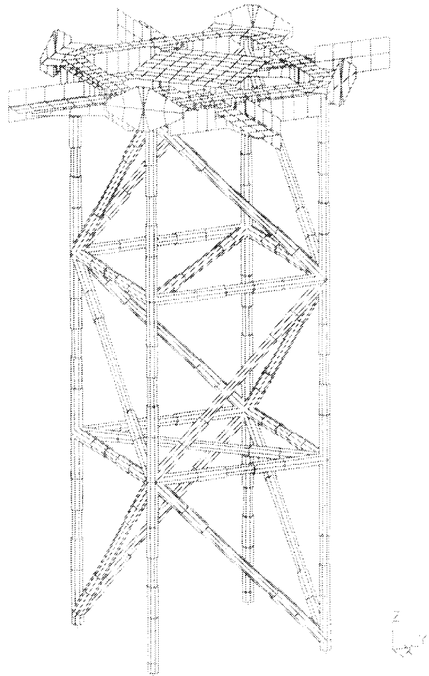
Fig. 69. Illustration of the finite element model of the JDX truss.
