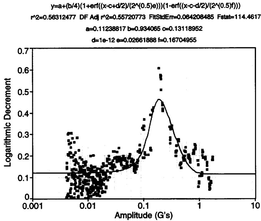
Fig. 114. Bend 1 test using pin set two in the 0° truss orientation.
