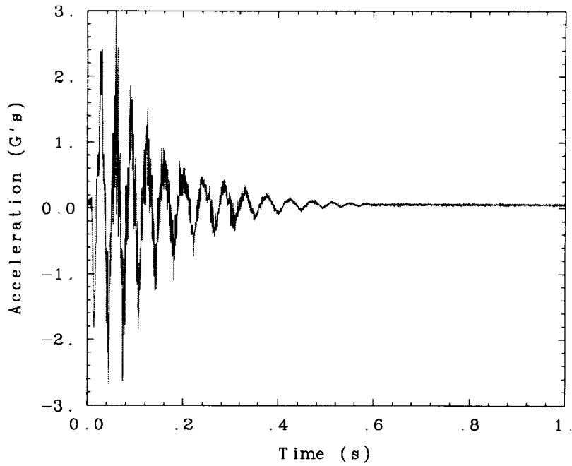
Fig. 21. Bend 1 mode twang test with pin set 3, 0° truss orientation.
