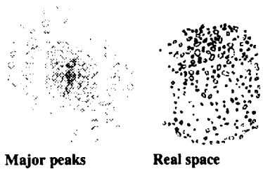
Major peaks
