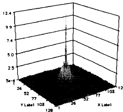
Three-dimensional intensity
