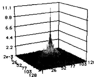
Three-dimensional intensity
