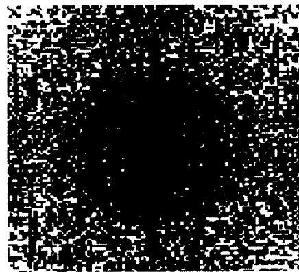
Unity gravity
