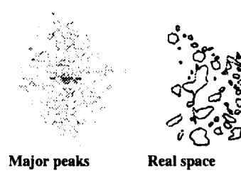
Major peaks
