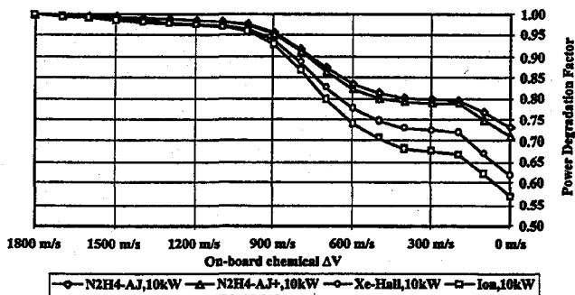
Fig. 8 Power degradation vs onboard chemical ΔV: 10-kW class GEO satellite.
