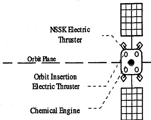
Fig. 3 Potential thruster placement.
