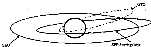
Fig. 1 Mission orbits.
