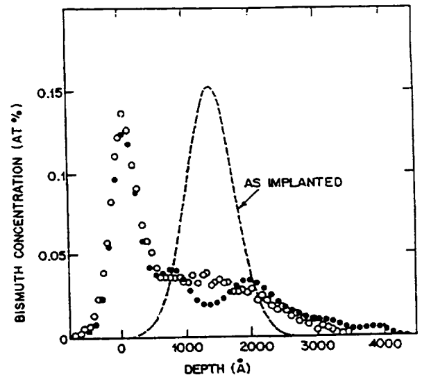
FIG. 1. The open circles are the experimental data for the depth distribution of bismuth implanted into silicon after laser melting of a surface layer. The closed circles are the depth distribution of bismuth atoms from the Monte Carlo simulations.
