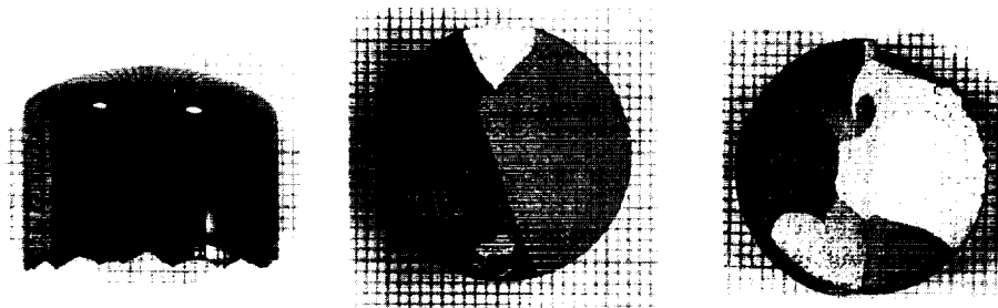
Fig. 6. Crystals. (a) Overall view. (b), (c) Cross sections of a crystal of X \approx 0.04 (no excess pressure) and X \approx 0.2 (excess P(Cd + Zn)), respectively.
