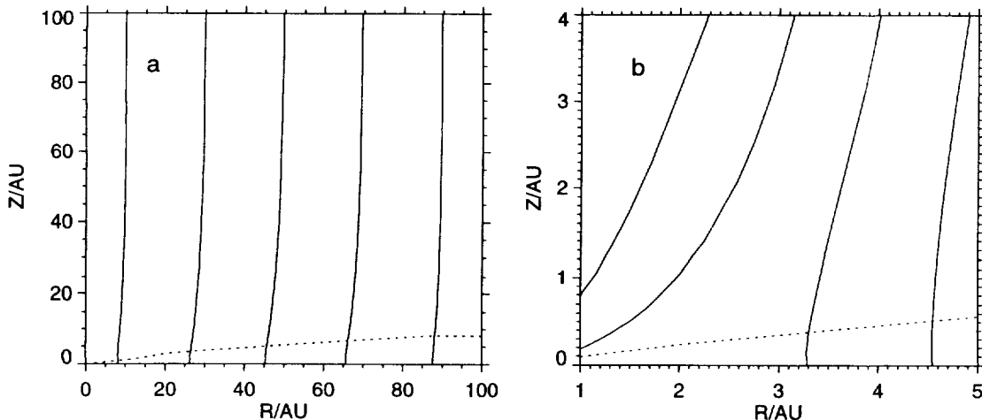
FIG. 4.—Plot of field lines of the steady state poloidal magnetic field resulting from dragging an initially uniform vertical field by the flow in a viscous proto-planetary disk characterized by \mathcal{P} = 0.01 ; (a) global view, (b) close-up of an inner portion of the disk to show the structure of the poloidal field near a region of low ionization.
