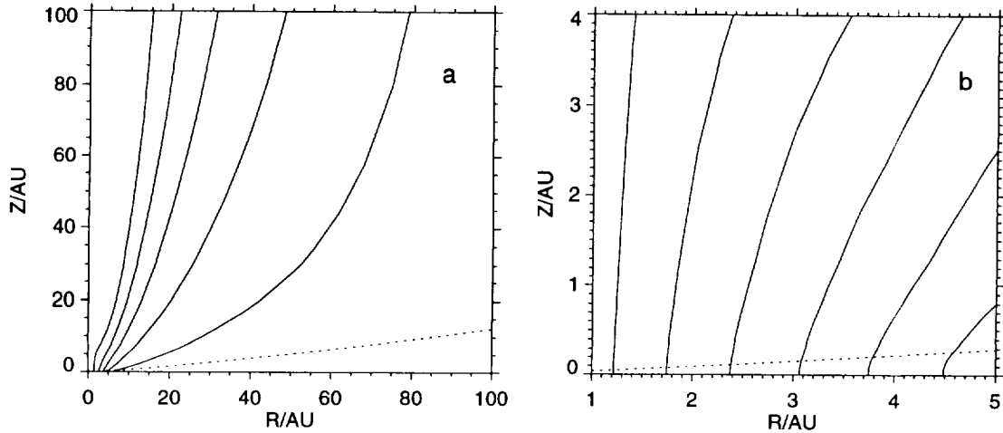
FIG. 6.—Plot of field lines of the steady state poloidal magnetic field resulting from dragging an initially uniform vertical field by the flow in a phenomenological model of a proto-planetary disk characterized by \dot{M} = 10^{-6} M_{\odot} \text{ yr}^{-1} ; (a) global view, (b) close-up of an inner portion of the disk.
