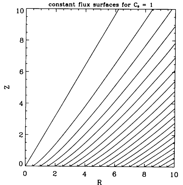
FIG. 3.—The shape of the compressed field lines for a model with \alpha = -1 and C_0 = 1 . The straight line coming from the origin shows the boundary angle, which is \theta_b = 0.552 for these parameters.
