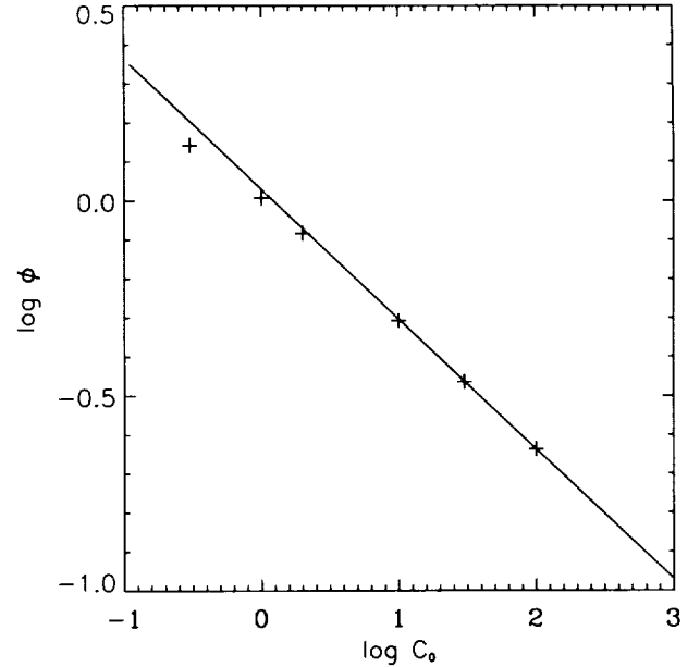
FIG. 5.—The scaling of the opening angle of the outflow \phi_{\text{BAL}} \equiv (\pi/2) - \theta_b with the parameter C_0 . The straight line is a line with slope -\frac{1}{3} ; the crosses are calculated by solving the full eq. (3.15) for different values of C_0 . It is seen that the scaling derived for C_0 \gg 1 is quite good even outside its formal range of validity.
