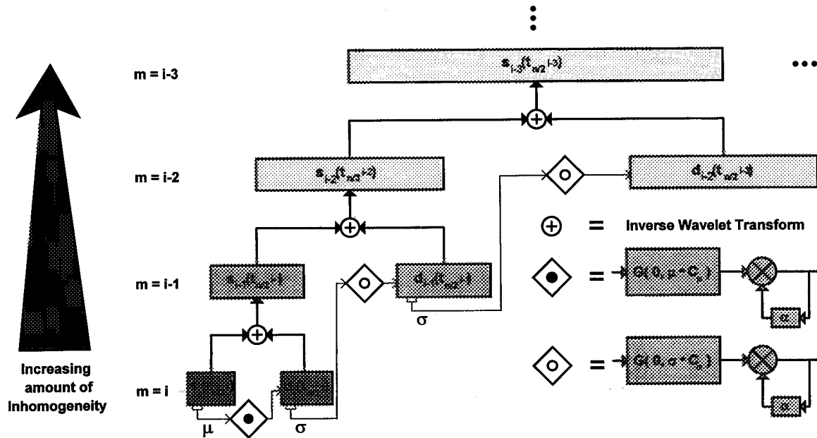
FIG. 12. Diagram of the VC model in the multiresolution framework.
