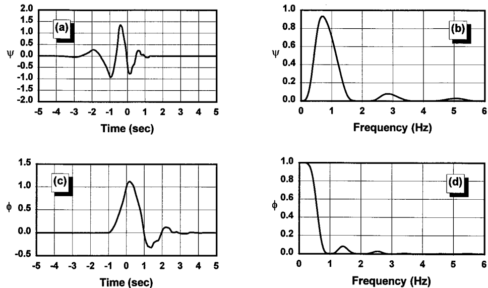
FIG. 1. Plot of the (a) D8 wavelet function, (b) its Fourier transform, (c) the corresponding scale function, and its (d) Fourier transform.
