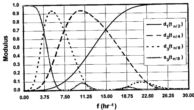
FIG. 3. Frequency ranges of multiresolution analysis for the LWP data.
