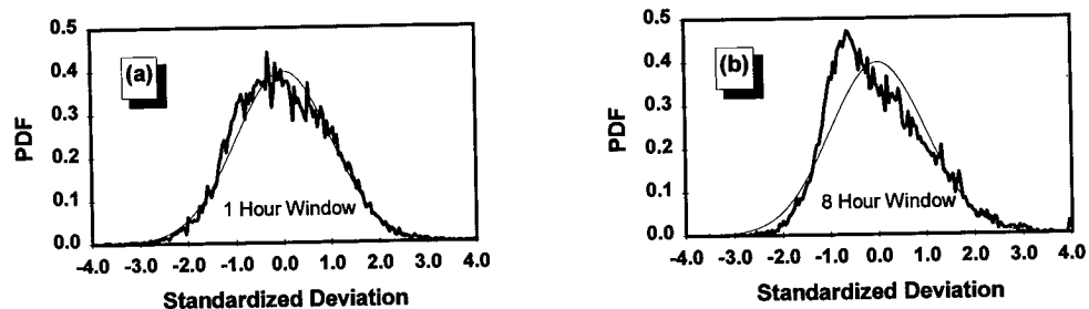
FIG. 8. LWP composite PDFs for (a) 1-h and (b) 8-h window sizes.
