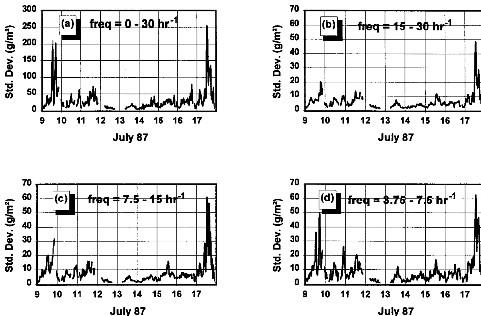
FIG. 6. Time development of the LWP data's local (a) standard deviation and standard deviation of the level (b) 1, (c) 2, and (d) 3 wavelet transform.
