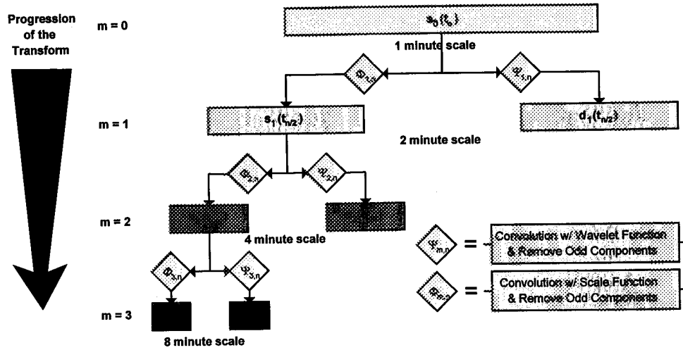
FIG. 2. Diagram of multiresolution analysis.
