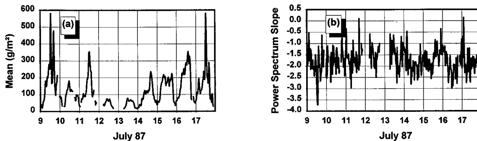
FIG. 5. Time development of the LWP data's local (a) mean and (b) slope of the power spectrum.
