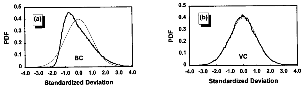
FIG. 14. Composite PDFs of the LWP from the (a) BC and (b) VC models.
