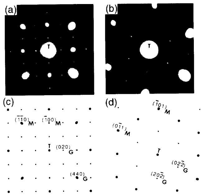
FIG. 11. (a,b) actual and (c,d) simulated [001] and [111] zone axes diffraction patterns of the \text{Ni}_{16}\text{Zr}_6\text{Si}_7 G-phase and NiAl matrix observed in the NiAl-0.05 at. % Zr alloy demonstrating the close precipitate and matrix lattice matching ( a_{\text{G-phase}} \approx 4 \times a_{\text{NiAl}} ).
