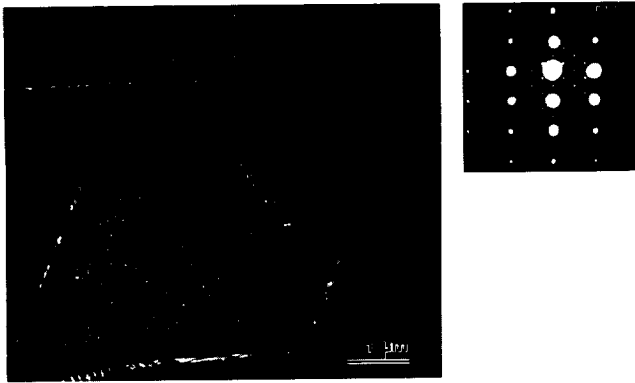
FIG. 9. TEM DF image close to a [011] zone axis showing the distribution and morphology of G-phase ( \text{Ni}_{16}\text{Hf}_6\text{Si}_7 ) in the NiAl-1.5 at. % Hf alloy after homogenization and furnace cooling.
