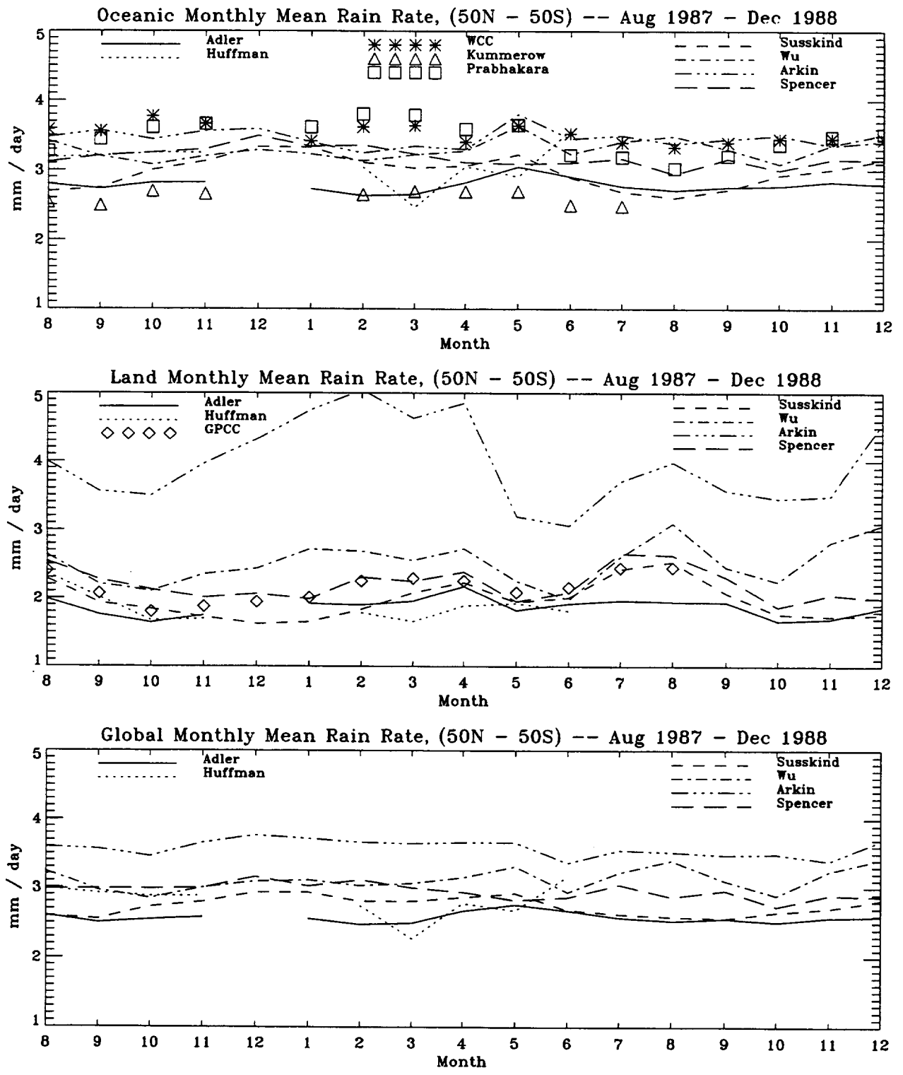
Figure 12: Time series of the global (50°N - 50°S) average for all algorithms over the oceans (upper panel), land (middle panel), and over both ocean and land (lower panel) from August 1987 to December 1988.
