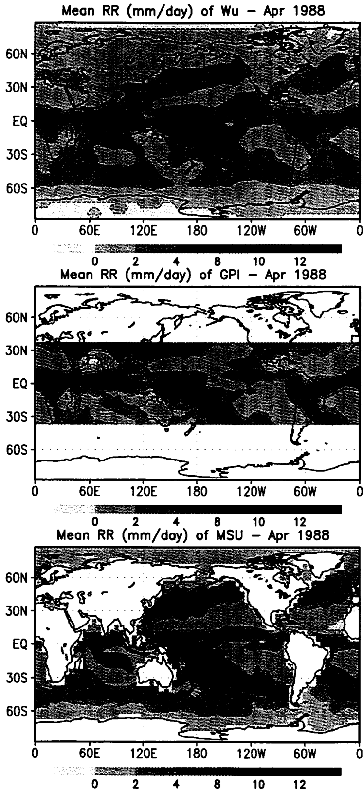
Figure 8 continued 2: Monthly rainfall for April 1988 for all algorithms.
