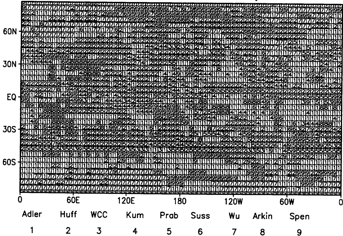
Figure 5.2: Same as Figure 3, except for May 1988.
