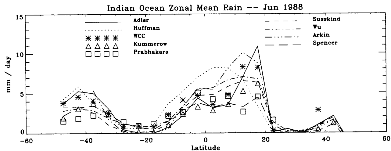
Figure 13.11: Zonal mean rain rates for the Pacific (upper panel), Atlantic (middle panel), and Indian ocean sector (lower panel) for June 1988.
