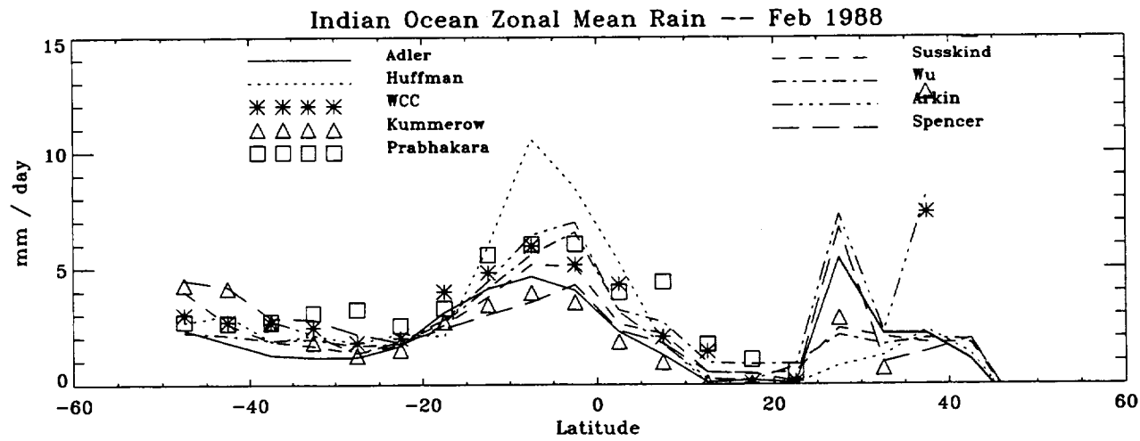
Figure 13.7: Zonal mean rain rates for the Pacific (upper panel), Atlantic (middle panel), and Indian ocean sector (lower panel) for February 1988.
