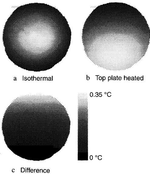
Fig. 6. Temperature measurement data a wavefront through isothermal chamber; b wavefront through heated chamber; c difference between the two
