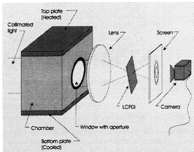
Fig. 2. Experimental apparatus for temperature measurement
