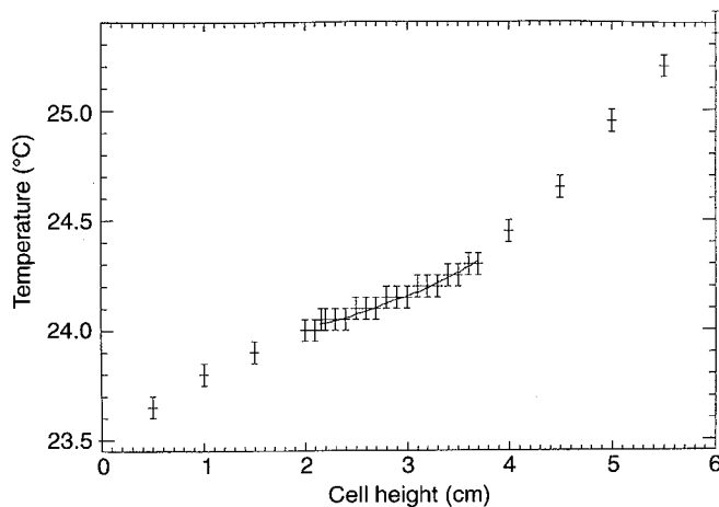
Fig. 7. Plot of temperature across chamber, measured with LCPDI (solid line) and traversing thermocouple (error bars)
