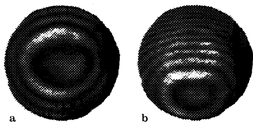
Fig. 3. Normalized masked interferograms taken a before and b after top chamber plate heated and bottom plate cooled
