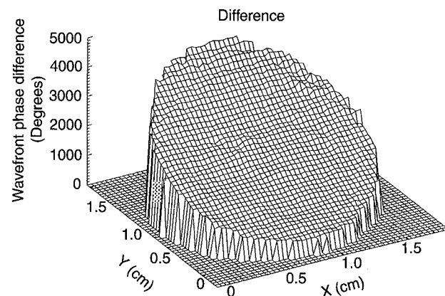
Fig. 5. Difference between wavefronts measured with isothermal and heated oil chamber
