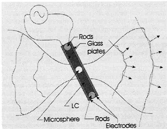
Fig. 1. Liquid crystal point diffraction interferometer filter schematic. Dashed lines indicate reference wave, solid lines indicate object wave
