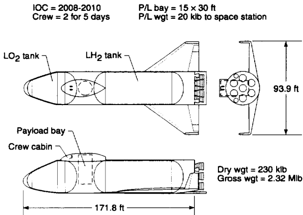
Figure 24. Reference rocket-powered SSTO configuration (ref. 17).
