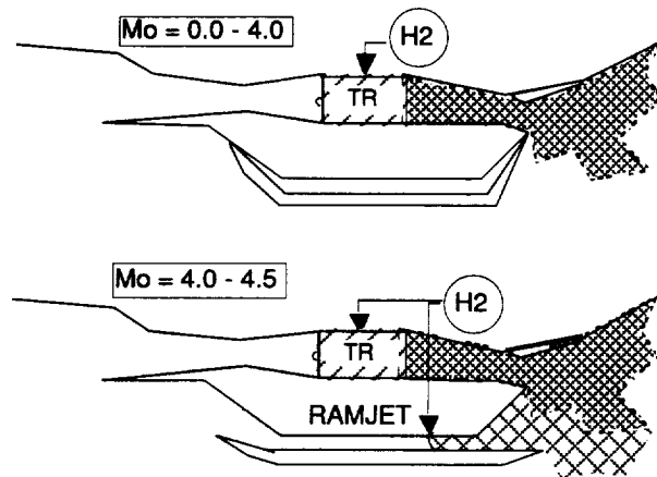
Figure 9a. Propulsion system operation (initial acceleration).
