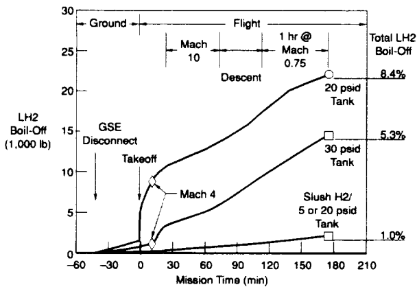
Figure 14. Boil-off comparison of liquid and slush hydrogen fuel system (ref. 6).
