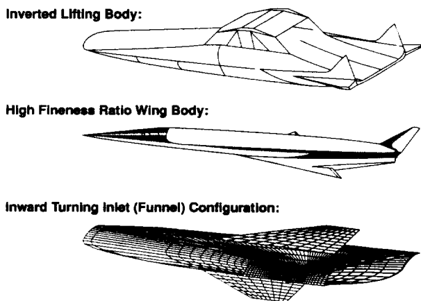
Figure 34. Extended/advanced configuration matrix (ref. 1).
