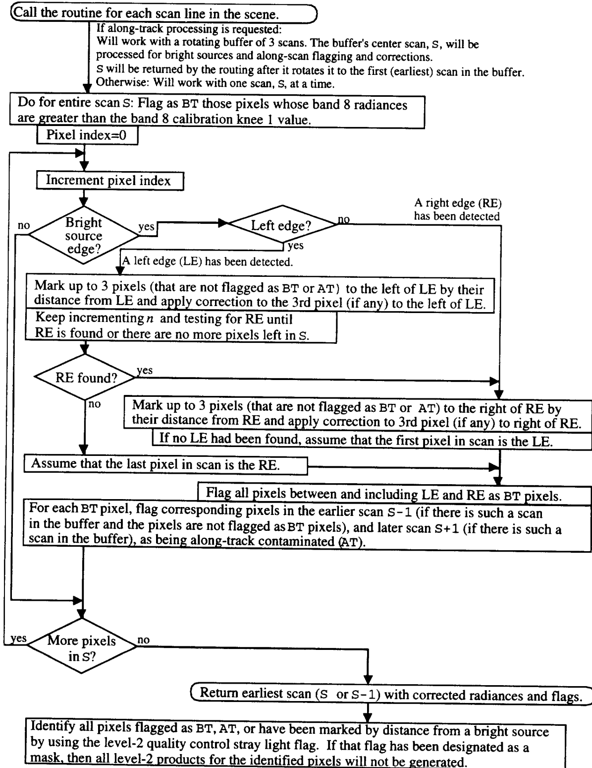
Fig. 12. Logic flow diagram for the detection and correction of stray light in SeaWiFS GAC level-1 data.
