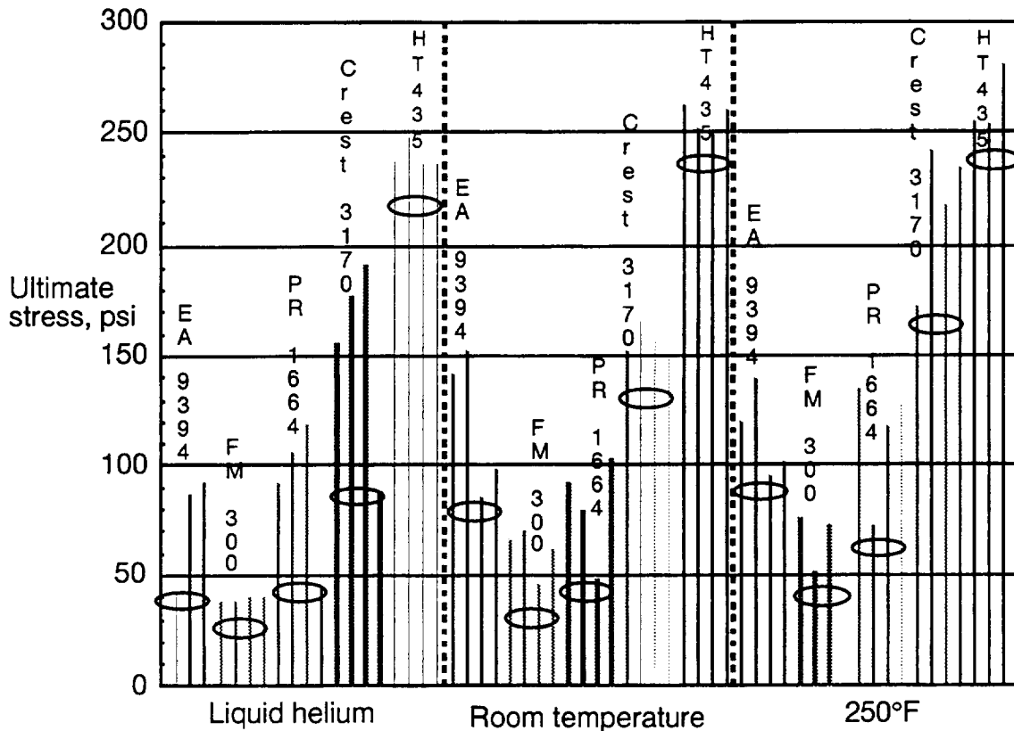
Figure 7: Ultimate stress of HRP honeycomb drill core bonded to Gr/Ep with five different adhesives and three different pre-conditionings tested at room temperature.
