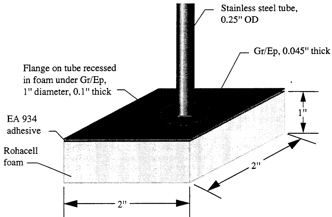
Figure 1: Schematic diagram of test specimen with stainless steel tube embedded between Gr/Ep and Rohacell foam.
