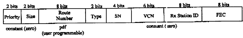
Figure 4: Packet Header Format
