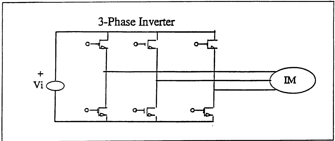
Figure 9. VSI-PWM Based IM-ASD Set.
