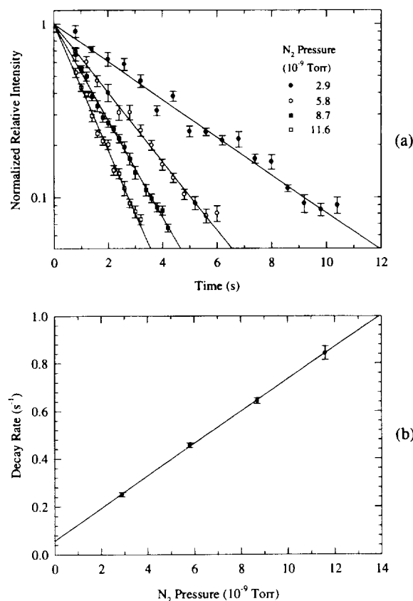
FIG. 3. (a) The normalized relative intensity of N^{2+} vs storage time at four different pressures of N_2 . (b) N^{2+} decay rate vs N_2 pressure.
