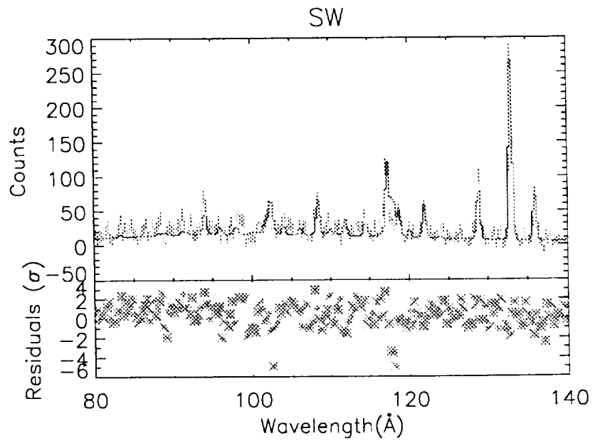
Figure 5. EUVE SW Spectral fits and residuals.
