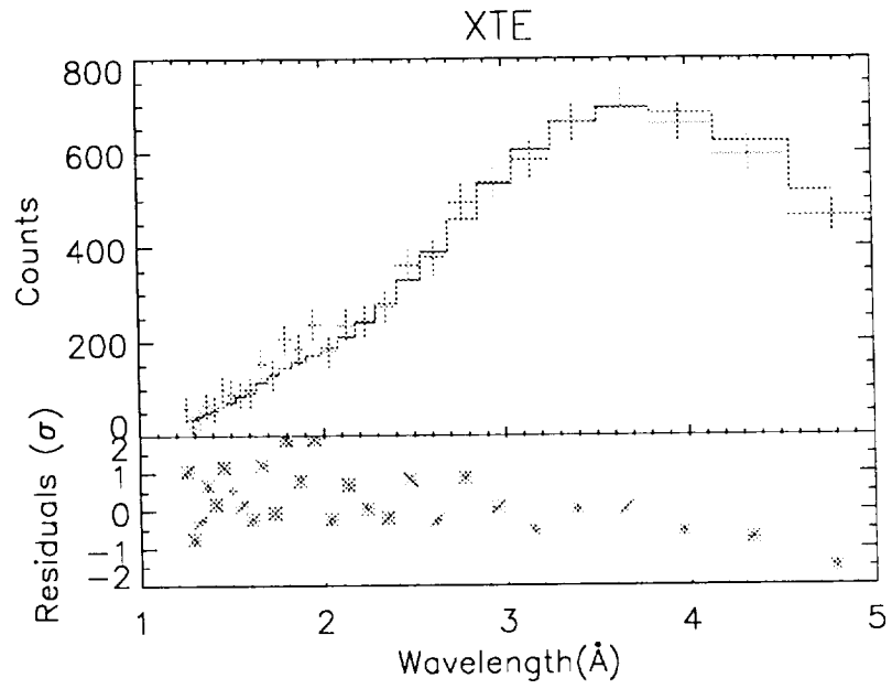
Figure 8. RXTE PCA Spectral fits and residuals.
