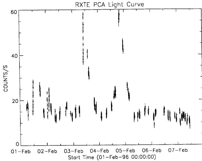
Figure 4. RXTE PCA Lightcurve for Algol observation.
