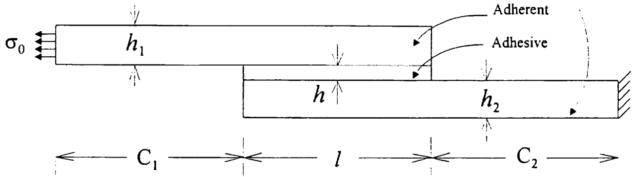
(a) without adhesive overflow
