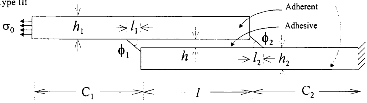
(c) with adhesive overflow
