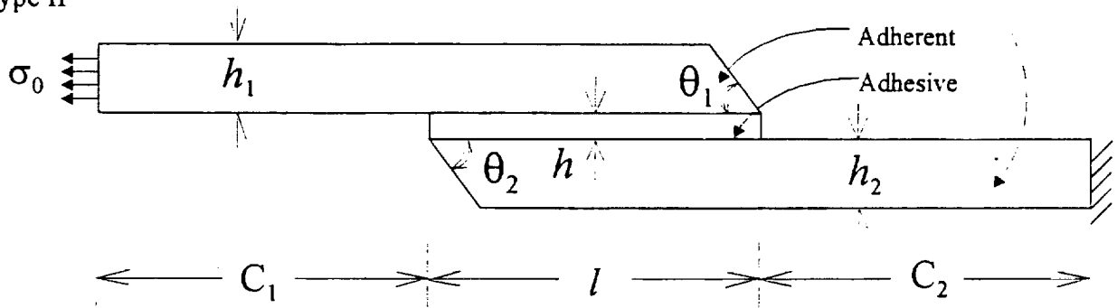
(b) with beveled adherents
