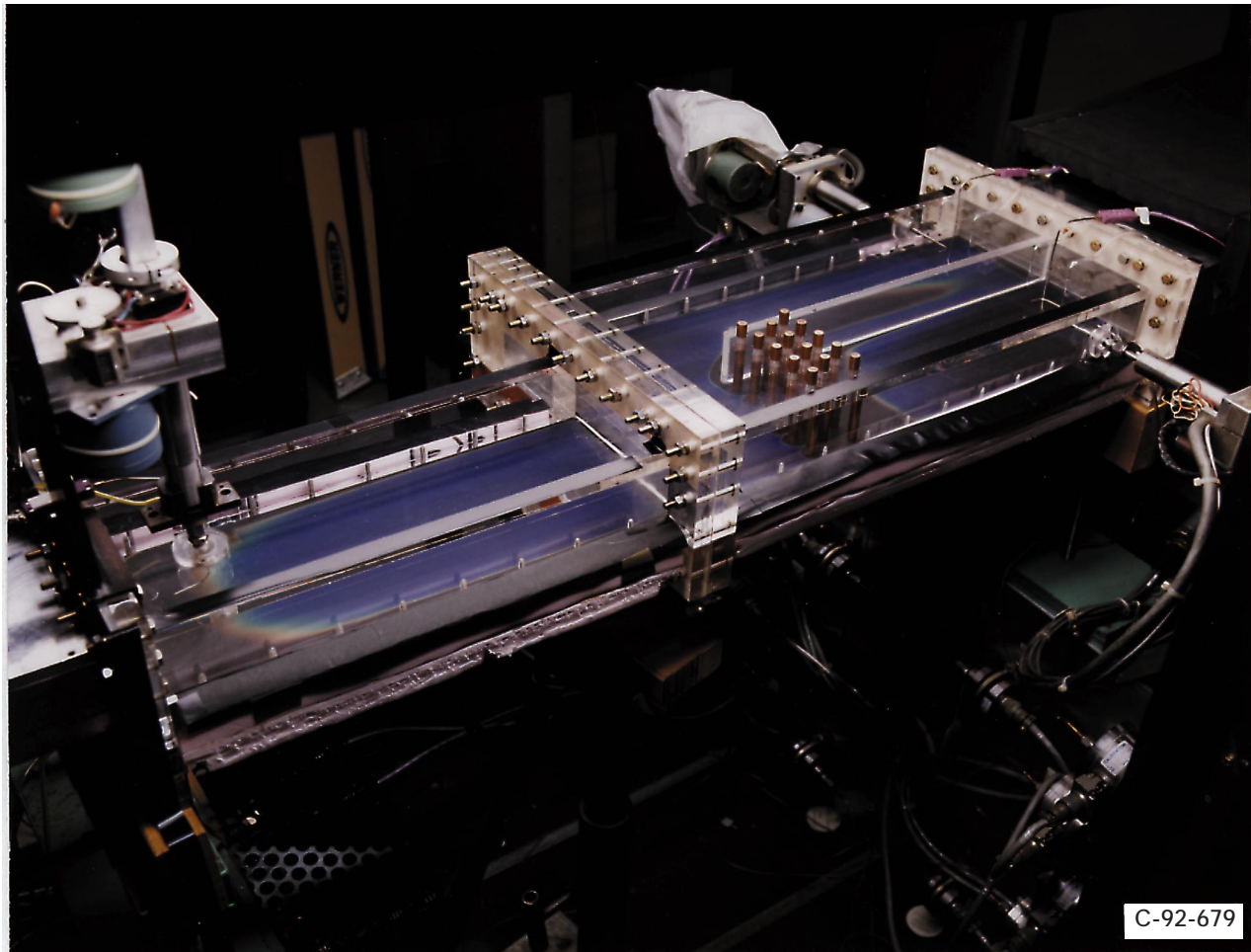
Figure 7.—Test section under flow conditions ( Re_{\text{entrance}} = 45\,000 ).
