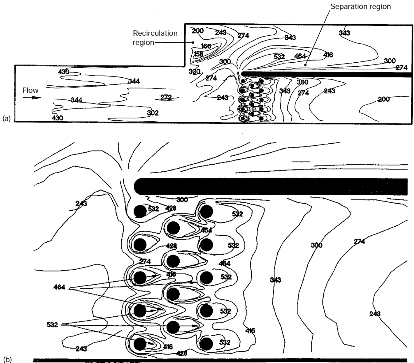
Figure 14.—Experimental heat transfer coefficients ( Re_{\text{entrance}} = 726\,000 ). (Coefficients given in W/m^2-K .) (a) Entire test surface. (b) Closeup of area.
