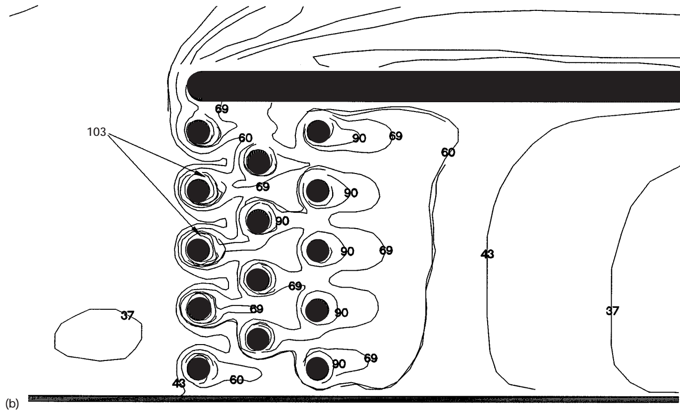
Figure 12.—Experimental heat transfer coefficients ( Re_{\text{entrance}} = 45\,000 ). (Coefficients given in W/(m^2-K) ) (a) Entire test section. (b) Closeup of pin area.
