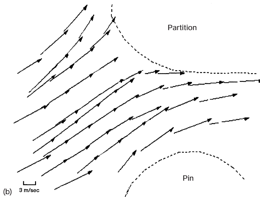
Figure 15.—Particle trajectories ( Re_{\text{entrance}} = 45\,000 ). (a) Video picture. (b) Velocity vector diagram.
