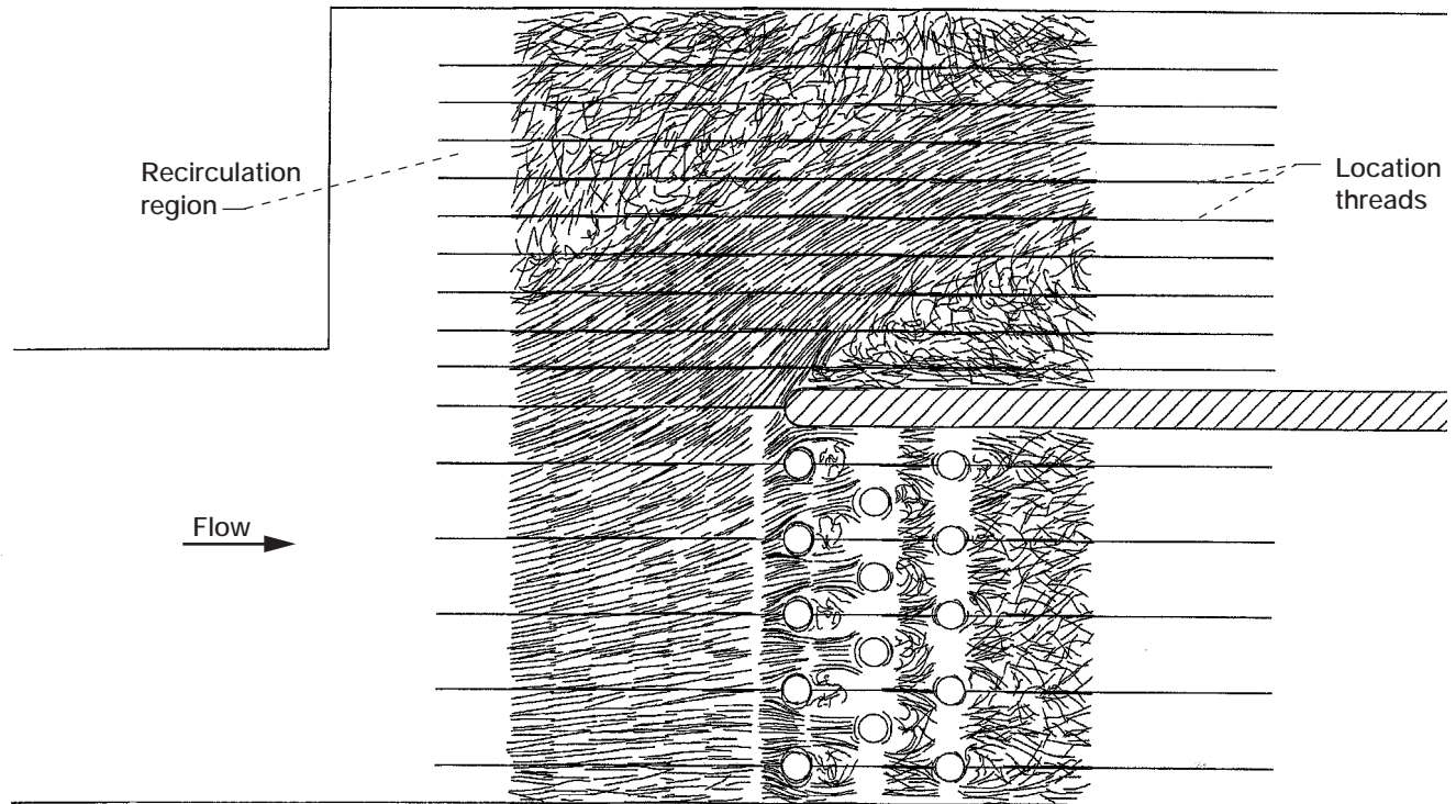
Figure 16.—Composite of digitized video data showing streamlines (300 video frames combined ( Re_{\text{entrance}} = 45\,000 )).
