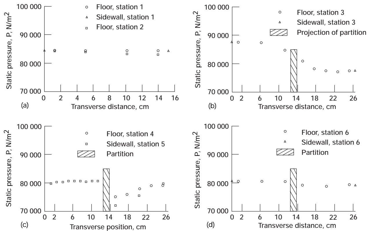
Figure 17.—Floor and sidewall static pressures (looking upstream). ( Re_{\text{entrance}} = 726\,000 ).
