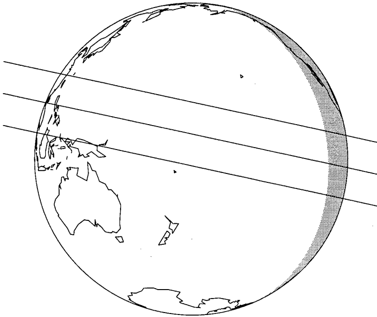
Fig. 5 Occultation of a 12.8 mag star by Pluto on November 11, 2002. The globe at the left shows a view of the Earth from Pluto when it occults a R = 12.8 mag star (McDonald, private communication). The centerline is the predicted center of Pluto's shadow, and the other two lines represent the limit of the northern and southern limbs. The shaded area is the region for which the sun is greater than 8 degrees below the horizon (Pluto is 33 deg from the sun). Both HOPI channels could obtain \sim 5 times the signal-to-noise of the light curve shown in Fig. 3 in the visible. Since the star is extremely red ( B - R = 3.5 ), with simultaneous observations in the K band (with the facility IR camera, if it can record occultation data) we could obtain a light curve with comparable S/N. With these data we could answer the question of whether Pluto's atmosphere has a haze layer or sharp thermal gradient. Note that this event (if it follows the current prediction) would be easily accessible with SOFIA, but inaccessible from ground-based telescopes.
