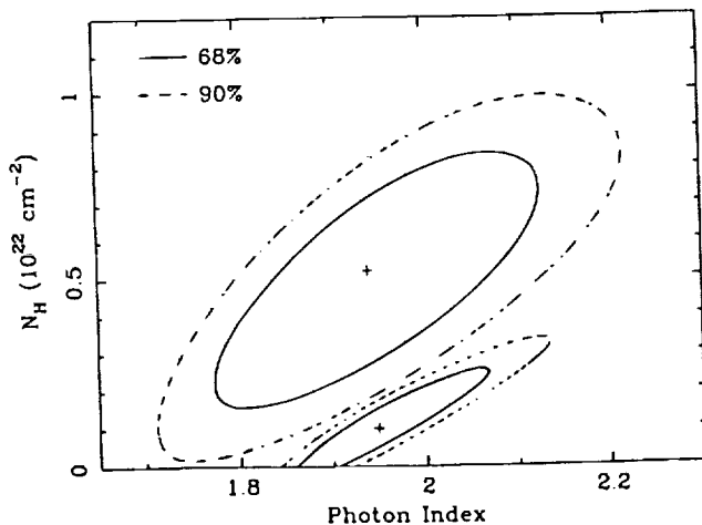
FIG. 4.— \chi^2 contours (90% and 1\sigma ) for the average 1988 Ginga spectrum and the 1989 Ginga spectrum for a joint fit of the reflection model, allowing the index and absorption to vary. These show that in the context of the reflection model, the spectral variability can be explained by variation in the neutral absorption column.
