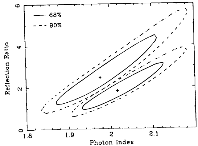
FIG. 5.— \chi^2 contours (90% and 1\sigma ) for Ginga spectra G88.1 and G88.2 from a joint fit of the reflection model, allowing the index and reflection ratio to vary. These show that in the context of the reflection model, the spectral variability can be attributed to variability in the ratio or the index or both.
