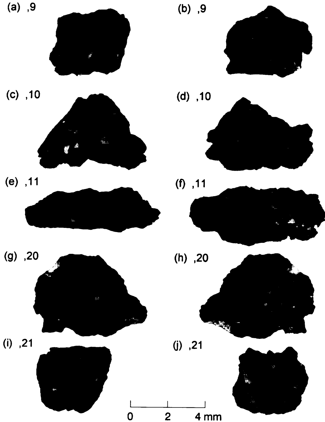
FIG. 1. Photomicrographs of subsplits of QUE 93069 analyzed by INAA. Two photographs are shown for each subsample ( e.g. , a and b are opposite sides of the same rock chip). Point counts of enlarged versions of these and additional photographs were used to estimate the proportion of clasts greater than \sim 100 \mu\text{m} . The results are as follows (clasts:matrix): split 9 (21:79); split 10 (40:60); split 11 (28:72); split 20 (31:69); and split 21 (20:80). The average proportions are 28% clasts and 72% matrix. These are minimum clast proportions because they neglect clasts smaller than \sim 100 \mu\text{m} .
