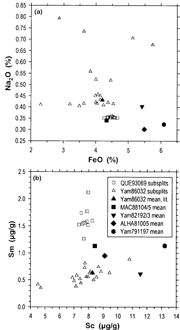
FIG. 7. Concentrations of (a) \text{Na}_2\text{O} and FeO and (b) Sm and Sc in subsplits of QUE 93069 and Yamato 86032 (this work) and comparison to mean concentrations in other feldspathic lunar meteorites. The five subsplits of Yamato 86032 that are rich in white clastic material are indicated by dotted triangles. For Yamato 86032, the mean is that of Koeberl et al. (1989); subsplits analyzed here are slightly more feldspathic on average. In this figure and throughout this work, average compositions of lunar meteorites are plotted and discussed. We have calculated these averages from the following sources and other references cited therein: Takeda et al. (1989), Koeberl et al. (1989, 1990), Jolliff et al. (1991, 1996), Warren and Kallemeyn (1991), Lindstrom et al. (1991), Palme et al. (1991), and this work.
