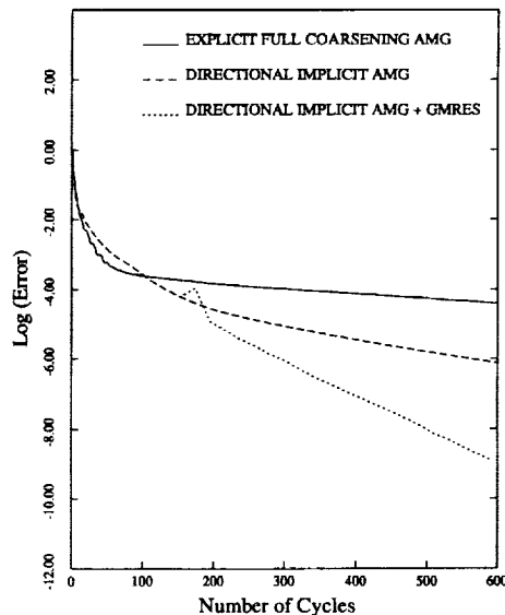
FIG. 18. Comparison of Convergence Rates Achieved by Various Multigrid Schemes for Flow Over Partial Span Flap Geometry
