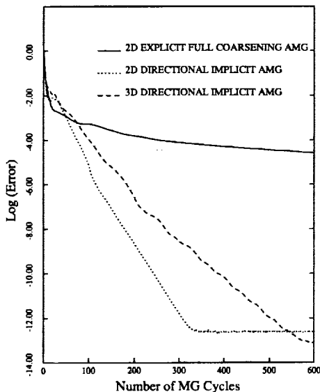
FIG. 13. Comparison of Convergence Rate obtained by Three-Dimensional Directional-Implicit Multigrid Algorithm with Rate Obtained on Equivalent Two-Dimensional Problem
