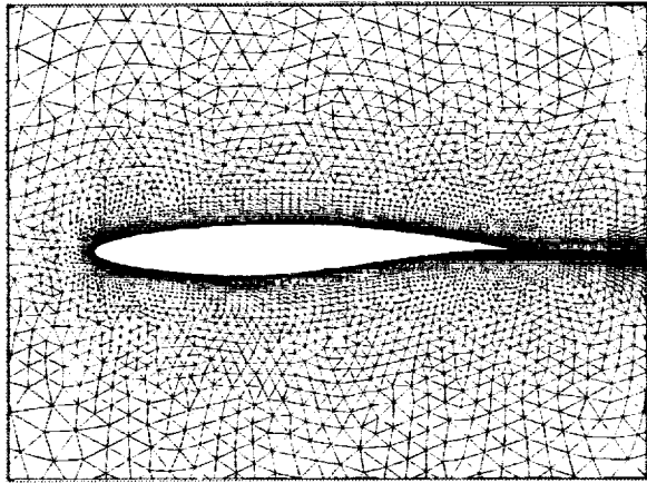
FIG. 2. Unstructured Grid Used for Computation of Transonic Flow Over RAE 2822 Airfoil. Number of Points = 16167, Wall Resolution = 10^{-6} chords
