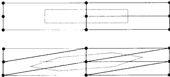
FIG. 1. Median control-volumes for stretched quadrilateral and triangular elements
