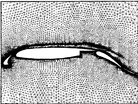
FIG. 8. Unstructured Grid Used for Computation of Subsonic Flow Over Three-Element Airfoil Geometry. Number of Points = 61,104, Wall Resolution = 10^{-6} chords
