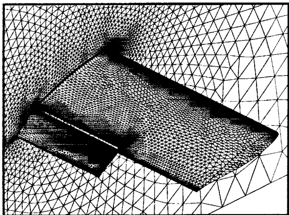
FIG. 16. Illustration of Unstructured Grid employed for Computation of Flow Over Partial-Span Flap Geometry. Number of Vertices = 549,176
