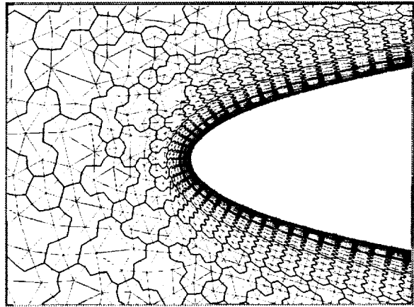
FIG. 4. First Agglomerated Multigrid Level Constructed on Grid of Figure 2 Illustrating 4:1 Directional Coarsening in Boundary Layer Region
