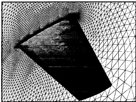
FIG. 14. Illustration of One of Three Unstructured Grids Employed For Computation of Flow Over ONERA M6 Wing: Number of vertices= 1.6 million, Wall Spacing = 10^{-6}
