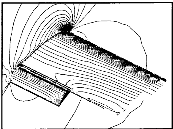
FIG. 17. Illustration of Computed Density Contours for Flow Over Partial-Span Flap Geometry. Mach Number = 0.2, Incidence = 10 degrees, Reynolds Number = 3.2 million
