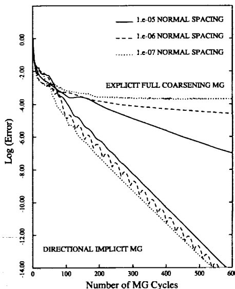
FIG. 6. Comparison of Explicit Isotropic and Directional-Implicit Agglomeration Multigrid Algorithm Convergence Rates on 3 Grids of Varying Normal Resolution
