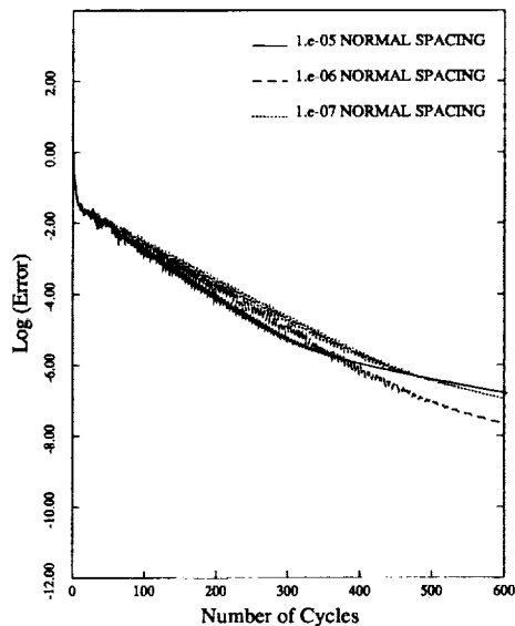
FIG. 15. Comparison of Convergence Rates Achieved by Directional Implicit Agglomeration Multigrid Algorithm on 3 Grids of Varying Normal Resolution for ONERA M6 Wing Geometry at Mach number = 0.1
