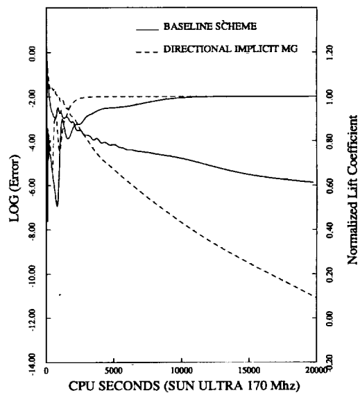
FIG. 11. Comparison of Convergence Rates obtained for Flow Over Three-Element Airfoil in terms of CPU time on Workstation
