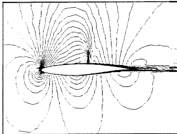
FIG. 5. Computed Mach Contours on Grid of Figure 2. Mach = 0.73, Incidence = 2.31 degrees, Re = 6.5 million
