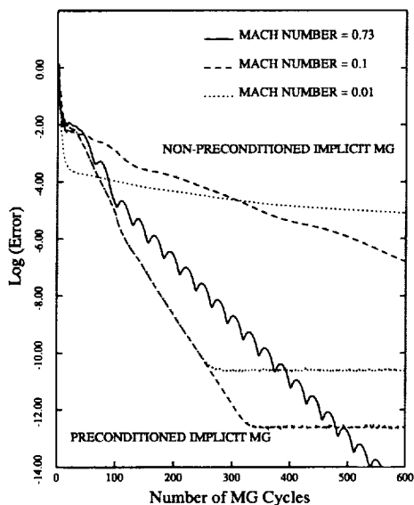
FIG. 7. Comparison of Low-Mach Number Preconditioned and Unpreconditioned Directional-Implicit Agglomeration Multigrid Algorithm Convergence Rates for Various freestream Mach Numbers
