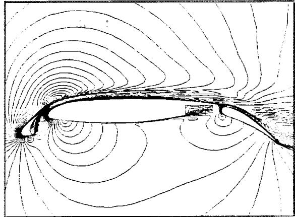
FIG. 10. Computed Mach Contours for Flow over Three-Element Airfoil. Mach = 0.2, Incidence = 16 degrees, Reynolds number = 9 million
