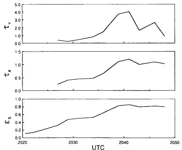
FIG. 18. Cloud optical properties derived from Fig. 17.
