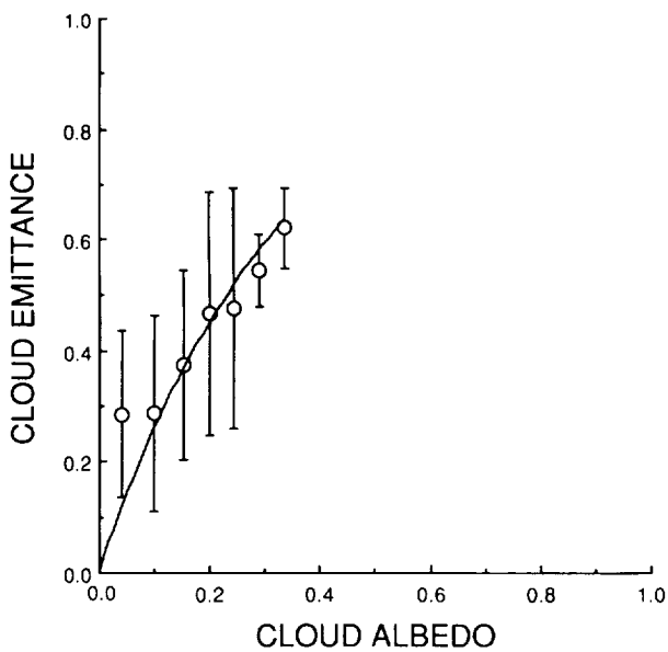
FIG. 5b. Cloud albedos and mean cloud emittances derived from Fig. 5a without "dark" pixels. Vertical lines represent standard deviations. The curved line denotes the regression fit to Eq. (7).
