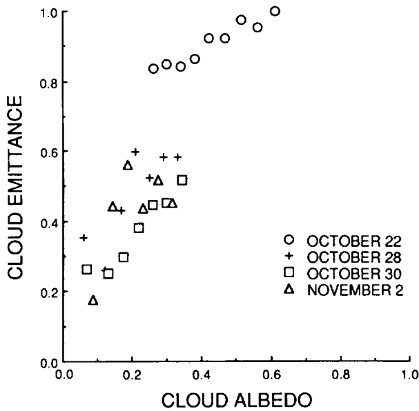
FIG. 8. Average cloud emittances and albedos from GOES at 2100 UTC over FMC during different IFO days.
