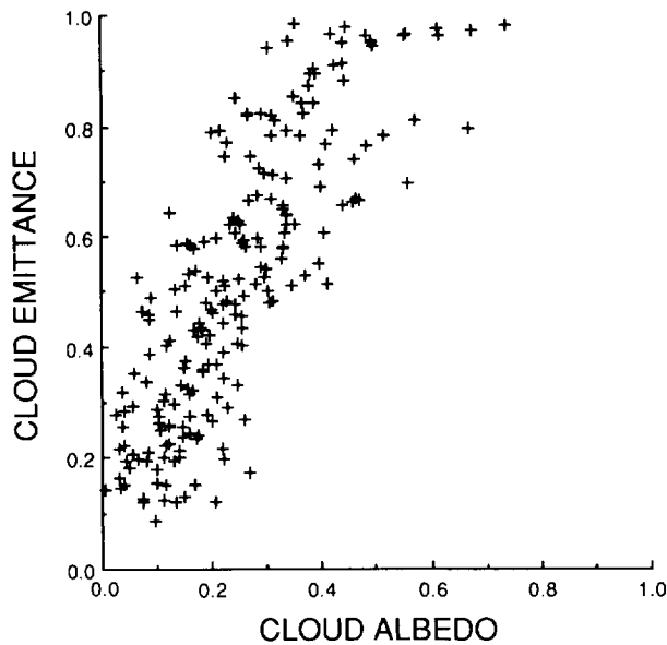
FIG. 9a. Average cloud emittance versus cloud albedo for all case study scenes from GOES over surface sites where T_s = T_c .
