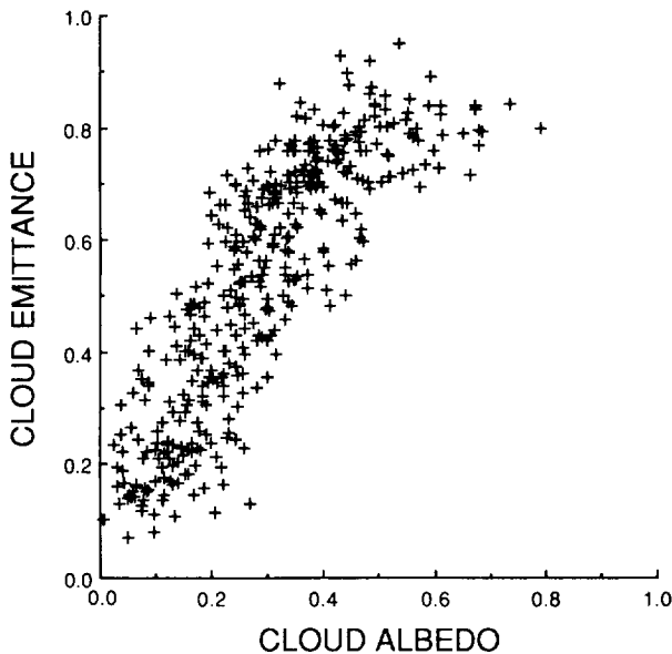
FIG. 15. Same as Fig. 9b, except T_c = T_c .
