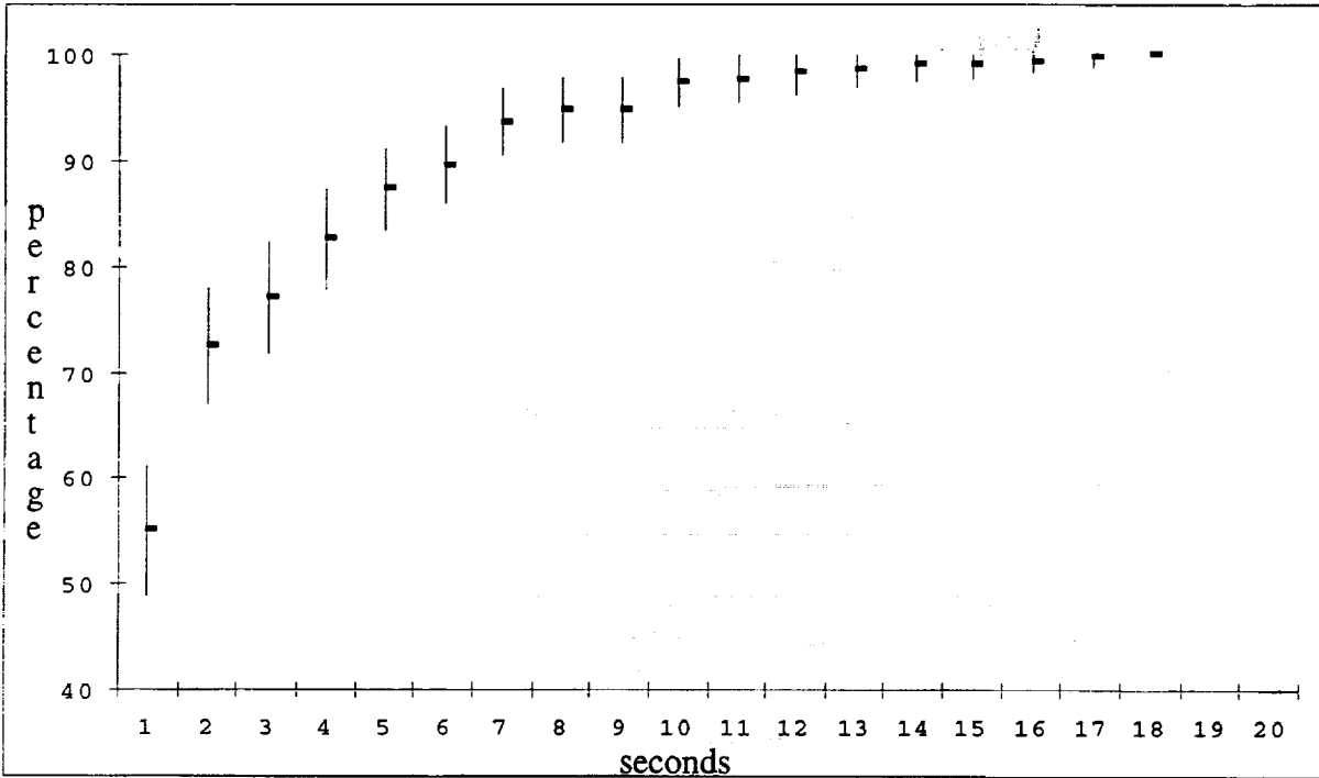
Figure 13. Availability of traffic data onboard the TSRV (percentage) versus delay (seconds).
