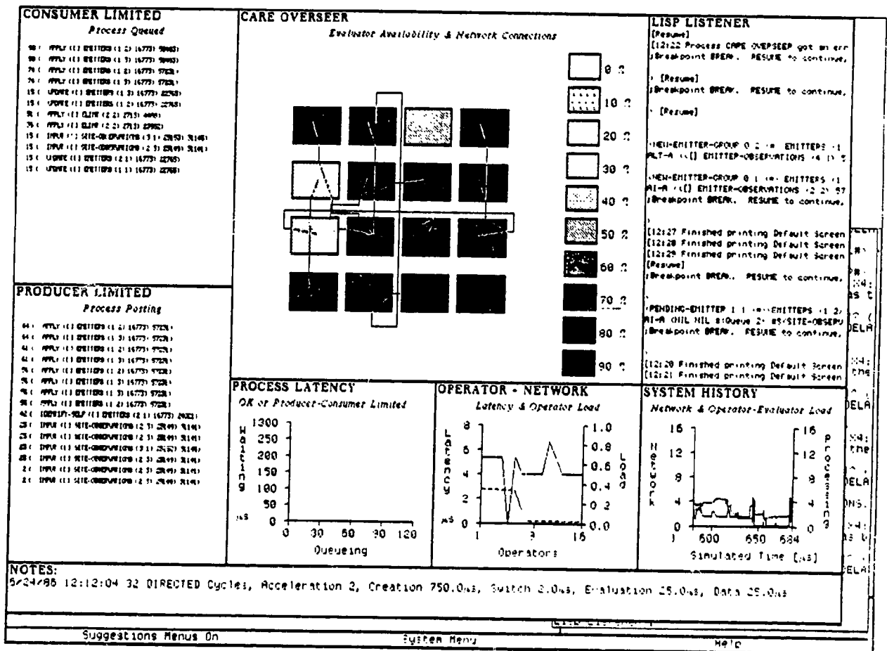
Figure 17: Overseer Instrument
