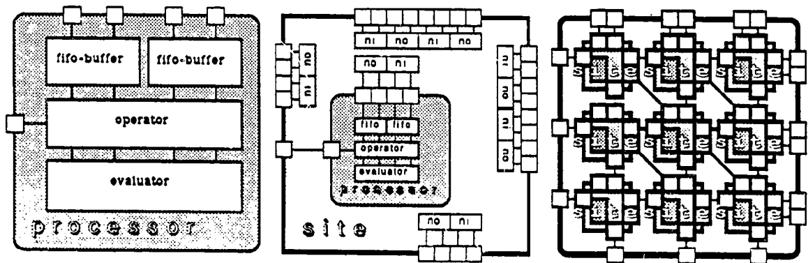
Figure 2: Hierarchical Composition
