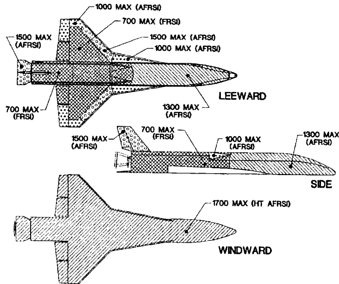
Figure 29. Thermal protection system multi-use temperature limits ( ^{\circ}\text{F} ).
