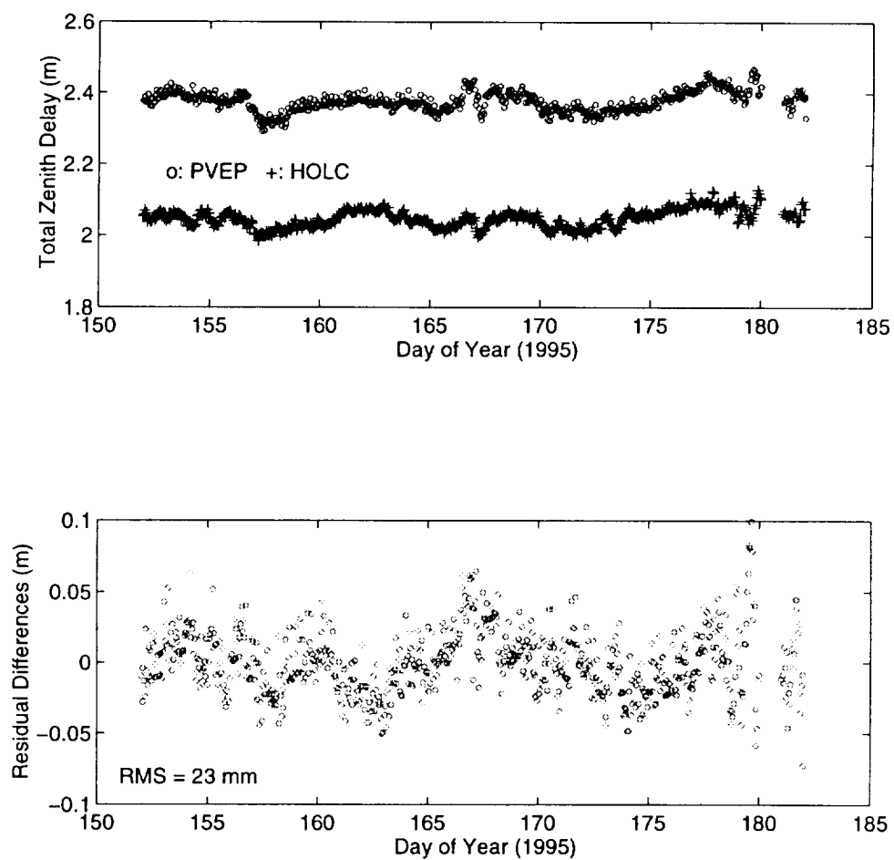
Figure 14: Neutral zenith delay time series of PVEP and HOLC and demeaned differences between these two sites. These differences indicate the magnitude of spatial variation.
