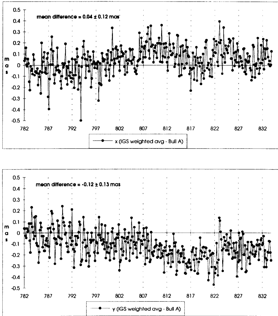
Figure 3: Difference between IGS mean and Bulletin A EOP values for 1995. (Bulletin A EOP were corrected with the ITRF93 inconsistency parameters)
