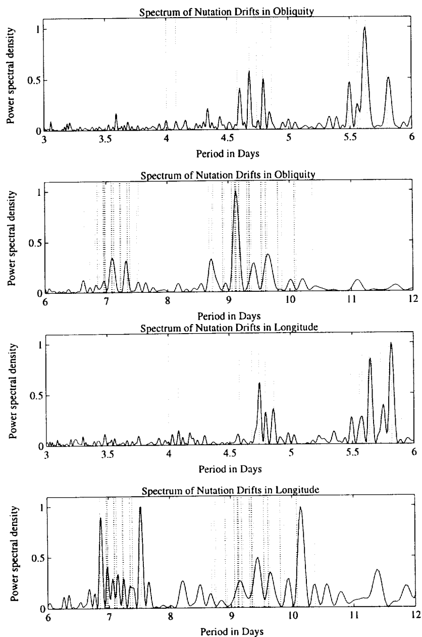
Figure 7: Spectrum of Nutation Corrections in Obliquity and Longitude Derived From the CODE Results in the Time Interval from April 1994 to January 1996.
