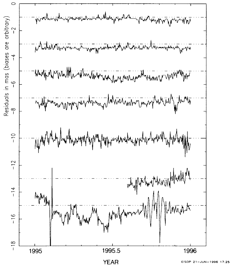
Figure 2: X pole coordinate in 1995. Daily differences of individual GPS series with IERS 95 P 01. Top to bottom: GFZ, JPL, CODE, EMR, ESOC, NOAA, SIO.
