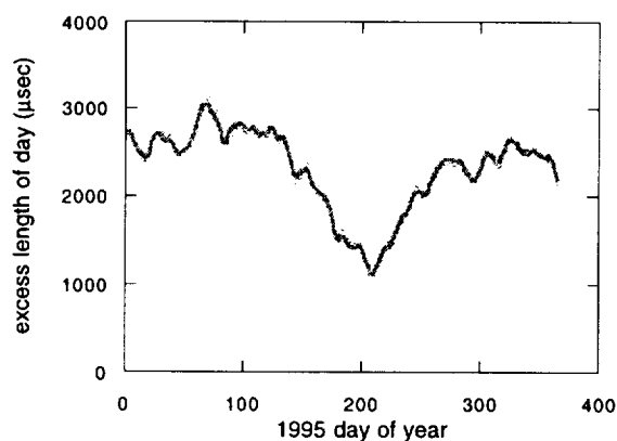
Figure 2: Length of day performance in 1995. Each dot corresponds to a daily estimate from the JPL AC; the shaded background indicates the IERSB Final value (from the time derivative of UTR1). The average difference of 2 \mu\text{sec}/\text{day} is insignificant. The low scatter of 46 \mu\text{sec}/\text{day} demonstrates the value of GPS estimates.
