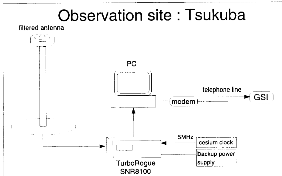
Figure 1: equipment on the Tsukuba site
