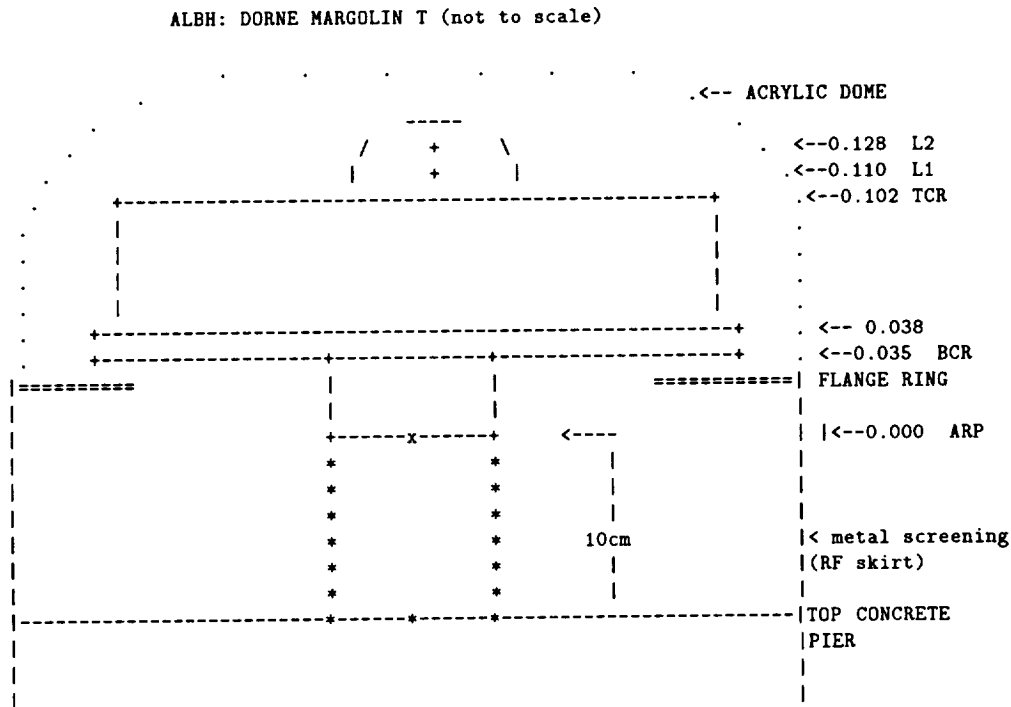
Figure 2: Antenna Schematic for Albert Head (ALBH) GPS Station
