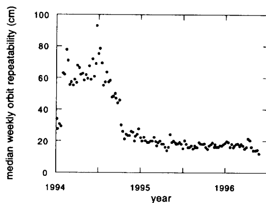
Figure 1: JPL orbit repeatability (3drms) since the official start of the IGS in 1994. Each weekly number indicates the median over all satellites and days during that week. (The daily number for a given satellite indicates the degree to which the precise orbit agrees with those of adjacent days near the midnight boundary.) Beginning in late 1994, the typical weekly value is about 20 cm or less.
