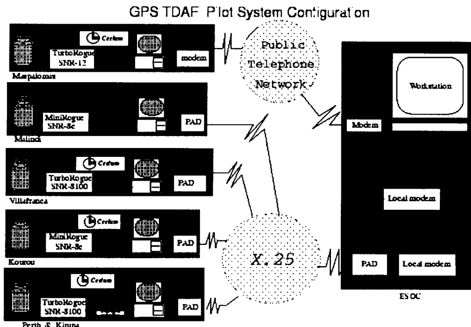
Figure 3: GPS-TDAF Plot System Configuration
