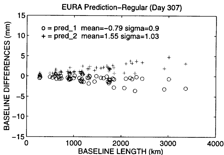
Figure 10: Baseline length determination comparison of using prediction 1 and prediction 2. The scatters show noticeable scaling errors in both cases.
