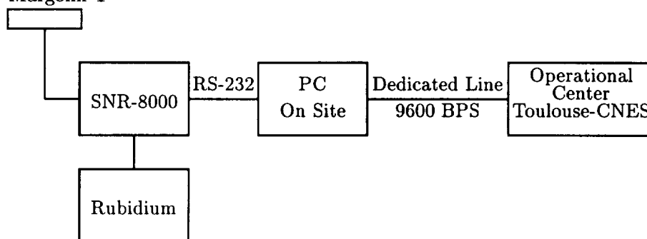
Figure 2: GPS System Configuration — Hartebeesthoek
