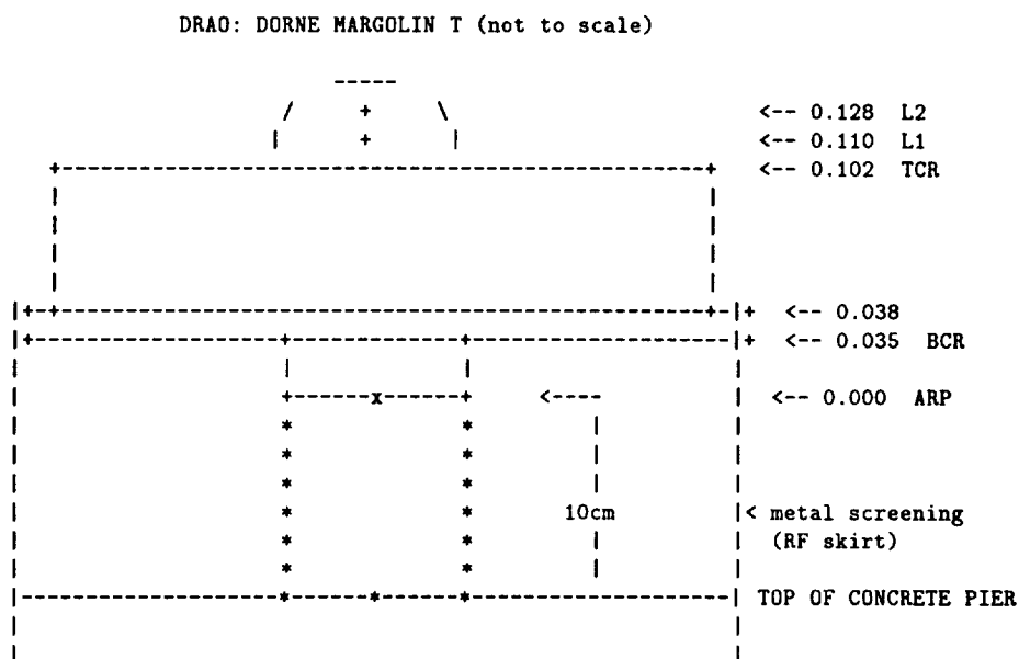
Figure 1: Antenna Schematic for Penticton (DRAO) GPS Station
