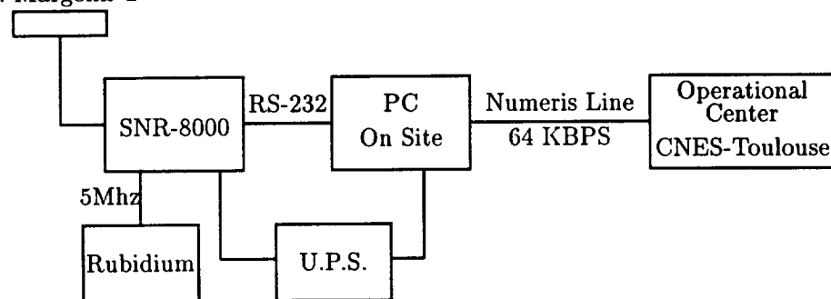
Figure 4: GPS Configuration: Pamatai
