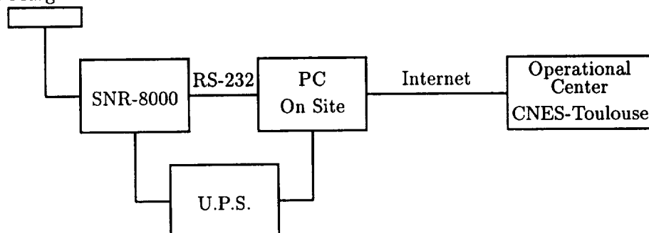
Figure 1: GPS System Configuration — Grasse
