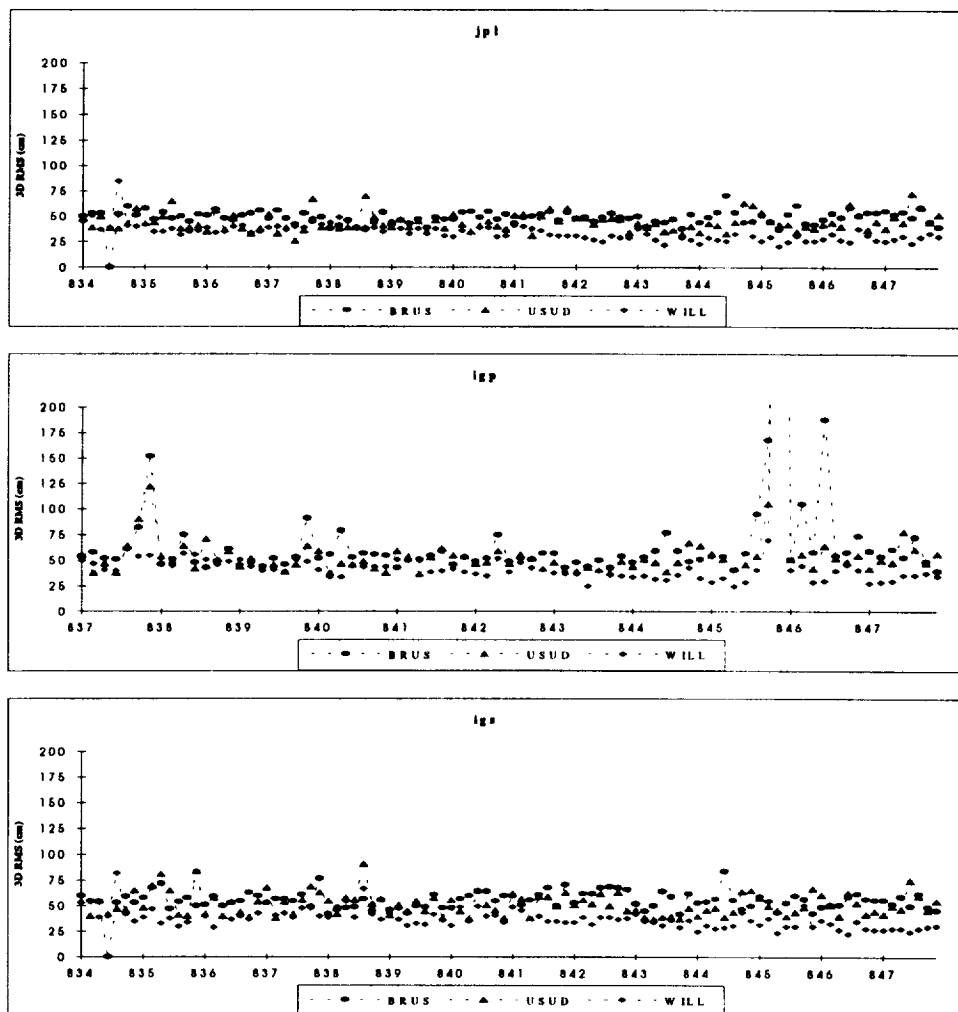
Figure 2: Rapid Combination—1996 Daily 3D Point Positioning RMS (navigation mode) for JPL, IGP and IGS.
