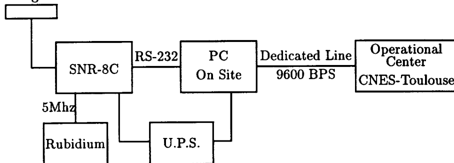
Figure 3: GPS System Configuration — Kerguelen
