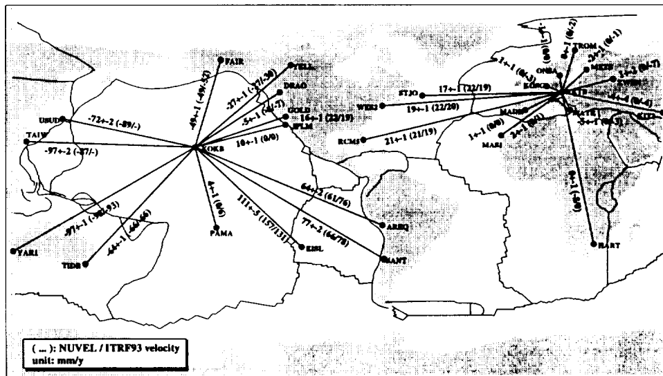
Figure 6: Baseline Rates of KOKB and WETB to Neighbouring Sites Derived from Weekly Coordinate Solutions (NUVEL-1 and ITRF93 values are given in parantheses).
