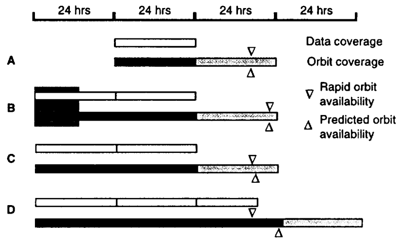
Figure 6: Orbital Prediction Schemes. Pred-A/B/C can only provide a few hours of real time orbit with sufficient precision while Pred-D can provide a full 24 hours of real time orbit coverage.
