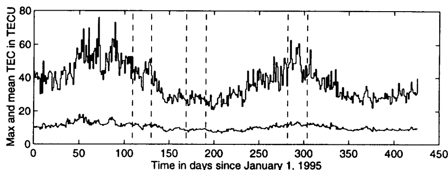
Figure 9: Maximum and Mean TEC Values Extracted from the Daily CODE GIMs. Shown in TEC units
