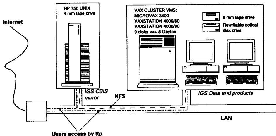
Figure 1: Computer architecture
