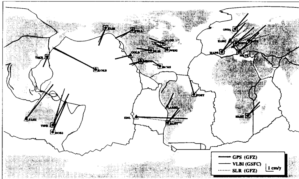
Figure 5: Site Velocities as Determined from Different Techniques:
