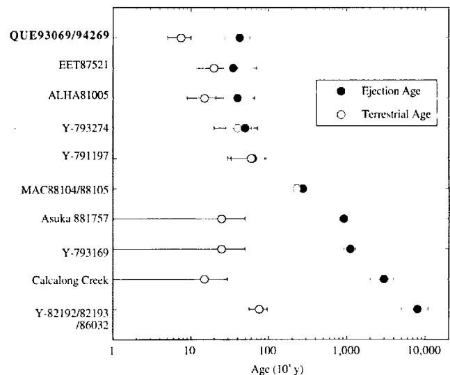
FIG 1. Ejection ages and terrestrial ages of lunar meteorites. The open circles indicate terrestrial ages, and the closed circles indicate ejection times from the Moon. The distance between the two circles indicates the transition time from the Moon to the Earth.
