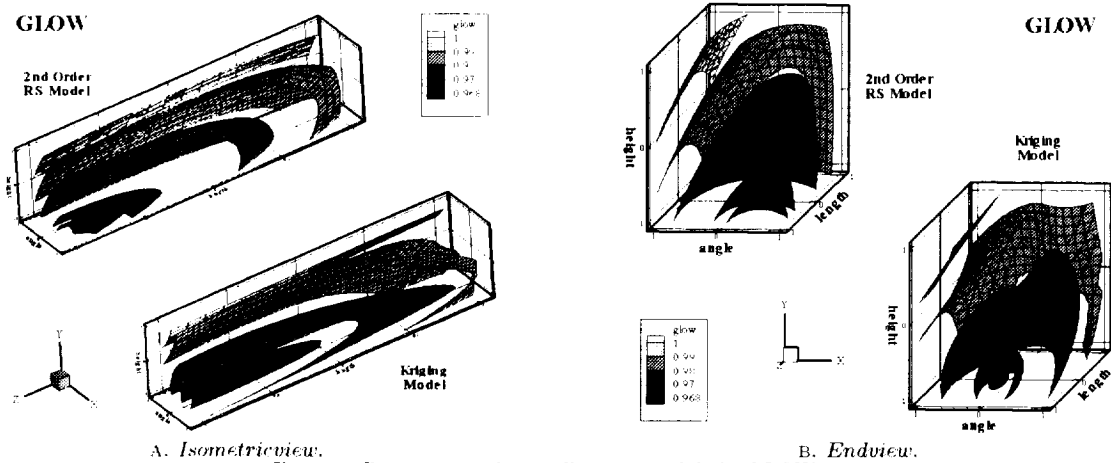
FIG. 11. Response surface and kriging models for GLOW.
