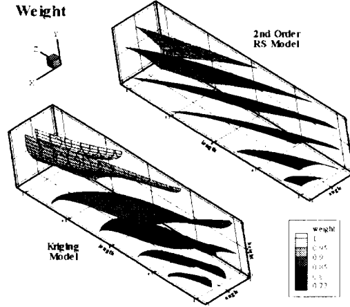
FIG. 10. Response surface and kriging models for weight.
