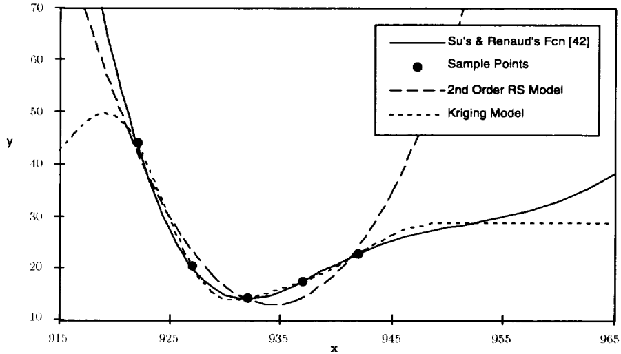
FIG. 3. One variable example for response surface and kriging models.
