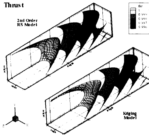
FIG. 9. Response surface and kriging models for thrust.
