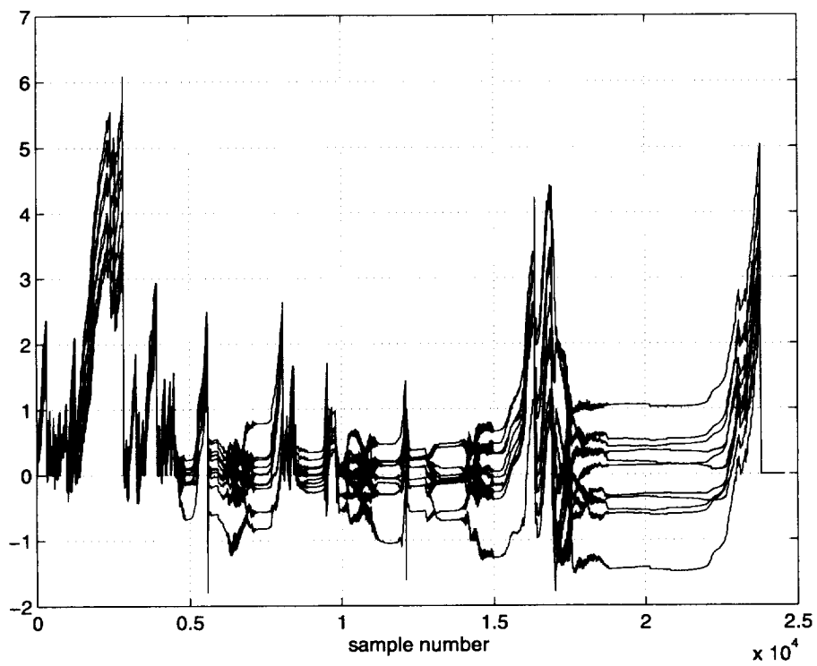
FIG. 2.4. The coefficients of the predictor from MNCMA
