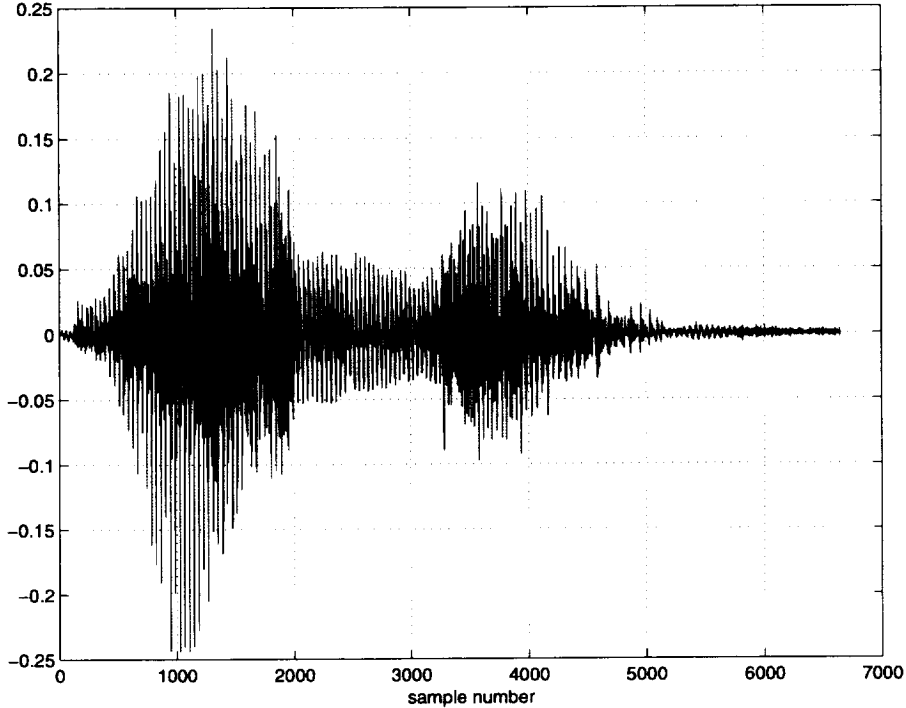
FIG. 3.5. Error signal (Constraint) from smoothing-only step
