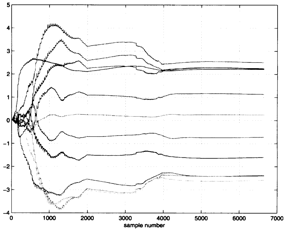
FIG. 3.7. Coefficients of the predictor from smoothing-only step
