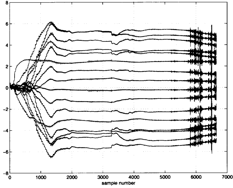
FIG. 3.12. Coefficients of the predictor from smoothing+non-iterative while L=16
