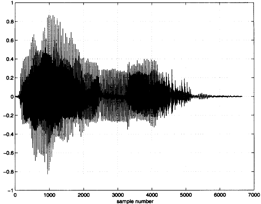
FIG. 3.13. Open-loop prediction by median coefficients from smoothing-only step while L=16
