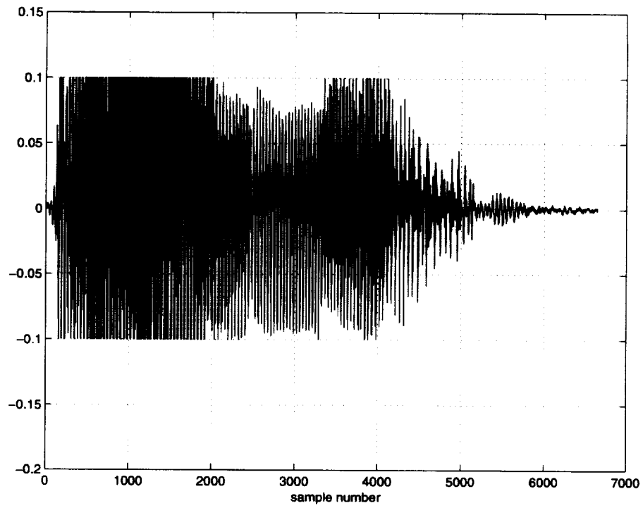
FIG. 3.15. Error signal (Constraint)
