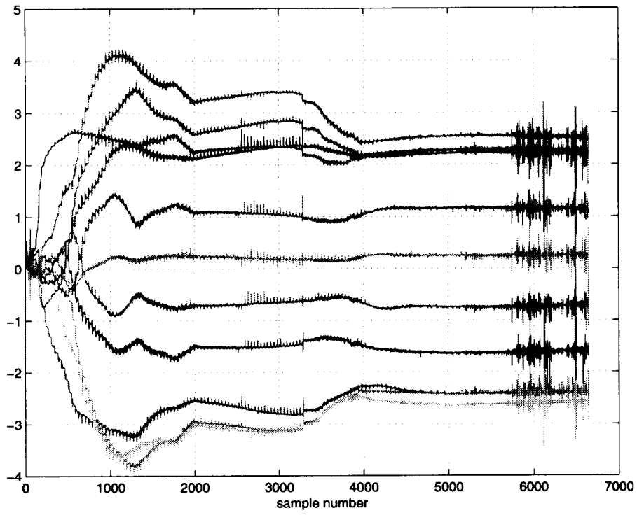
FIG. 3.8. Coefficients of the predictor from smoothing+non-iterative
