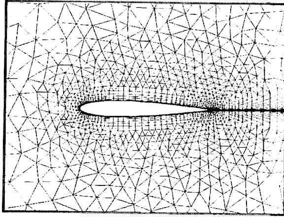
FIG. 2.1. Mixed element grid used for viscous flow calculations about NACA 0012 airfoil; Number of vertices = 4880
