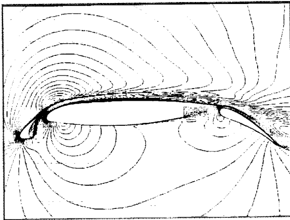
FIG. 7.6. Computed Mach Contours for Three-Element Airfoil Calculation. Mach = 0.2, Incidence = 16 degrees, Re number = 5 million
