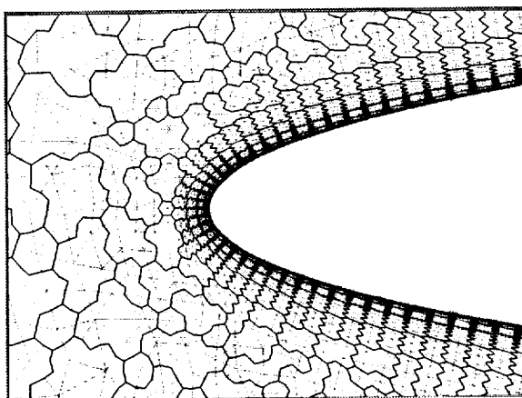
FIG. 9.1. Example of Agglomerated Grid Using 4:1 Coarsening along Lines in Boundary-Layer Region
