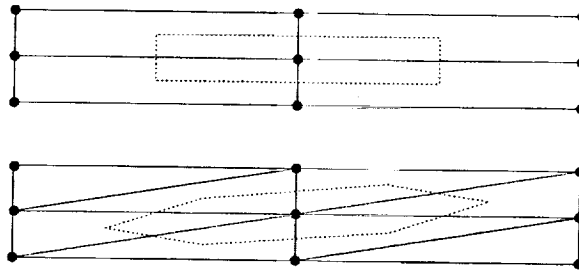
FIG. 2.2. Median control-volumes for stretched quadrilateral and triangular elements
