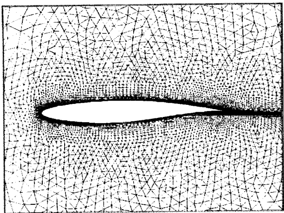
FIG. 6.1. Unstructured Grid Used for Computation of Transonic Flow Over RAE 2822 Airfoil. Number of Points = 16167, Wall Resolution = 10^{-6} chords
