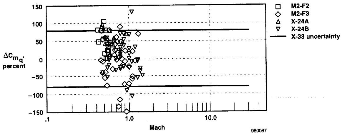
Figure 9. The X-33 pitch damping uncertainty.
