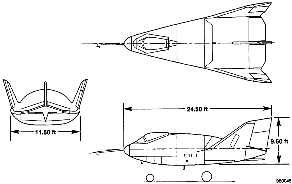
(e) The X-24A vehicle.
