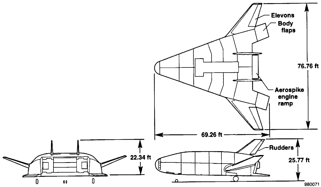
Figure 1. Three-view of the X-33 vehicle.
