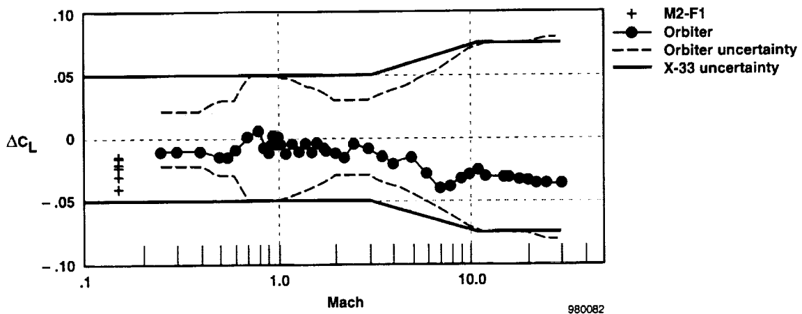
(b) Lift uncertainty.
