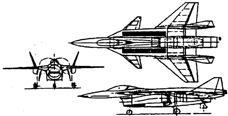
Figure 4. Ejector lift/vectored thrust concept combat aircraft, from ref. 3.
