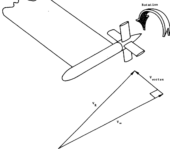
Figure 4. Vortex and stream flows and the resulting velocity, from ref. 6.
