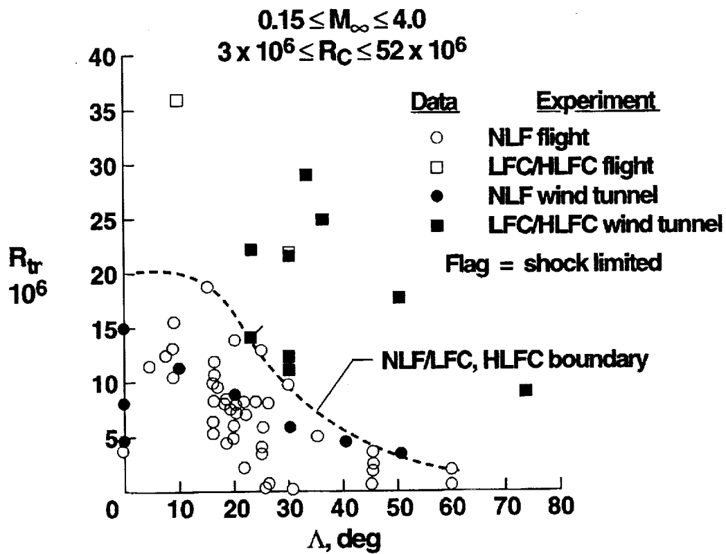
Figure 1. Effect of wing sweep on transition, from ref. 5.
