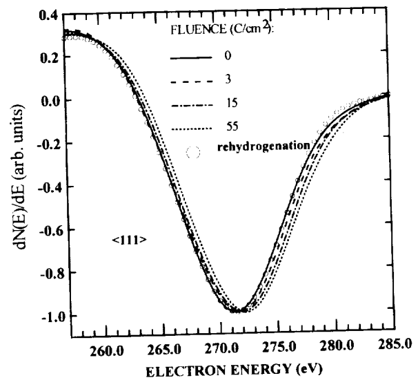
FIG. 1. Carbon A_0 Auger peak for the single-crystal diamond after various electron beam exposures (fluence range from 0 to 55\text{ C}/\text{cm}^2 ), and after subsequent rehydrogenation.
