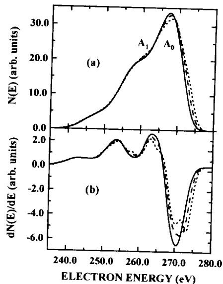
FIG. 7. Auger spectrum (a) and derivative of the Auger spectrum (b) of (111) diamond surface for various hydrogen coverages: 100%, solid line; 80%, dashed line; 60%, dotted line.
